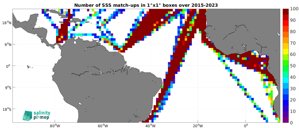
Figure 5: Number of SSS match-ups between TSG (LEGOS-DM) SSS and the SMAP SSS L3 v5.0 - Monthly (JPL) SSS product for the Tropical Atlantic Ocean Pi-MEP region over 1^\circ \times 1^\circ boxes and for the full satellite product period.
