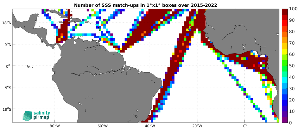
Figure 5: Number of SSS match-ups between TSG (LEGOS-DM) SSS and the SMAP SSS L3 v5.0 - Monthly (JPL) SSS product for the Tropical Atlantic Ocean Pi-MEP region over 1°×1° boxes and for the full satellite product period.
