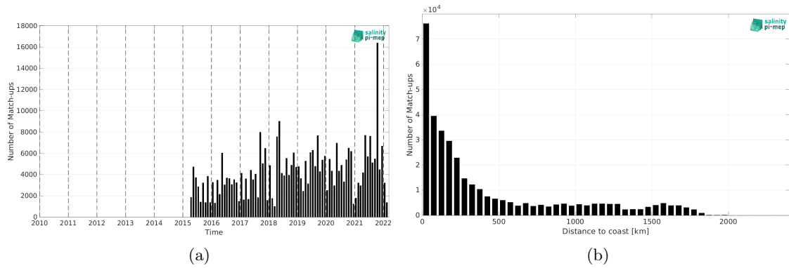
Figure 2: Number of match-ups between TSG (LEGOS-DM) and SMAP SSS L3 v5.0 - Monthly (JPL) SSS as a function of time (a) and as function of the distance to coast (b) over the Tropical Atlantic Ocean Pi-MEP region and for the full satellite product period.
