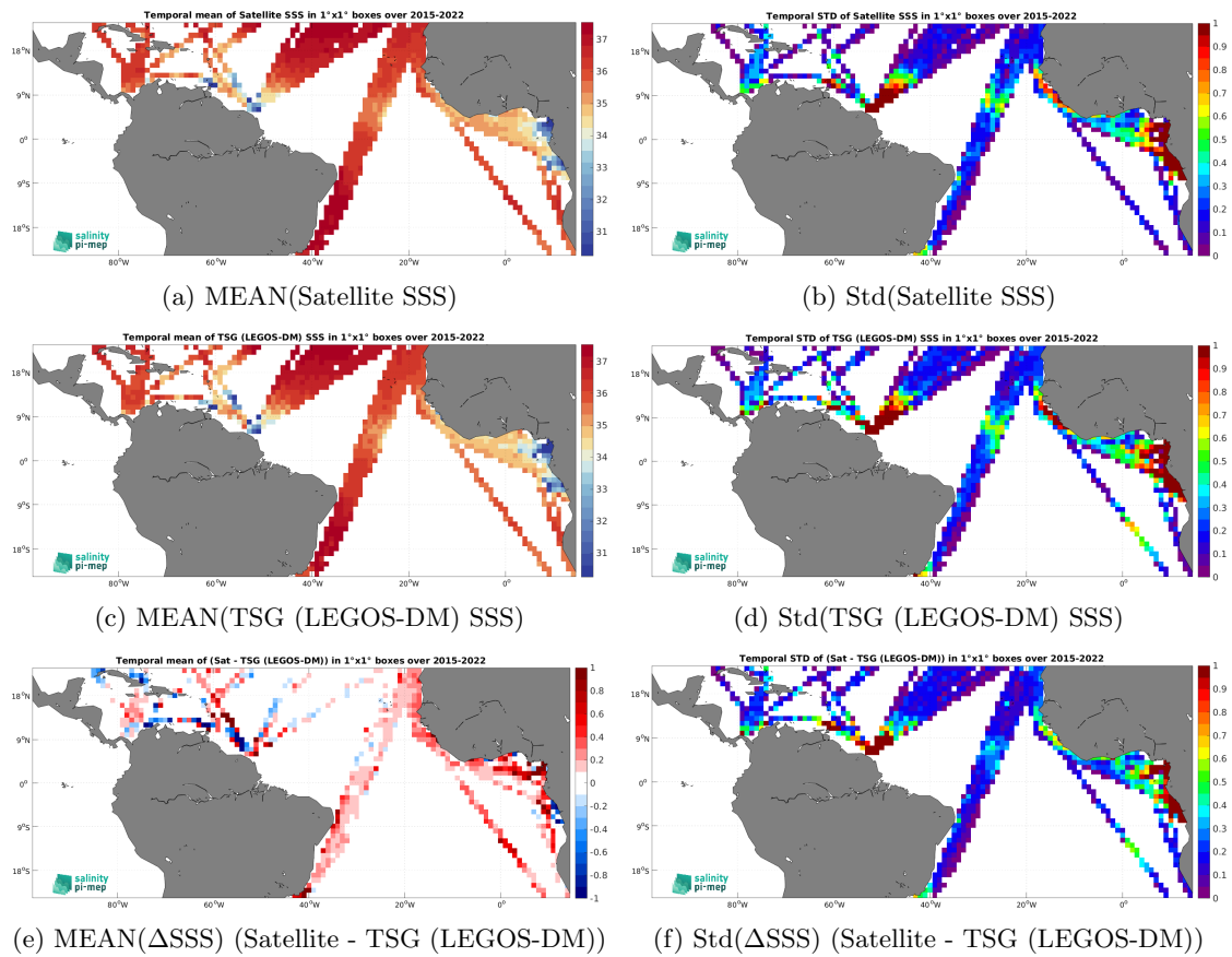
Figure 7: Temporal mean (left) and Std (right) of SSS from SMAP SSS L3 v5.0 - Monthly (JPL) (top), TSG (LEGOS-DM) (middle), and of \Delta SSS (Satellite - TSG (LEGOS-DM)). Only match-up pairs are used to generate these maps.
