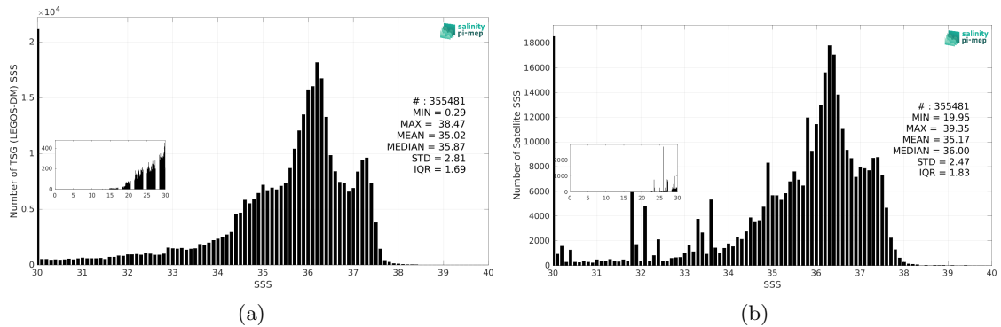
Figure 3: Histograms of SSS from TSG (LEGOS-DM) (a) and SMAP SSS L3 v5.0 - Monthly (JPL) (b) considering all match-up pairs per bins of 0.1 over the Tropical Atlantic Ocean Pi-MEP region and for the full satellite product period.
