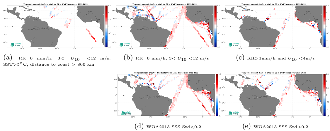
Figure 14: Temporal mean gridded over spatial boxes of size 1^\circ \times 1^\circ of \Delta SSS (SMAP SSS L3 v5.0 - Monthly (JPL) - TSG (LEGOS-DM)) for 5 different subdatasets corresponding to:RR=0 mm/h, 3 < U_{10} < 12 m/s, SST >5^\circ\text{C} , distance to coast > 800 km (a), RR=0 mm/h, 3 < U_{10} < 12 m/s (b), RR >1 mm/h and U_{10} < 4 m/s (c), WOA2013 SSS Std <0.2 (d), WOA2013 SSS Std >0.2 (e).
