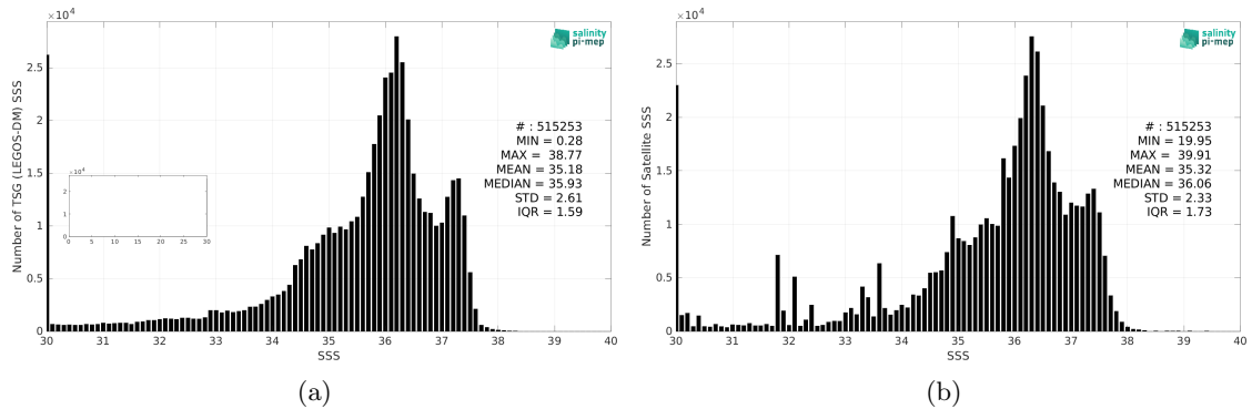
Figure 2: Histograms of SSS from TSG (LEGOS-DM) (a) and SMAP SSS L3 v5.0 - Monthly (JPL) (b) considering all match-up pairs per bins of 0.1 over the Tropical Atlantic Ocean Pi-MEP region and for the full satellite product period.
