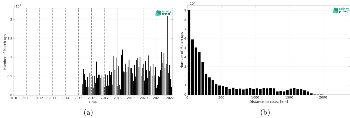
Figure 1: Number of match-ups between TSG (LEGOS-DM) and SMAP SSS L3 v5.0 - Monthly (JPL) SSS as a function of time (a) and as function of the distance to coast (b) over the Tropical Atlantic Ocean Pi-MEP region and for the full satellite product period.
