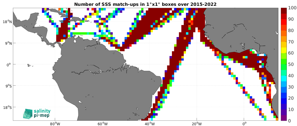
Figure 4: Number of SSS match-ups between TSG (LEGOS-DM) SSS and the SMAP SSS L3 v5.0 - Monthly (JPL) SSS product for the Tropical Atlantic Ocean Pi-MEP region over 1^\circ \times 1^\circ boxes and for the full satellite product period.
