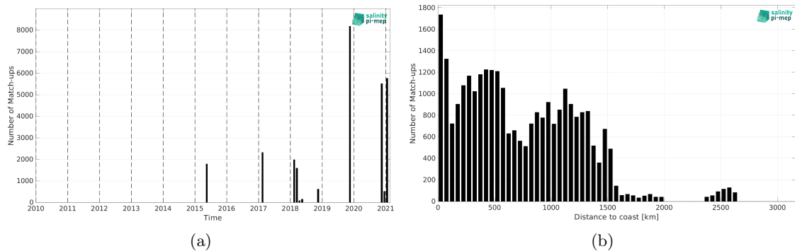
Figure 2: Number of match-ups between TSG (GOSUD-Sailing-ship) and SMAP SSS L3 v5.0 - Monthly (JPL) SSS as a function of time (a) and as function of the distance to coast (b) over the Tropical Atlantic Ocean Pi-MEP region and for the full satellite product period.
