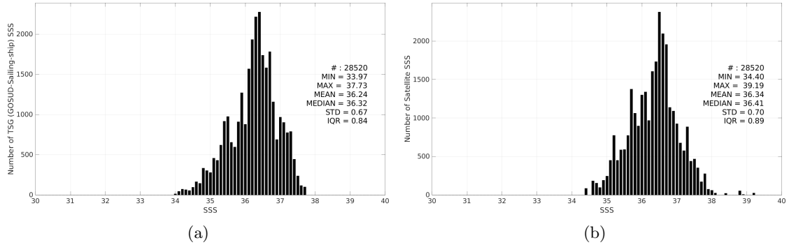
Figure 3: Histograms of SSS from TSG (GOSUD-Sailing-ship) (a) and SMAP SSS L3 v5.0 - Monthly (JPL) (b) considering all match-up pairs per bins of 0.1 over the Tropical Atlantic Ocean Pi-MEP region and for the full satellite product period.
