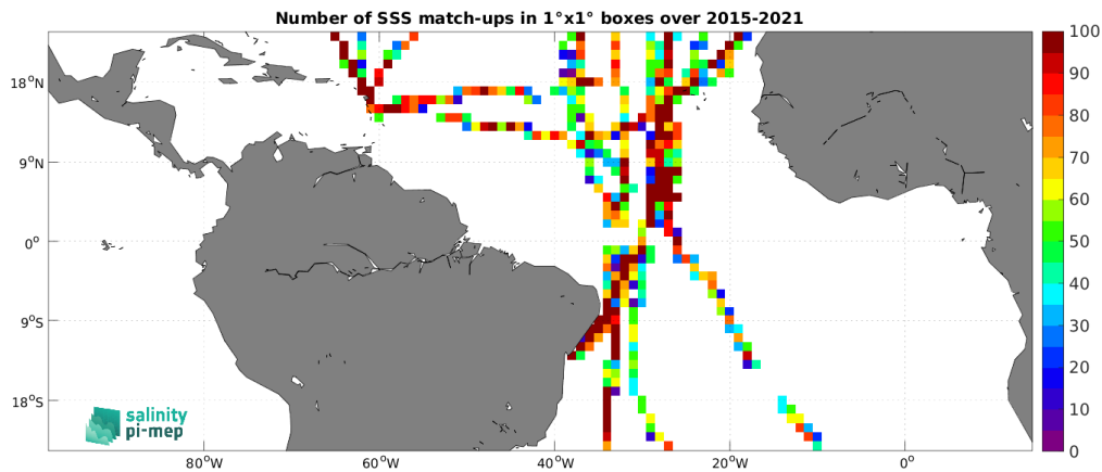
Figure 5: Number of SSS match-ups between TSG (GOSUD-Sailing-ship) SSS and the SMAP SSS L3 v5.0 - Monthly (JPL) SSS product for the Tropical Atlantic Ocean Pi-MEP region over 1^\circ \times 1^\circ boxes and for the full satellite product period.
