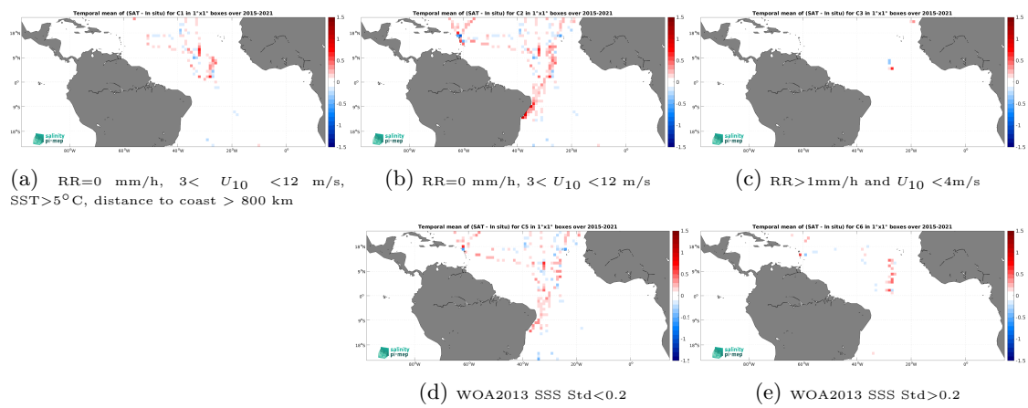
Figure 14: Temporal mean gridded over spatial boxes of size 1^\circ \times 1^\circ of \Delta\text{SSS} (SMAP SSS L3 v5.0 - Monthly (JPL) - TSG (GOSUD-Sailing-ship)) for 5 different subdatasets corresponding to:RR=0 mm/h, 3 < U_{10} < 12 m/s, SST>5°C, distance to coast > 800 km (a), RR=0 mm/h, 3 < U_{10} < 12 m/s (b), RR>1mm/h and U_{10} < 4 m/s (c), WOA2013 SSS Std<0.2 (d), WOA2013 SSS Std>0.2 (e).
