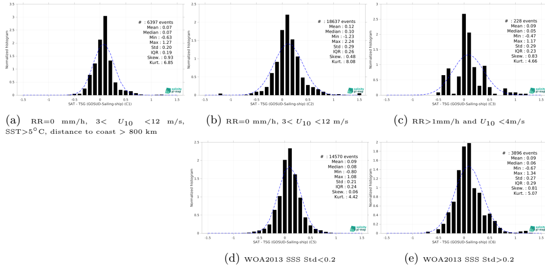
Figure 15: Normalized histogram of \Delta\text{SSS} (SMAP SSS L3 v5.0 - Monthly (JPL) - TSG (GOSUD-Sailing-ship)) for 5 different subdatasets corresponding to: RR=0 mm/h, 3 < U_{10} < 12 m/s, SST>5°C, distance to coast > 800 km (a), RR=0 mm/h, 3 < U_{10} < 12 m/s (b), RR>1mm/h and U_{10} < 4 m/s (c), WOA2013 SSS Std<0.2 (d), WOA2013 SSS Std>0.2 (e).
