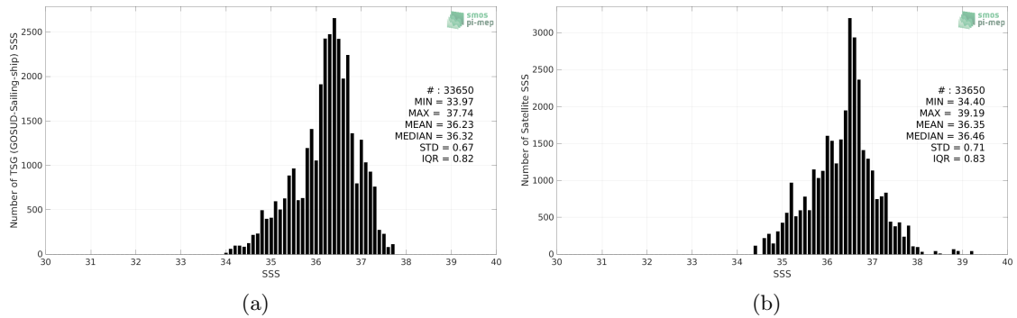
Figure 2: Histograms of SSS from TSG (GOSUD-Sailing-ship) (a) and SMAP SSS L3 v5.0 - Monthly (JPL) (b) considering all match-up pairs per bins of 0.1 over the Tropical Atlantic Ocean Pi-MEP region and for the full satellite product period.
