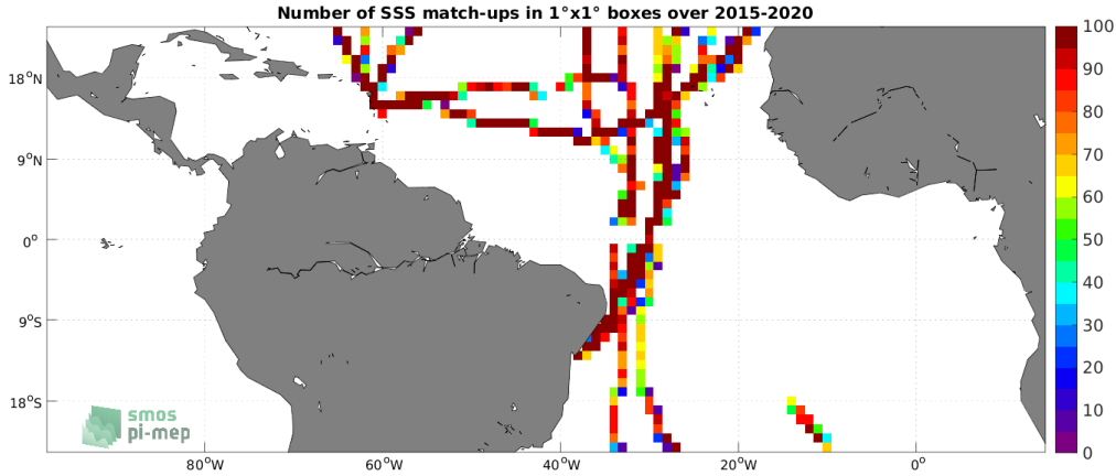
Figure 4: Number of SSS match-ups between TSG (GOSUD-Sailing-ship) SSS and the SMAP SSS L3 v5.0 - Monthly (JPL) SSS product for the Tropical Atlantic Ocean Pi-MEP region over 1^\circ \times 1^\circ boxes and for the full satellite product period.
