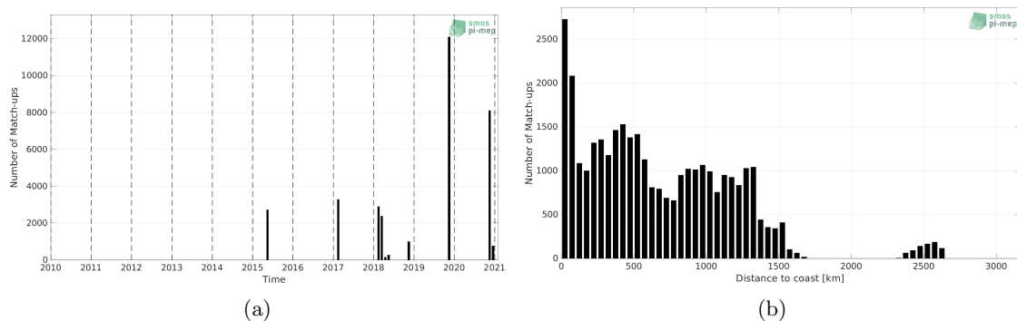
Figure 1: Number of match-ups between TSG (GOSUD-Sailing-ship) and SMAP SSS L3 v5.0 - Monthly (JPL) SSS as a function of time (a) and as function of the distance to coast (b) over the Tropical Atlantic Ocean Pi-MEP region and for the full satellite product period.
