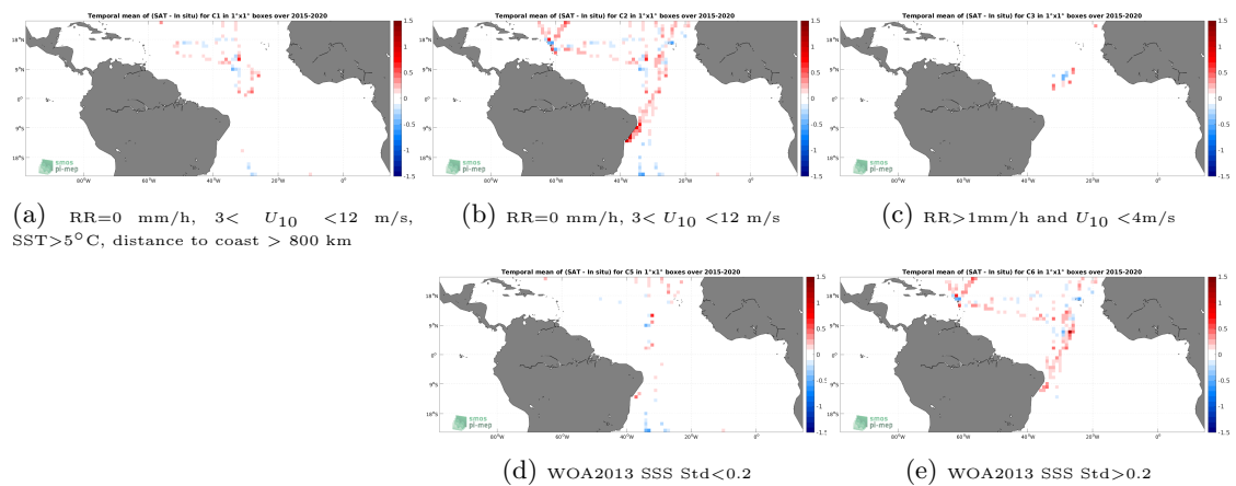
Figure 12: Temporal mean gridded over spatial boxes of size 1^\circ \times 1^\circ of \Delta SSS (SMAP SSS L3 v5.0 - Monthly (JPL) - TSG (GOSUD-Sailing-ship)) for 5 different subdatasets corresponding to:RR=0 mm/h, 3 < U_{10} < 12 m/s, SST >5^\circ\text{C} , distance to coast > 800 km (a), RR=0 mm/h, 3 < U_{10} < 12 m/s (b), RR >1 mm/h and U_{10} < 4 m/s (c), WOA2013 SSS Std <0.2 (d), WOA2013 SSS Std >0.2 (e).
