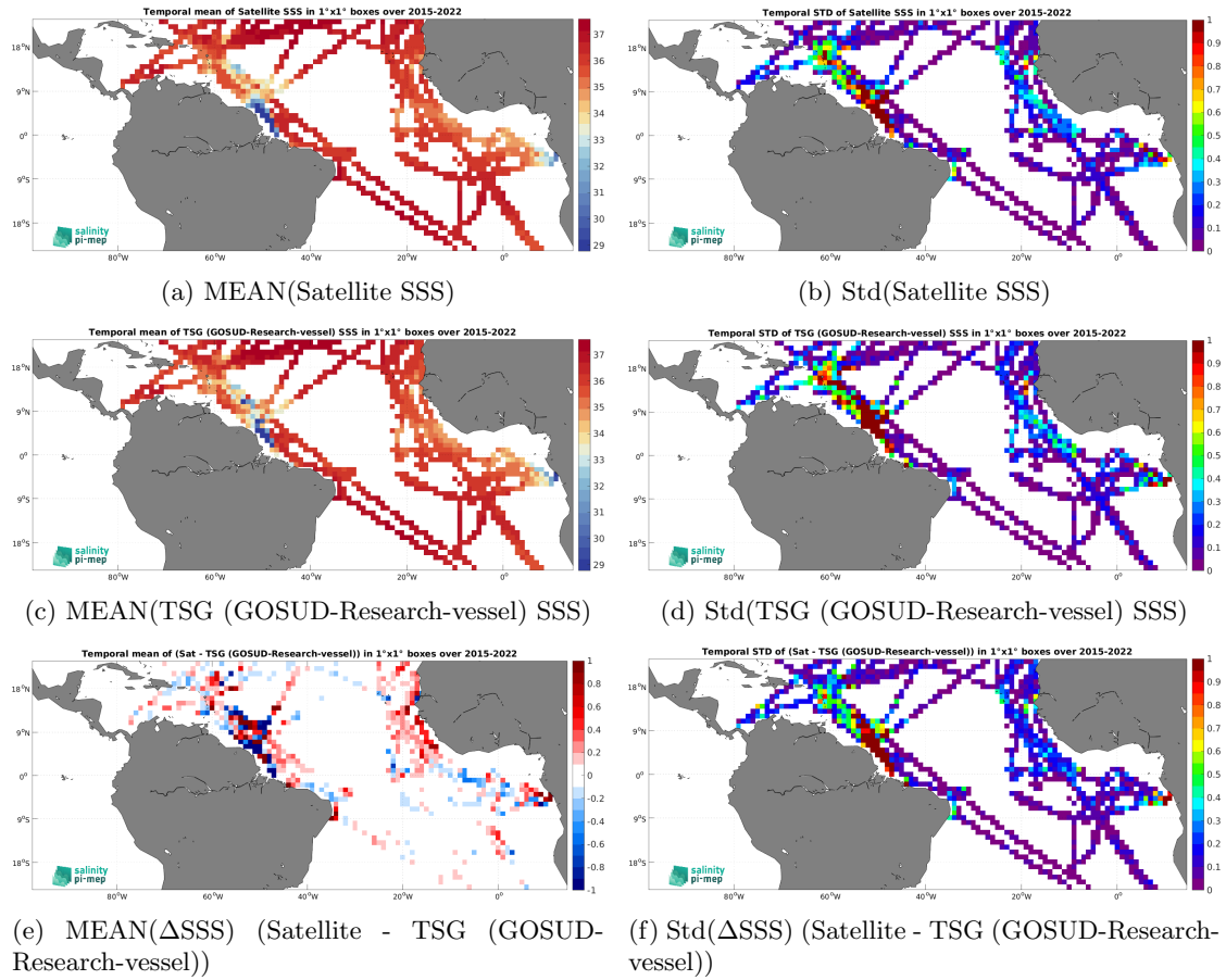
Figure 7: Temporal mean (left) and Std (right) of SSS from SMAP SSS L3 v5.0 - Monthly (JPL) (top), TSG (GOSUD-Research-vessel) (middle), and of \Delta SSS (Satellite - TSG (GOSUD-Research-vessel)). Only match-up pairs are used to generate these maps.
