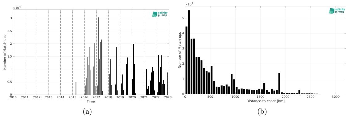
Figure 2: Number of match-ups between TSG (GOSUD-Research-vessel) and SMAP SSS L3 v5.0 - Monthly (JPL) SSS as a function of time (a) and as function of the distance to coast (b) over the Tropical Atlantic Ocean Pi-MEP region and for the full satellite product period.
