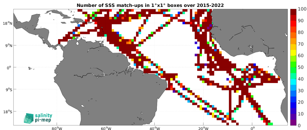
Figure 5: Number of SSS match-ups between TSG (GOSUD-Research-vessel) SSS and the SMAP SSS L3 v5.0 - Monthly (JPL) SSS product for the Tropical Atlantic Ocean Pi-MEP region over 1^\circ \times 1^\circ boxes and for the full satellite product period.
