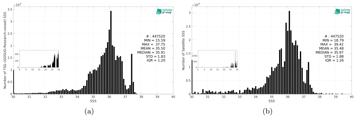
Figure 3: Histograms of SSS from TSG (GOSUD-Research-vessel) (a) and SMAP SSS L3 v5.0 - Monthly (JPL) (b) considering all match-up pairs per bins of 0.1 over the Tropical Atlantic Ocean Pi-MEP region and for the full satellite product period.
