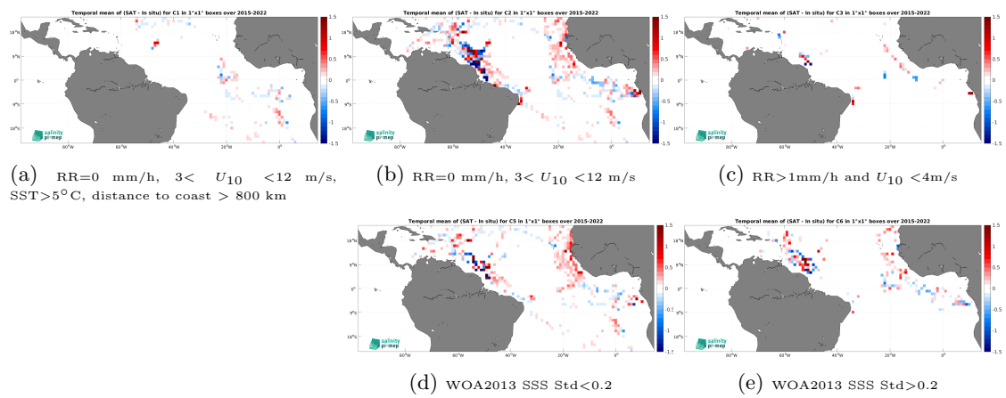
Figure 14: Temporal mean gridded over spatial boxes of size 1^\circ \times 1^\circ of \Delta\text{SSS} (SMAP SSS L3 v5.0 - Monthly (JPL) - TSG (GOSUD-Research-vessel)) for 5 different subdatasets corresponding to:RR=0 mm/h, 3 < U_{10} < 12 m/s, SST >5^\circ\text{C} , distance to coast > 800 km (a), RR=0 mm/h, 3 < U_{10} < 12 m/s (b), RR >1 mm/h and U_{10} < 4 m/s (c), WOA2013 SSS Std <0.2 (d), WOA2013 SSS Std >0.2 (e).
