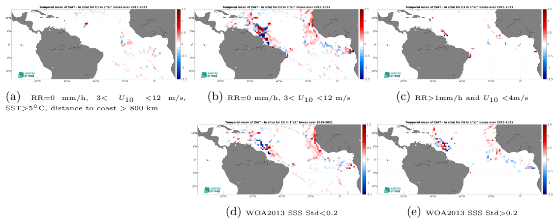
Figure 14: Temporal mean gridded over spatial boxes of size 1^\circ \times 1^\circ of \Delta\text{SSS} (SMAP SSS L3 v5.0 - Monthly (JPL) - TSG (GOSUD-Research-vessel)) for 5 different subdatasets corresponding to:RR=0 mm/h, 3 < U_{10} < 12 m/s, SST >5^\circ\text{C} , distance to coast > 800 km (a), RR=0 mm/h, 3 < U_{10} < 12 m/s (b), RR >1 mm/h and U_{10} < 4 m/s (c), WOA2013 SSS Std <0.2 (d), WOA2013 SSS Std >0.2 (e).
