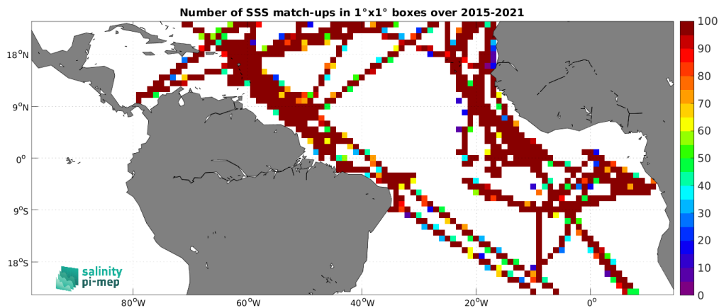
Figure 5: Number of SSS match-ups between TSG (GOSUD-Research-vessel) SSS and the SMAP SSS L3 v5.0 - Monthly (JPL) SSS product for the Tropical Atlantic Ocean Pi-MEP region over 1°x1° boxes and for the full satellite product period.
