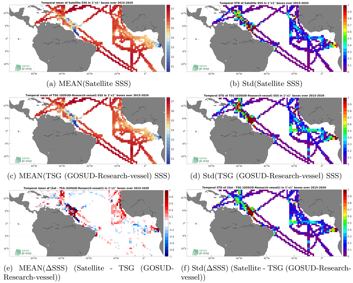
Figure 6: Temporal mean (left) and Std (right) of SSS from SMAP SSS L3 v5.0 - Monthly (JPL) (top), TSG (GOSUD-Research-vessel) (middle), and of \Delta SSS (Satellite - TSG (GOSUD-Research-vessel)). Only match-up pairs are used to generate these maps.
