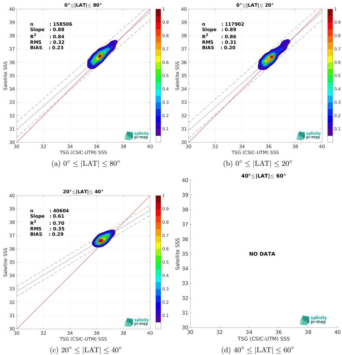
Figure 10: Contour maps of the concentration of SMAP SSS L3 v5.0 - Monthly (JPL) SSS (y-axis) versus TSG (CSIC-UTM) SSS (x-axis) at match-up pairs for different latitude bands. For each plot, the red line shows x=y . The black thin and dashed lines indicate a linear fit through the data cloud and the \pm 95\% confidence levels, respectively. The number match-up pairs n , the slope and R^2 coefficient of the linear fit, the root mean square (RMS) and the mean bias between satellite and in situ data are indicated for each latitude band in each plots.
