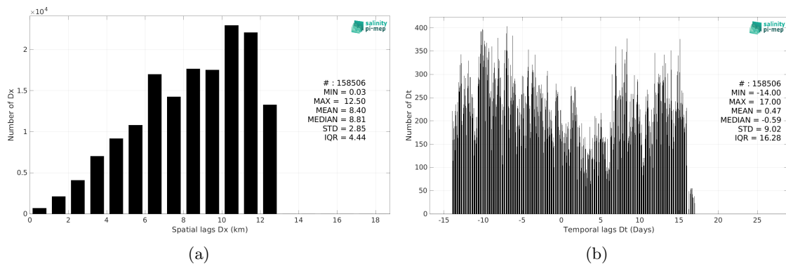
Figure 6: Histograms of the spatial (a) and temporal (b) lags between the location/time of the TSG (CSIC-UTM) measurement and the date of the corresponding SMAP SSS L3 v5.0 - Monthly (JPL) SSS pixel.
