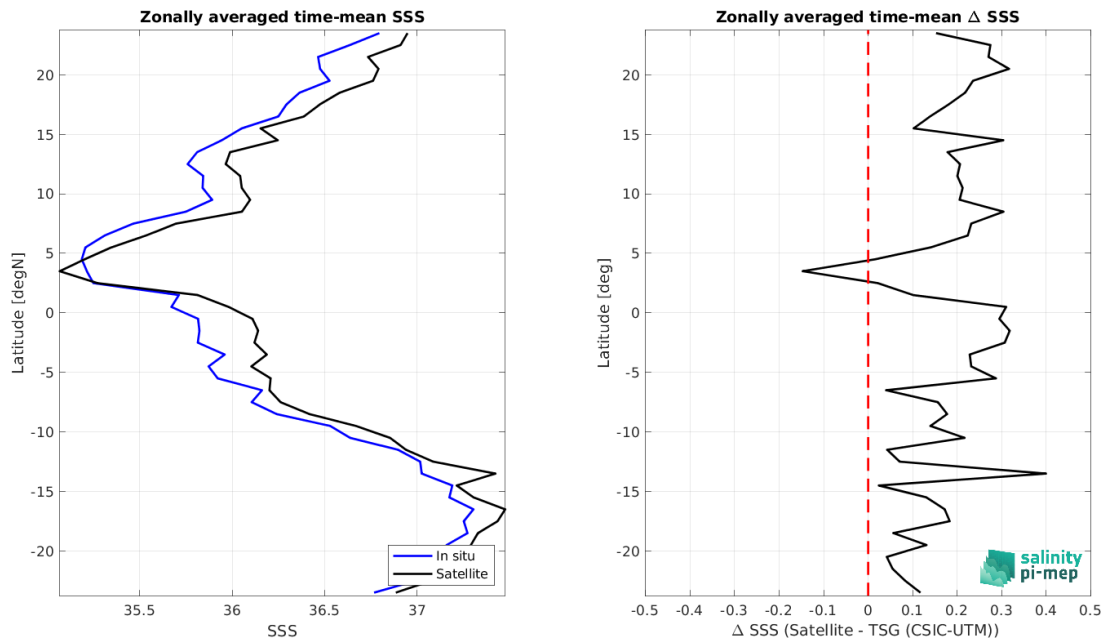
Figure 9: Left panel: Zonal mean SSS from SMAP SSS L3 v5.0 - Monthly (JPL) satellite product (black) and from TSG (CSIC-UTM) (blue). Right panel: Zonal mean of \Delta SSS (Satellite - TSG (CSIC-UTM)) for all the collected Pi-MEP match-up pairs estimated over the full satellite product period.
