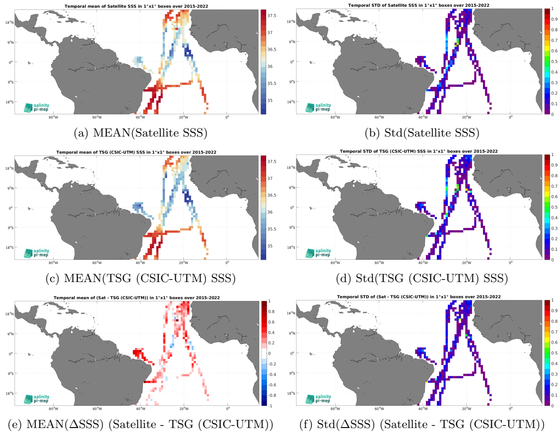
Figure 7: Temporal mean (left) and Std (right) of SSS from SMAP SSS L3 v5.0 - Monthly (JPL) (top), TSG (CSIC-UTM) (middle), and of \Delta SSS (Satellite - TSG (CSIC-UTM)). Only match-up pairs are used to generate these maps.
