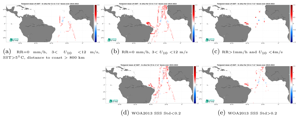
Figure 14: Temporal mean gridded over spatial boxes of size 1^\circ \times 1^\circ of \Delta\text{SSS} (SMAP SSS L3 v5.0 - Monthly (JPL) - TSG (CSIC-UTM)) for 5 different subdatasets corresponding to:RR=0 mm/h, 3 < U_{10} < 12 m/s, SST >5^\circ\text{C} , distance to coast > 800 km (a), RR=0 mm/h, 3 < U_{10} < 12 m/s (b), RR >1 mm/h and U_{10} < 4 m/s (c), WOA2013 SSS Std <0.2 (d), WOA2013 SSS Std >0.2 (e).
