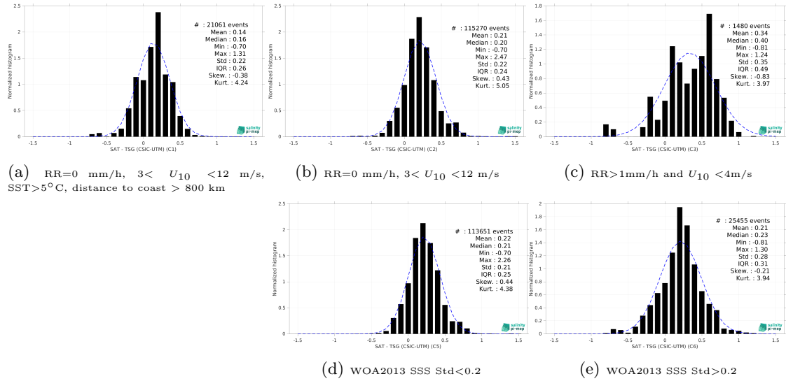
Figure 15: Normalized histogram of \Delta SSS (SMAP SSS L3 v5.0 - Monthly (JPL) - TSG (CSIC-UTM)) for 5 different subdatasets corresponding to: RR=0 mm/h, 3 < U_{10} < 12 m/s, SST>5°C, distance to coast > 800 km (a), RR=0 mm/h, 3 < U_{10} < 12 m/s (b), RR>1mm/h and U_{10} < 4 m/s (c), WOA2013 SSS Std<0.2 (d), WOA2013 SSS Std>0.2 (e).
