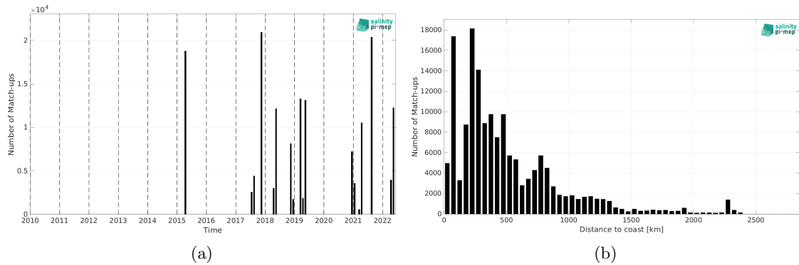
Figure 2: Number of match-ups between TSG (CSIC-UTM) and SMAP SSS L3 v5.0 - Monthly (JPL) SSS as a function of time (a) and as function of the distance to coast (b) over the Tropical Atlantic Ocean Pi-MEP region and for the full satellite product period.
