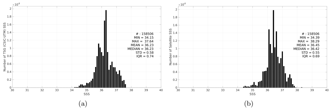
Figure 3: Histograms of SSS from TSG (CSIC-UTM) (a) and SMAP SSS L3 v5.0 - Monthly (JPL) (b) considering all match-up pairs per bins of 0.1 over the Tropical Atlantic Ocean Pi-MEP region and for the full satellite product period.
