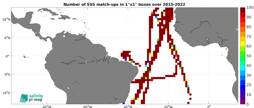
Figure 5: Number of SSS match-ups between TSG (CSIC-UTM) SSS and the SMAP SSS L3 v5.0 - Monthly (JPL) SSS product for the Tropical Atlantic Ocean Pi-MEP region over 1^\circ \times 1^\circ boxes and for the full satellite product period.
