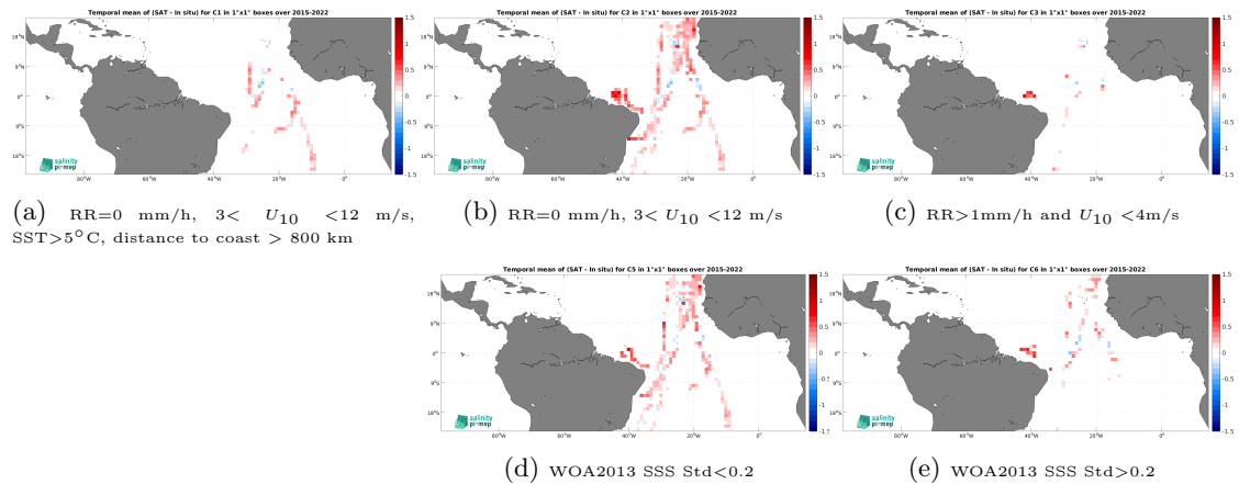
Figure 12: Temporal mean gridded over spatial boxes of size 1^\circ \times 1^\circ of \Delta\text{SSS} (SMAP SSS L3 v5.0 - Monthly (JPL) - TSG (CSIC-UTM)) for 5 different subdatasets corresponding to:RR=0 mm/h, 3 < U_{10} < 12 m/s, SST > 5^\circ\text{C} , distance to coast > 800 km (a), RR=0 mm/h, 3 < U_{10} < 12 m/s (b), RR > 1 mm/h and U_{10} < 4 m/s (c), WOA2013 SSS Std < 0.2 (d), WOA2013 SSS Std > 0.2 (e).
