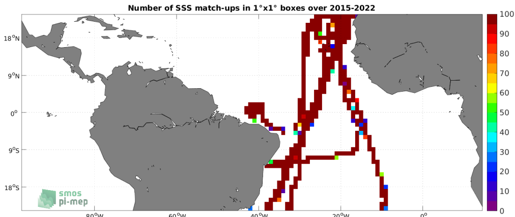
Figure 4: Number of SSS match-ups between TSG (CSIC-UTM) SSS and the SMAP SSS L3 v5.0 - Monthly (JPL) SSS product for the Tropical Atlantic Ocean Pi-MEP region over 1^\circ \times 1^\circ boxes and for the full satellite product period.
