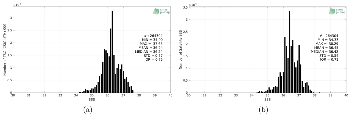
Figure 2: Histograms of SSS from TSG (CSIC-UTM) (a) and SMAP SSS L3 v5.0 - Monthly (JPL) (b) considering all match-up pairs per bins of 0.1 over the Tropical Atlantic Ocean Pi-MEP region and for the full satellite product period.
