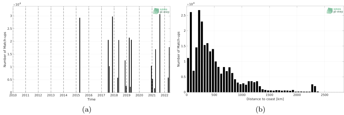
Figure 1: Number of match-ups between TSG (CSIC-UTM) and SMAP SSS L3 v5.0 - Monthly (JPL) SSS as a function of time (a) and as function of the distance to coast (b) over the Tropical Atlantic Ocean Pi-MEP region and for the full satellite product period.
