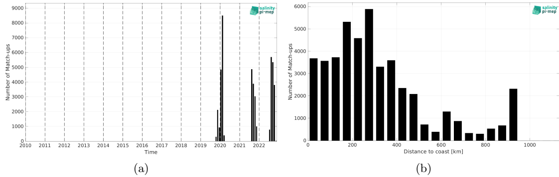
Figure 2: Number of match-ups between Saildrone and SMAP SSS L3 v5.0 - Monthly (JPL) SSS as a function of time (a) and as function of the distance to coast (b) over the Tropical Atlantic Ocean Pi-MEP region and for the full satellite product period.
