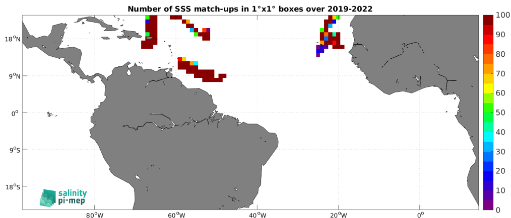
Figure 5: Number of SSS match-ups between Saildrone SSS and the SMAP SSS L3 v5.0 - Monthly (JPL) SSS product for the Tropical Atlantic Ocean Pi-MEP region over 1^\circ \times 1^\circ boxes and for the full satellite product period.
