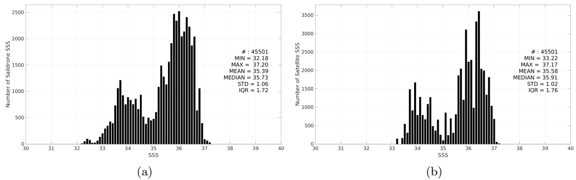
Figure 3: Histograms of SSS from Saildrone (a) and SMAP SSS L3 v5.0 - Monthly (JPL) (b) considering all match-up pairs per bins of 0.1 over the Tropical Atlantic Ocean Pi-MEP region and for the full satellite product period.
