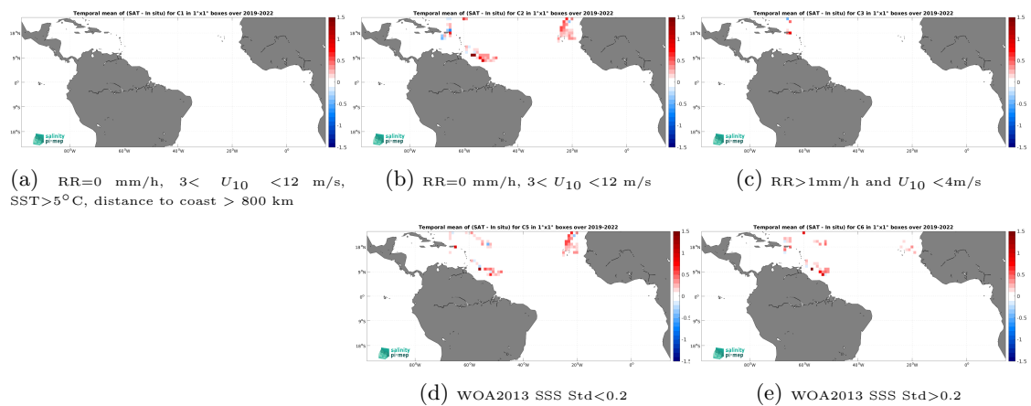
Figure 14: Temporal mean gridded over spatial boxes of size 1^\circ \times 1^\circ of \Delta SSS (SMAP SSS L3 v5.0 - Monthly (JPL) - Sairdrone) for 5 different subdatasets corresponding to:RR=0 mm/h, 3 < U_{10} < 12 m/s, SST >5^\circ\text{C} , distance to coast > 800 km (a), RR=0 mm/h, 3 < U_{10} < 12 m/s (b), RR >1 mm/h and U_{10} < 4 m/s (c), WOA2013 SSS Std <0.2 (d), WOA2013 SSS Std >0.2 (e).
