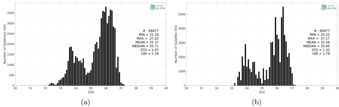
Figure 2: Histograms of SSS from Saildrone (a) and SMAP SSS L3 v5.0 - Monthly (JPL) (b) considering all match-up pairs per bins of 0.1 over the Tropical Atlantic Ocean Pi-MEP region and for the full satellite product period.
