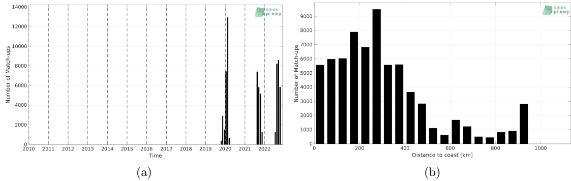
Figure 1: Number of match-ups between Saildrone and SMAP SSS L3 v5.0 - Monthly (JPL) SSS as a function of time (a) and as function of the distance to coast (b) over the Tropical Atlantic Ocean Pi-MEP region and for the full satellite product period.
