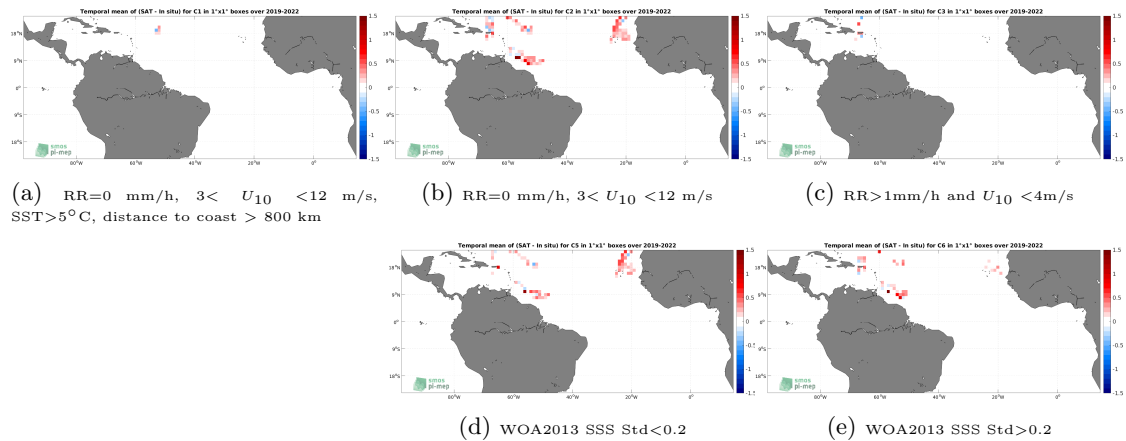
Figure 12: Temporal mean gridded over spatial boxes of size 1^\circ \times 1^\circ of \Delta SSS (SMAP SSS L3 v5.0 - Monthly (JPL) - Sairdrone) for 5 different subdatasets corresponding to:RR=0 mm/h, 3 < U_{10} < 12 m/s, SST >5^\circ\text{C} , distance to coast > 800 km (a), RR=0 mm/h, 3 < U_{10} < 12 m/s (b), RR >1 mm/h and U_{10} < 4 m/s (c), WOA2013 SSS Std <0.2 (d), WOA2013 SSS Std >0.2 (e).
