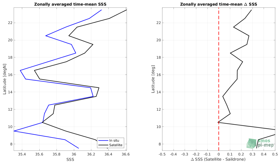
Figure 8: Left panel: Zonal mean SSS from SMAP SSS L3 v5.0 - Monthly (JPL) satellite product (black) and from Sairdrone (blue). Right panel: Zonal mean of \Delta SSS (Satellite - Sairdrone) for all the collected Pi-MEP match-up pairs estimated over the full satellite product period.
