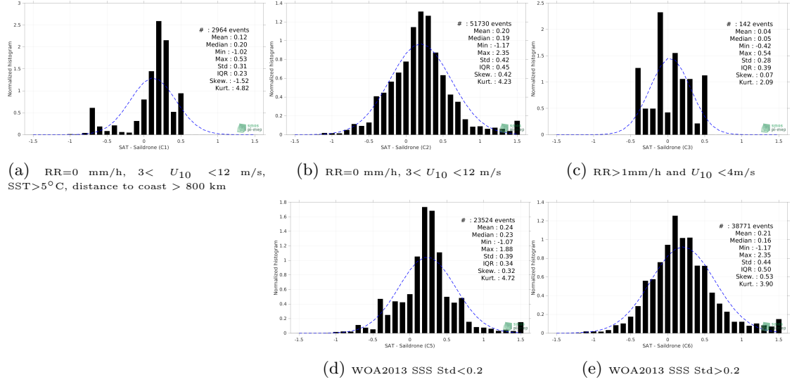
Figure 13: Normalized histogram of \Delta SSS (SMAP SSS L3 v5.0 - Monthly (JPL) - Sairdrone) for 5 different subdatasets corresponding to: RR=0 mm/h, 3 < U_{10} < 12 m/s, SST > 5°C, distance to coast > 800 km (a), RR=0 mm/h, 3 < U_{10} < 12 m/s (b), RR > 1mm/h and U_{10} < 4 m/s (c), WOA2013 SSS Std < 0.2 (d), WOA2013 SSS Std > 0.2 (e).
