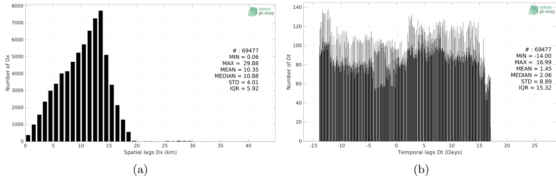
Figure 5: Histograms of the spatial (a) and temporal (b) lags between the location/time of the Saildrone measurement and the date of the corresponding SMAP SSS L3 v5.0 - Monthly (JPL) SSS pixel.
