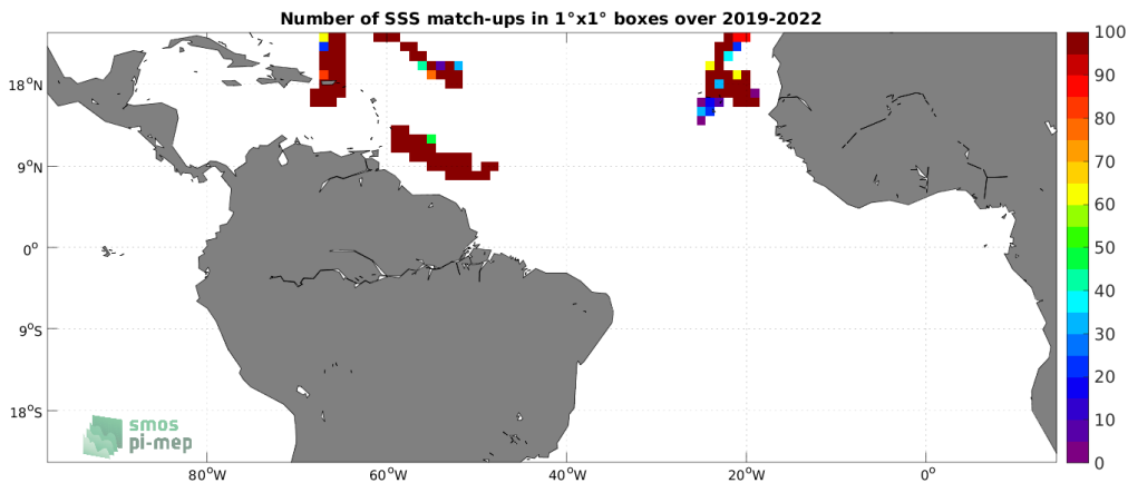
Figure 4: Number of SSS match-ups between Saildrone SSS and the SMAP SSS L3 v5.0 - Monthly (JPL) SSS product for the Tropical Atlantic Ocean Pi-MEP region over 1^\circ \times 1^\circ boxes and for the full satellite product period.
