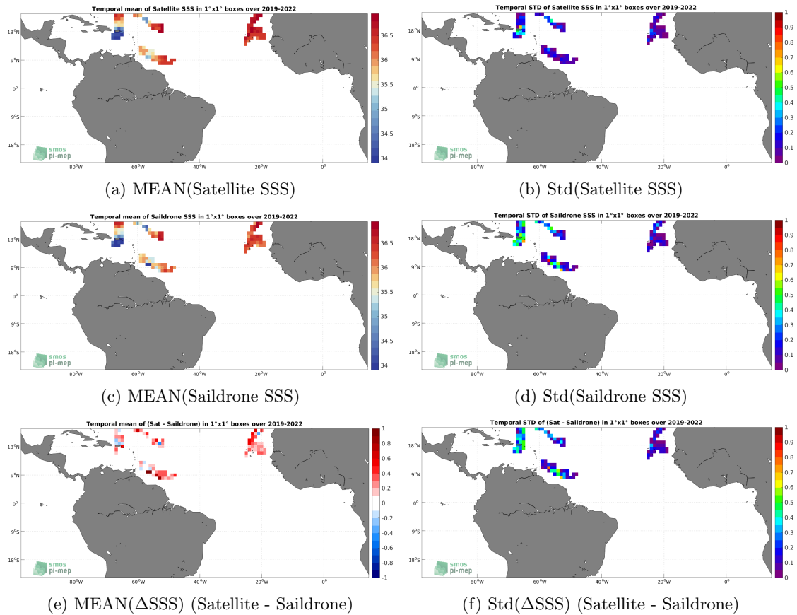
Figure 6: Temporal mean (left) and Std (right) of SSS from SMAP SSS L3 v5.0 - Monthly (JPL) (top), Saildrone (middle), and of \Delta SSS (Satellite - Saildrone). Only match-up pairs are used to generate these maps.
