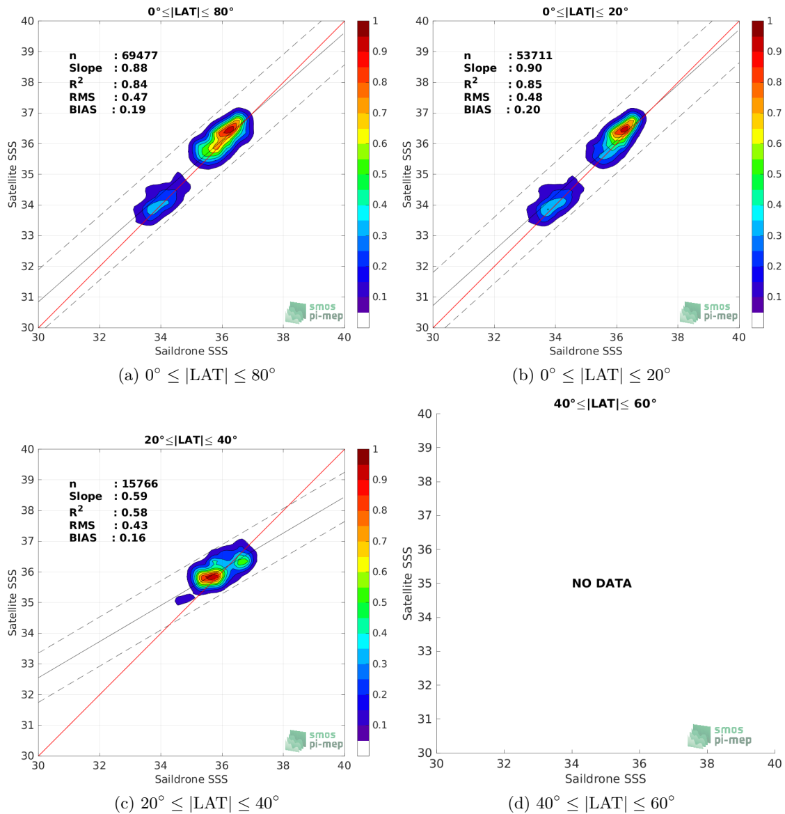
Figure 9: Contour maps of the concentration of SMAP SSS L3 v5.0 - Monthly (JPL) SSS (y-axis) versus SAILDRONE SSS (x-axis) at match-up pairs for different latitude bands. For each plot, the red line shows x=y . The black thin and dashed lines indicate a linear fit through the data cloud and the \pm 95\% confidence levels, respectively. The number match-up pairs n , the slope and R^2 coefficient of the linear fit, the root mean square (RMS) and the mean bias between satellite and in situ data are indicated for each latitude band in each plots.
