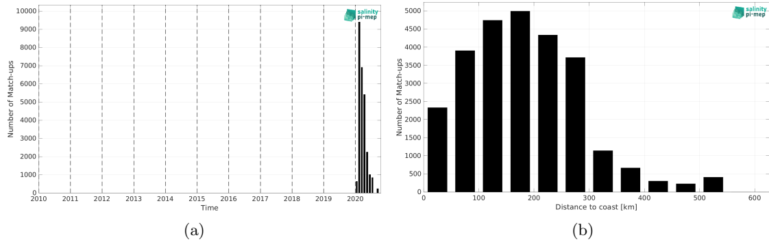
Figure 2: Number of match-ups between Surface drifters and SMAP SSS L3 v5.0 - Monthly (JPL) SSS as a function of time (a) and as function of the distance to coast (b) over the Tropical Atlantic Ocean Pi-MEP region and for the full satellite product period.
