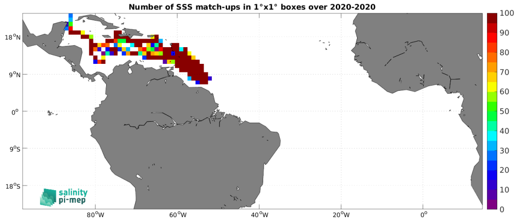
Figure 4: Number of SSS match-ups between Surface drifters SSS and the SMAP SSS L3 v5.0 - Monthly (JPL) SSS product for the Tropical Atlantic Ocean Pi-MEP region over 1^\circ \times 1^\circ boxes and for the full satellite product period.
