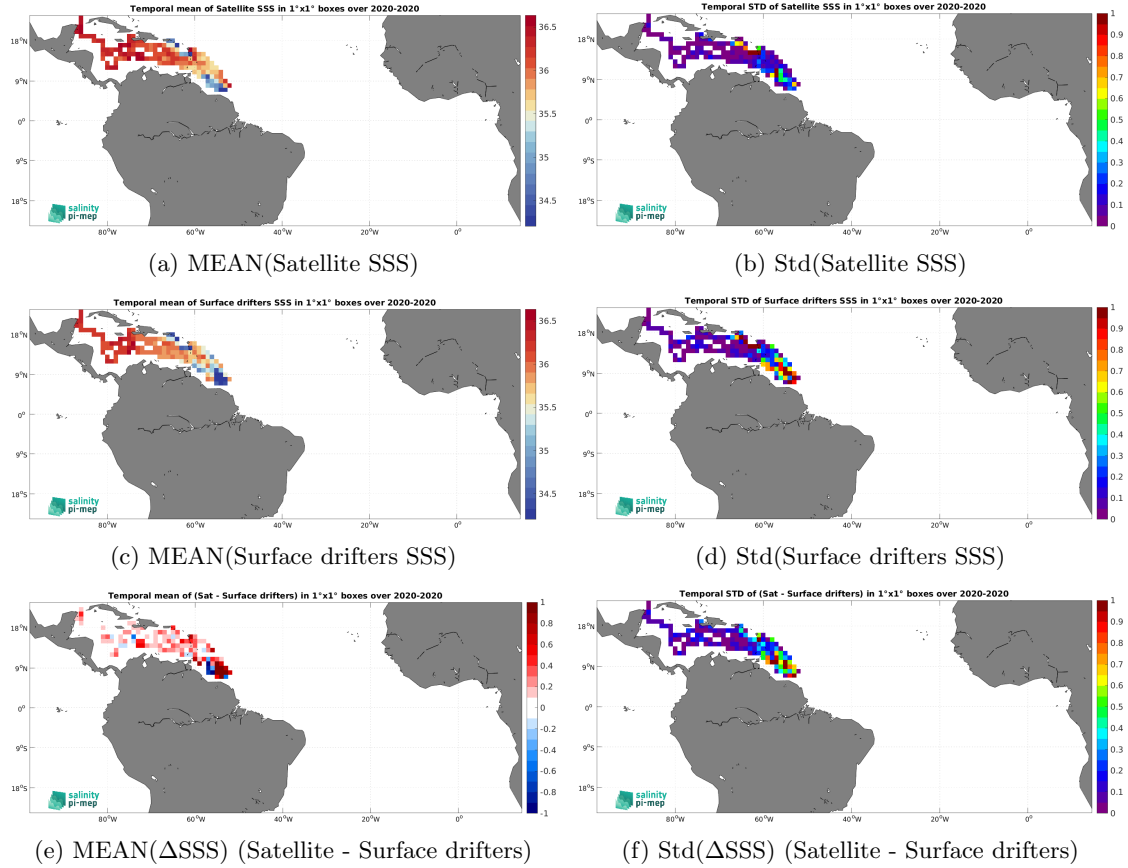
Figure 6: Temporal mean (left) and Std (right) of SSS from SMAP SSS L3 v5.0 - Monthly (JPL) (top), Surface drifters (middle), and of \Delta\text{SSS} (Satellite - Surface drifters). Only match-up pairs are used to generate these maps.
