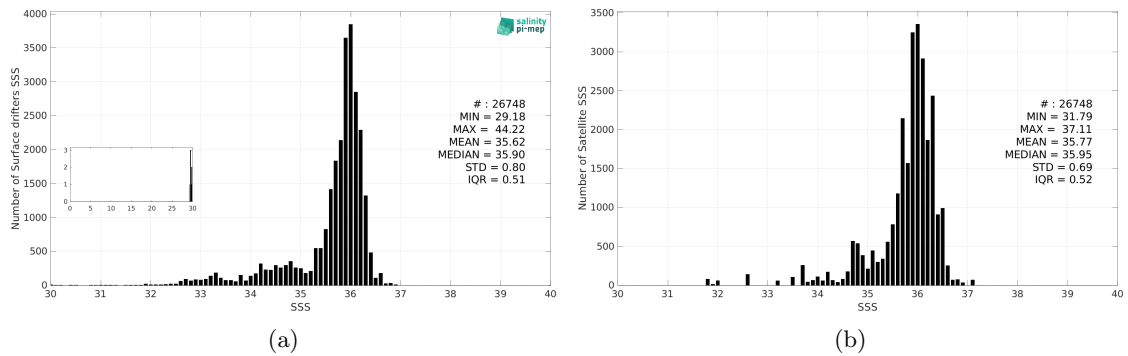
Figure 3: Histograms of SSS from Surface drifters (a) and SMAP SSS L3 v5.0 - Monthly (JPL) (b) considering all match-up pairs per bins of 0.1 over the Tropical Atlantic Ocean Pi-MEP region and for the full satellite product period.
