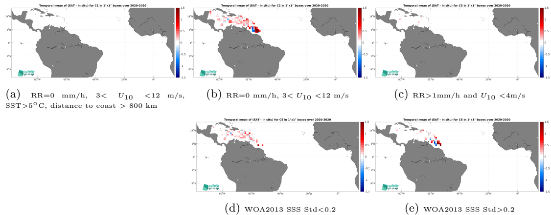
Figure 13: Temporal mean gridded over spatial boxes of size 1^\circ \times 1^\circ of \Delta\text{SSS} (SMAP SSS L3 v5.0 - Monthly (JPL) - Surface drifters) for 5 different subdatasets corresponding to:RR=0 mm/h, 3 < U_{10} < 12 m/s, SST >5^\circ\text{C} , distance to coast > 800 km (a), RR=0 mm/h, 3 < U_{10} < 12 m/s (b), RR >1 mm/h and U_{10} < 4 m/s (c), WOA2013 SSS Std <0.2 (d), WOA2013 SSS Std >0.2 (e).
