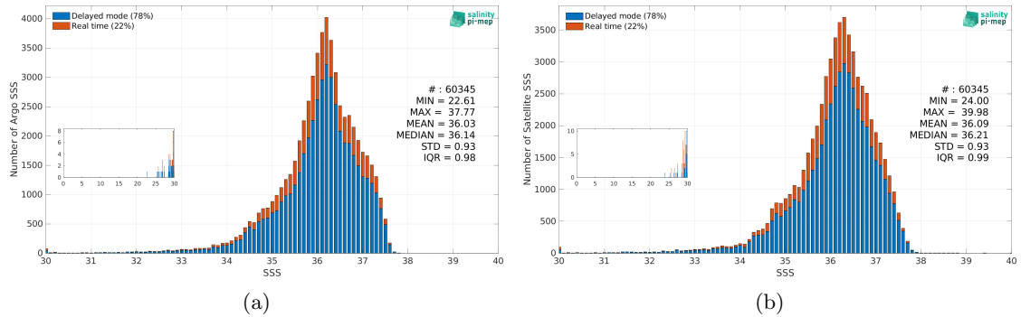
Figure 3: Histograms of SSS from Argo (a) and SMAP SSS L3 v5.0 - Monthly (JPL) (b) considering all match-up pairs per bins of 0.1 over the Tropical Atlantic Ocean Pi-MEP region and for the full satellite product period.
