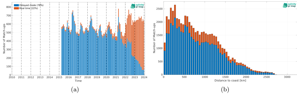
Figure 2: Number of match-ups between Argo and SMAP SSS L3 v5.0 - Monthly (JPL) SSS as a function of time (a) and as function of the distance to coast (b) over the Tropical Atlantic Ocean Pi-MEP region and for the full satellite product period.
