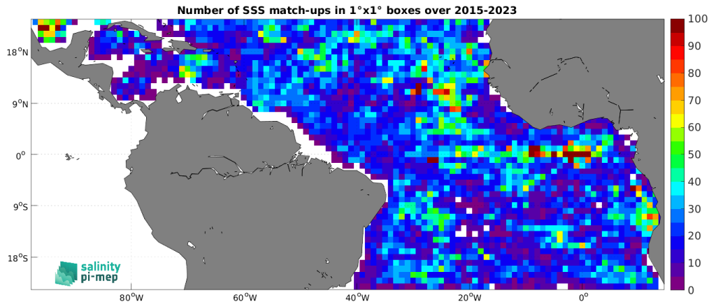
Figure 5: Number of SSS match-ups between Argo SSS and the SMAP SSS L3 v5.0 - Monthly (JPL) SSS product for the Tropical Atlantic Ocean Pi-MEP region over 1^\circ \times 1^\circ boxes and for the full satellite product period.
