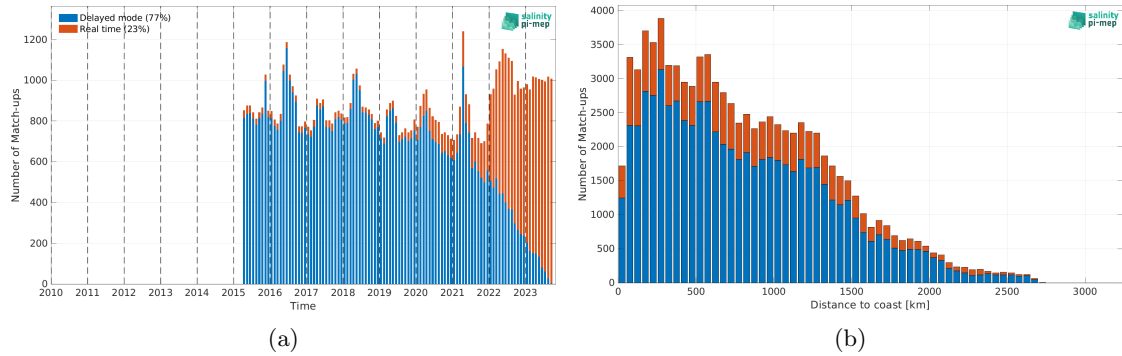
Figure 1: Number of match-ups between Argo and SMAP SSS L3 v5.0 - Monthly (JPL) SSS as a function of time (a) and as function of the distance to coast (b) over the Tropical Atlantic Ocean Pi-MEP region and for the full satellite product period.
