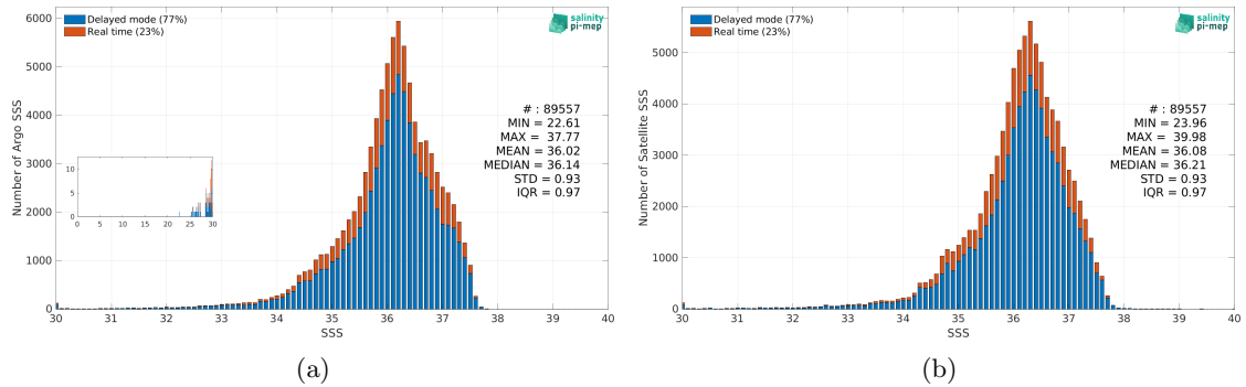
Figure 2: Histograms of SSS from Argo (a) and SMAP SSS L3 v5.0 - Monthly (JPL) (b) considering all match-up pairs per bins of 0.1 over the Tropical Atlantic Ocean Pi-MEP region and for the full satellite product period.
