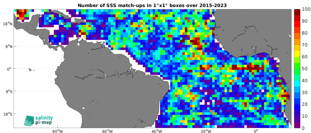
Figure 4: Number of SSS match-ups between Argo SSS and the SMAP SSS L3 v5.0 - Monthly (JPL) SSS product for the Tropical Atlantic Ocean Pi-MEP region over 1^\circ \times 1^\circ boxes and for the full satellite product period.
