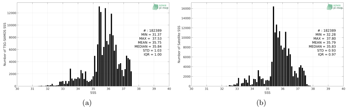
Figure 2: Histograms of SSS from TSG-SAMOS (a) and SMAP-L3-JPL-V4.3-8DAY-RUNNING-60KM (b) considering all match-up pairs per bins of 0.1 over the Tropical Atlantic Ocean Pi-MEP region and for the full satellite product period.
