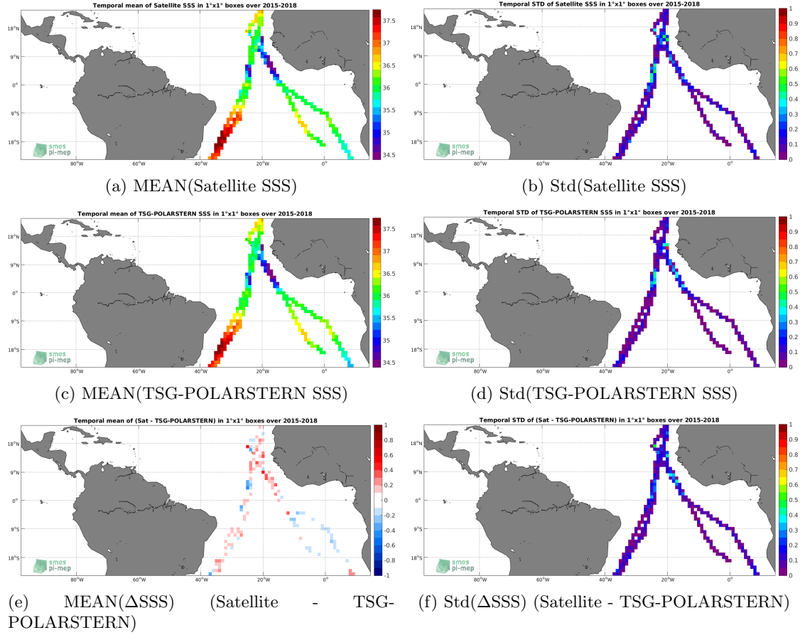
Figure 6: Temporal mean (left) and Std (right) of SSS from SMAP-L3-JPL-V4.3-8DAY-RUNNING-60KM (top), TSG-POLARSTERN (middle), and of \Delta SSS (Satellite - TSG-POLARSTERN). Only match-up pairs are used to generate these maps.
