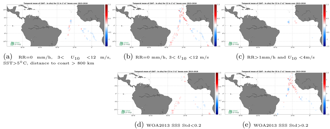
Figure 12: Temporal mean gridded over spatial boxes of size 1^\circ \times 1^\circ of \Delta SSS (SMAP-L3-JPL-V4.3-8DAY-RUNNING-60KM - TSG-POLARSTERN) for 5 different subdatasets corresponding to:RR=0 mm/h, 3 < U_{10} < 12 m/s, SST >5^\circ\text{C} , distance to coast > 800 km (a), RR=0 mm/h, 3 < U_{10} < 12 m/s (b), RR >1 mm/h and U_{10} < 4 m/s (c), WOA2013 SSS Std <0.2 (d), WOA2013 SSS Std >0.2 (e).
