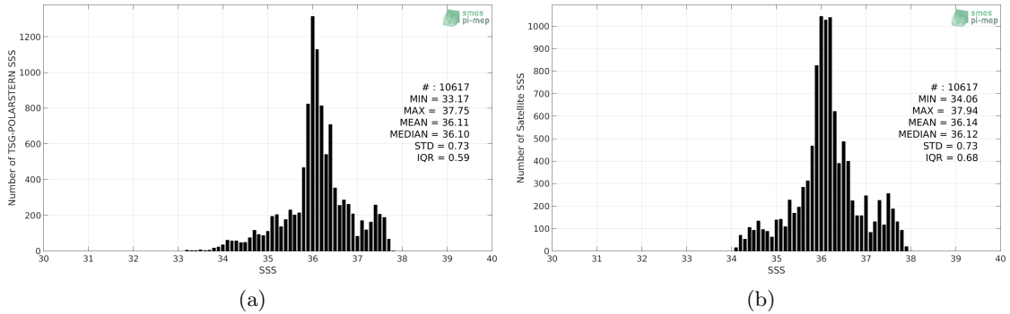
Figure 2: Histograms of SSS from TSG-POLARSTERN (a) and SMAP-L3-JPL-V4.3-8DAY-RUNNING-60KM (b) considering all match-up pairs per bins of 0.1 over the Tropical Atlantic Ocean Pi-MEP region and for the full satellite product period.
