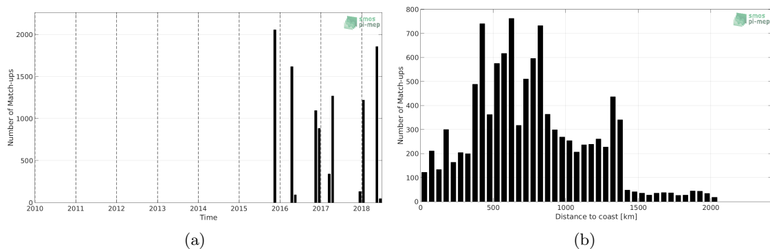
Figure 1: Number of match-ups between TSG-POLARSTERN and SMAP-L3-JPL-V4.3-8DAY-RUNNING-60KM SSS as a function of time (a) and as function of the distance to coast (b) over the Tropical Atlantic Ocean Pi-MEP region and for the full satellite product period.
