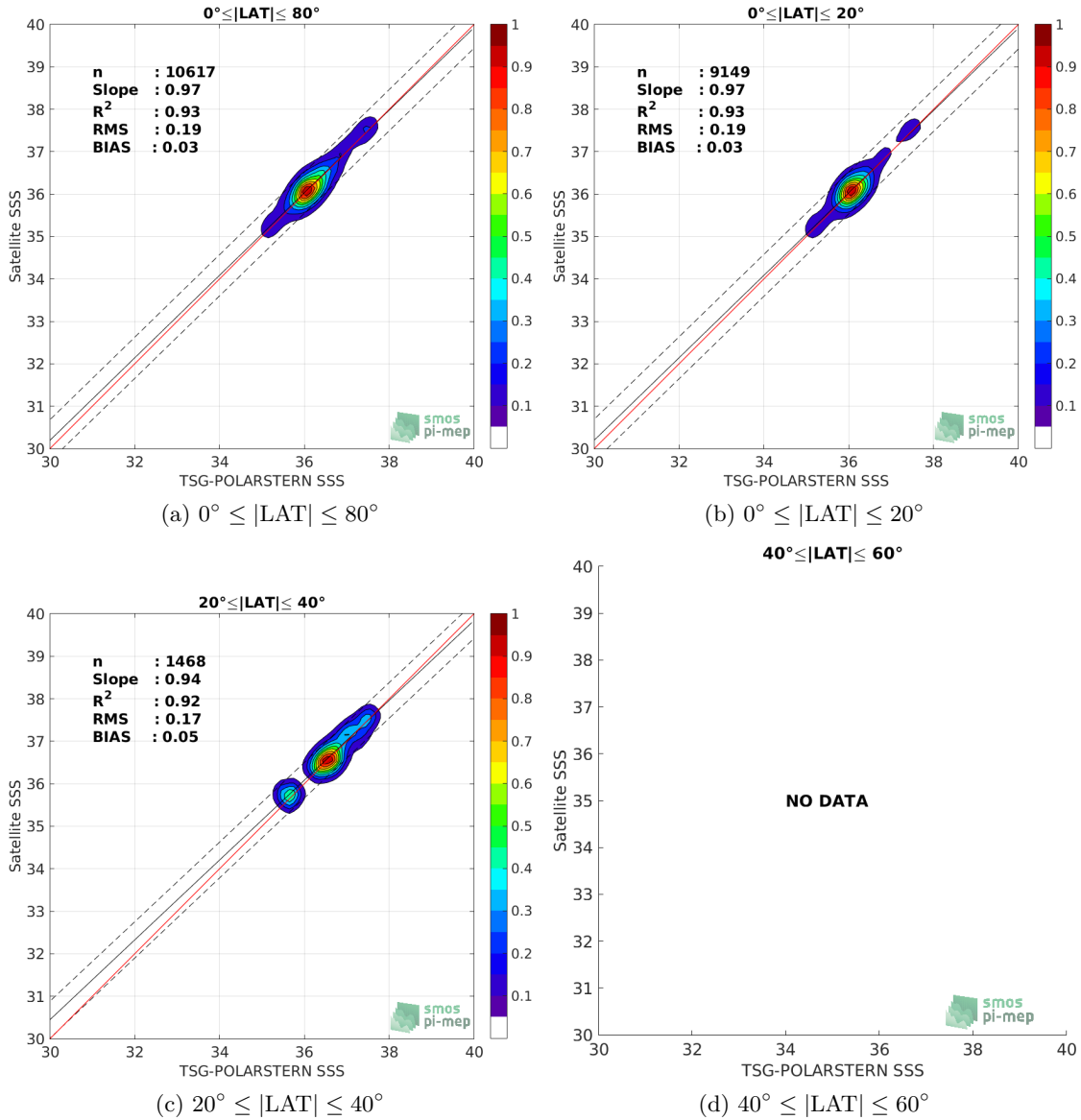
Figure 9: Contour maps of the concentration of SMAP-L3-JPL-V4.3-8DAY-RUNNING-60KM SSS (y-axis) versus TSG-POLARSTERN SSS (x-axis) at match-up pairs for different latitude bands. For each plot, the red line shows x=y . The black thin and dashed lines indicate a linear fit through the data cloud and the \pm 95\% confidence levels, respectively. The number match-up pairs n , the slope and R^2 coefficient of the linear fit, the root mean square (RMS) and the mean bias between satellite and in situ data are indicated for each latitude band in each plots.
