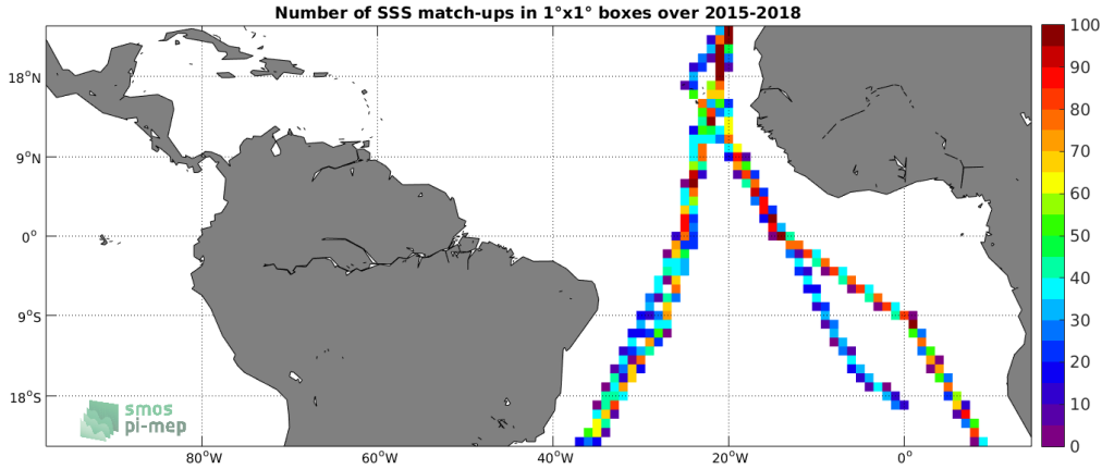
Figure 4: Number of SSS match-ups between TSG-POLARSTERN SSS and the SMAP-L3-JPL-V4.3-8DAY-RUNNING-60KM SSS product for the Tropical Atlantic Ocean Pi-MEP region over 1^\circ \times 1^\circ boxes and for the full satellite product period.
