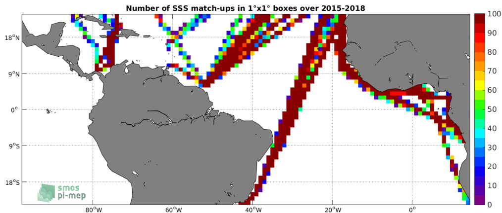
Figure 4: Number of SSS match-ups between TSG-LEGOS-DM SSS and the SMAP-L3-JPL-V4.3-8DAY-RUNNING-60KM SSS product for the Tropical Atlantic Ocean Pi-MEP region over 1^\circ \times 1^\circ boxes and for the full satellite product period.
