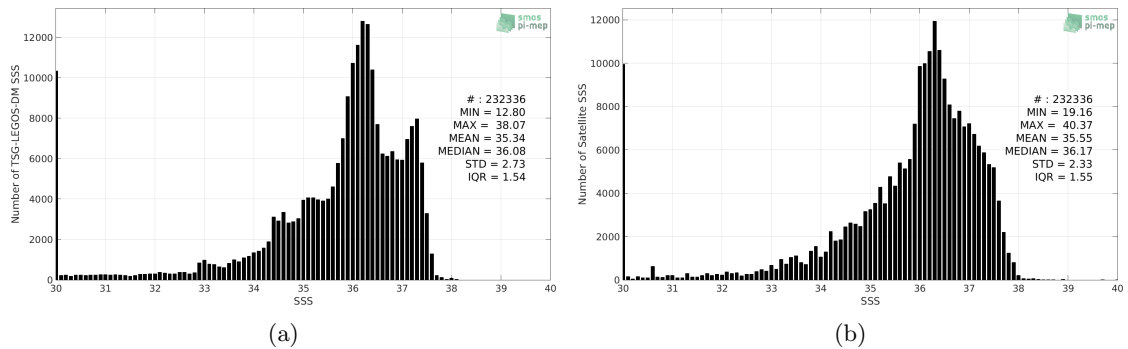
Figure 2: Histograms of SSS from TSG-LEGOS-DM (a) and SMAP-L3-JPL-V4.3-8DAY-RUNNING-60KM (b) considering all match-up pairs per bins of 0.1 over the Tropical Atlantic Ocean Pi-MEP region and for the full satellite product period.
