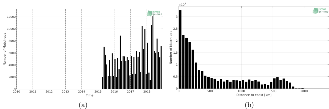
Figure 1: Number of match-ups between TSG-LEGOS-DM and SMAP-L3-JPL-V4.3-8DAY-RUNNING-60KM SSS as a function of time (a) and as function of the distance to coast (b) over the Tropical Atlantic Ocean Pi-MEP region and for the full satellite product period.
