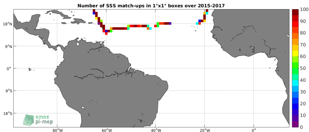
Figure 4: Number of SSS match-ups between TSG-GOSUD-Sailing-ship SSS and the SMAP-L3-JPL-V4.3-8DAY-RUNNING-60KM SSS product for the Tropical Atlantic Ocean Pi-MEP region over 1^\circ \times 1^\circ boxes and for the full satellite product period.
