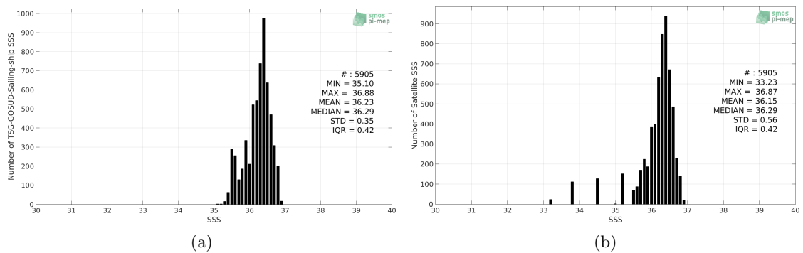
Figure 2: Histograms of SSS from TSG-GOSUD-Sailing-ship (a) and SMAP-L3-JPL-V4.3-8DAY-RUNNING-60KM (b) considering all match-up pairs per bins of 0.1 over the Tropical Atlantic Ocean Pi-MEP region and for the full satellite product period.
