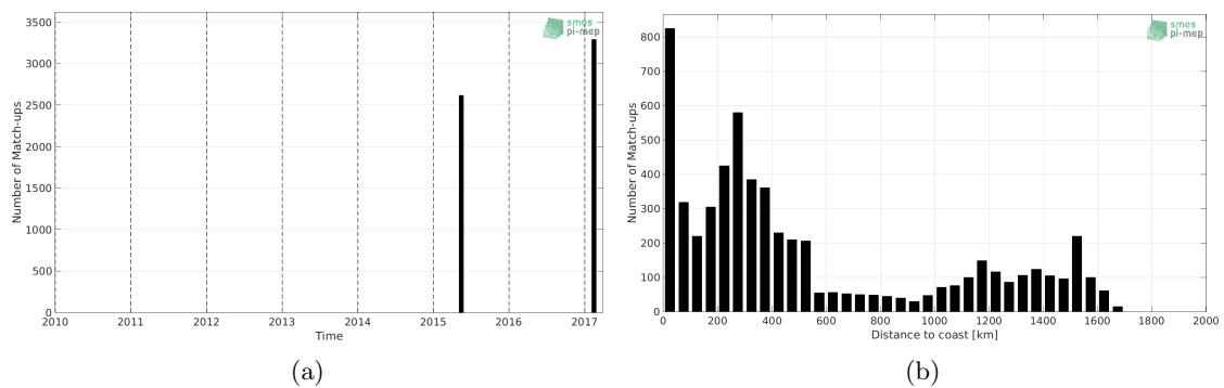
Figure 1: Number of match-ups between TSG-GOSUD-Sailing-ship and SMAP-L3-JPL-V4.3-8DAY-RUNNING-60KM SSS as a function of time (a) and as function of the distance to coast (b) over the Tropical Atlantic Ocean Pi-MEP region and for the full satellite product period.
