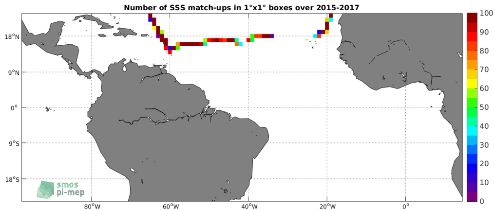
Figure 4: Number of SSS match-ups between TSG-GOSUD-Sailing-ship SSS and the SMAP-L3-JPL-V4.3-8DAY-RUNNING-60KM SSS product for the Tropical Atlantic Ocean Pi-MEP region over 1°x1° boxes and for the full satellite product period.
