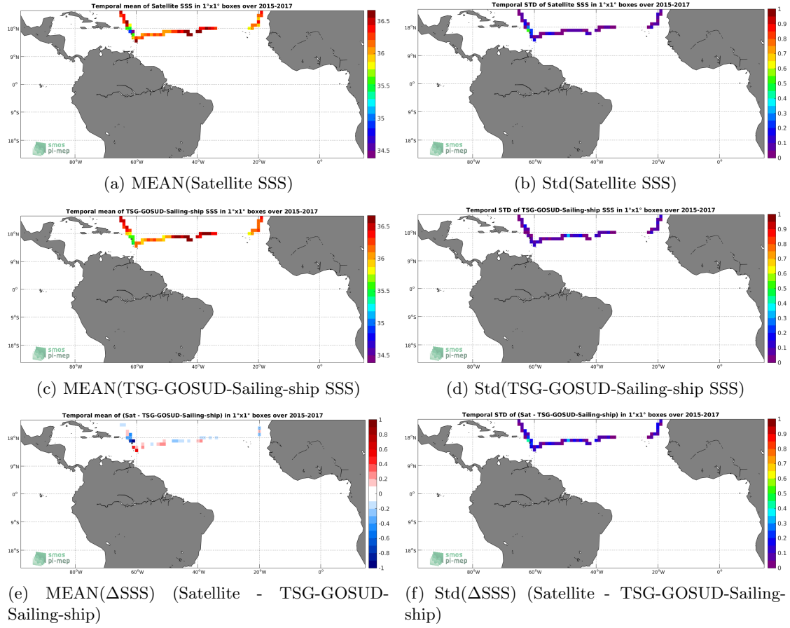
Figure 6: Temporal mean (left) and Std (right) of SSS from SMAP-L3-JPL-V4.3-8DAY-RUNNING-60KM (top), TSG-GOSUD-Sailing-ship (middle), and of \Delta SSS (Satellite - TSG-GOSUD-Sailing-ship). Only match-up pairs are used to generate these maps.
