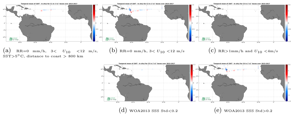
Figure 12: Temporal mean gridded over spatial boxes of size 1^\circ \times 1^\circ of \Delta SSS (SMAP-L3-JPL-V4.3-8DAY-RUNNING-60KM - TSG-GOSUD-Sailing-ship) for 5 different subdatasets corresponding to:RR=0 mm/h, 3 < U_{10} < 12 m/s, SST>5°C, distance to coast > 800 km (a), RR=0 mm/h, 3 < U_{10} < 12 m/s (b), RR>1mm/h and U_{10} < 4 m/s (c), WOA2013 SSS Std<0.2 (d), WOA2013 SSS Std>0.2 (e).
