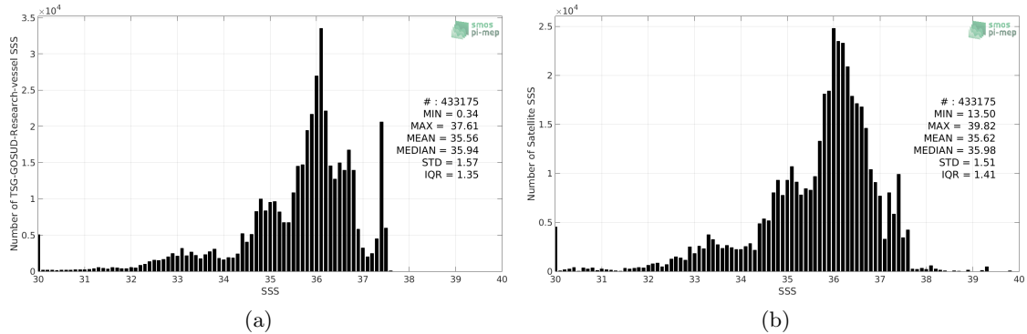
Figure 2: Histograms of SSS from TSG-GOSUD-Research-vessel (a) and SMAP-L3-JPL-V4.3-8DAY-RUNNING-60KM (b) considering all match-up pairs per bins of 0.1 over the Tropical Atlantic Ocean Pi-MEP region and for the full satellite product period.
