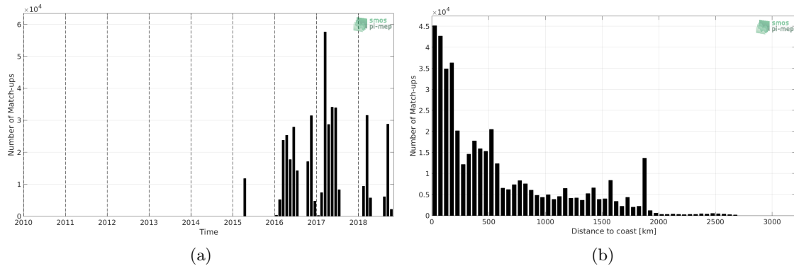
Figure 1: Number of match-ups between TSG-GOSUD-Research-vessel and SMAP-L3-JPL-V4.3-8DAY-RUNNING-60KM SSS as a function of time (a) and as function of the distance to coast (b) over the Tropical Atlantic Ocean Pi-MEP region and for the full satellite product period.
