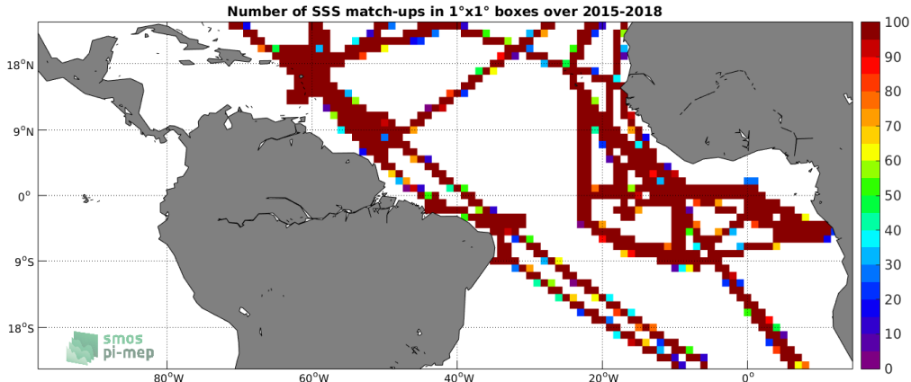
Figure 4: Number of SSS match-ups between TSG-GOSUD-Research-vessel SSS and the SMAP-L3-JPL-V4.3-8DAY-RUNNING-60KM SSS product for the Tropical Atlantic Ocean Pi-MEP region over 1^\circ \times 1^\circ boxes and for the full satellite product period.
