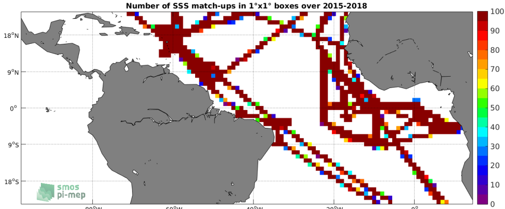
Figure 4: Number of SSS match-ups between TSG-GOSUD-Research-vessel SSS and the SMAP-L3-JPL-V4.3-8DAY-RUNNING-60KM SSS product for the Tropical Atlantic Ocean Pi-MEP region over 1°x1° boxes and for the full satellite product period.
