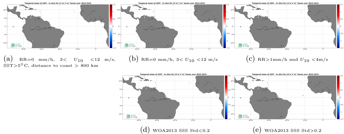
Figure 11: Temporal mean gridded over spatial boxes of size 1^{\circ}\times 1^{\circ} of \Delta\text{SSS} (SMAP-L3-JPL-V4.3-8DAY-RUNNING-60KM - Surface drifters) for 5 different subdatasets corresponding to:RR=0 mm/h, 3 < U_{10} < 12 m/s, SST > 5^{\circ}\text{C} , distance to coast > 800 km (a), RR=0 mm/h, 3 < U_{10} < 12 m/s (b), RR > 1 mm/h and U_{10} < 4 m/s (c), WOA2013 SSS Std < 0.2 (d), WOA2013 SSS Std > 0.2 (e).
