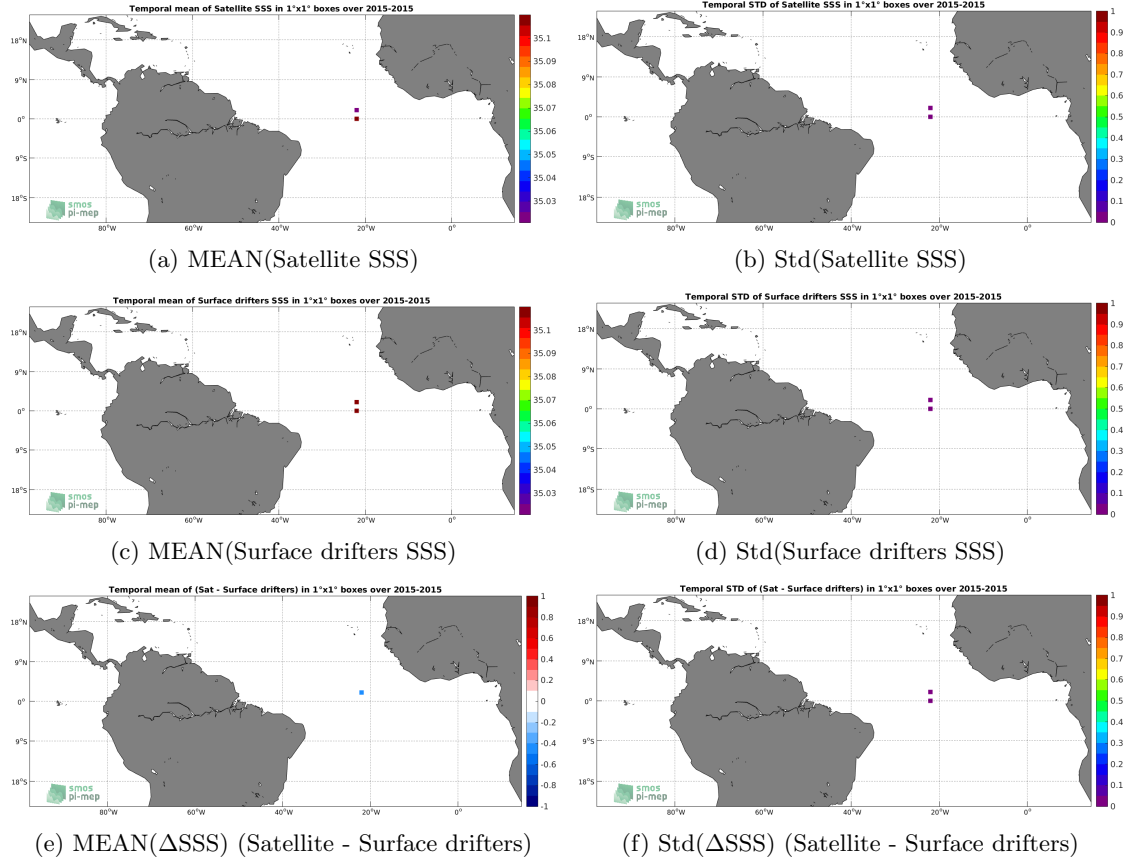
Figure 5: Temporal mean (left) and Std (right) of SSS from SMAP-L3-JPL-V4.3-8DAY-RUNNING-60KM (top), Surface drifters (middle), and of \Delta SSS (Satellite - Surface drifters). Only match-up pairs are used to generate these maps.
