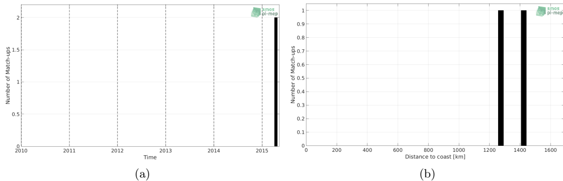
Figure 1: Number of match-ups between Surface drifters and SMAP-L3-JPL-V4.3-8DAY-RUNNING-60KM SSS as a function of time (a) and as function of the distance to coast (b) over the Tropical Atlantic Ocean Pi-MEP region and for the full satellite product period.
