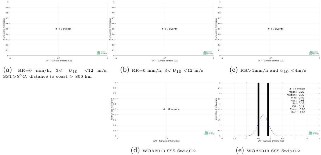
Figure 12: Normalized histogram of \Delta\text{SSS} (SMAP-L3-JPL-V4.3-8DAY-RUNNING-60KM - Surface drifters) for 5 different subdatasets corresponding to: RR=0 mm/h, 3 < U_{10} < 12 m/s, SST > 5^\circ\text{C} , distance to coast > 800 km (a), RR=0 mm/h, 3 < U_{10} < 12 m/s (b), RR > 1\text{mm/h} and U_{10} < 4\text{m/s} (c), WOA2013 SSS Std < 0.2 (d), WOA2013 SSS Std > 0.2 (e).
