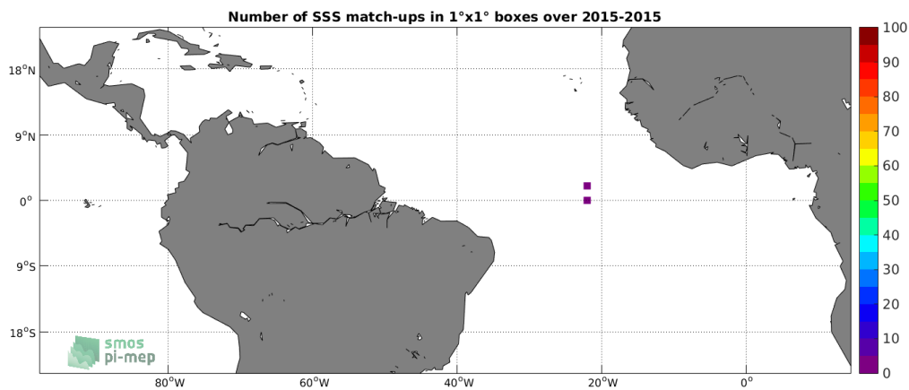
Figure 3: Number of SSS match-ups between Surface drifters SSS and the SMAP-L3-JPL-V4.3-8DAY-RUNNING-60KM SSS product for the Tropical Atlantic Ocean Pi-MEP region over 1°x1° boxes and for the full satellite product period.
