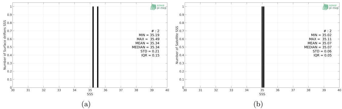
Figure 2: Histograms of SSS from Surface drifters (a) and SMAP-L3-JPL-V4.3-8DAY-RUNNING-60KM (b) considering all match-up pairs per bins of 0.1 over the Tropical Atlantic Ocean Pi-MEP region and for the full satellite product period.
