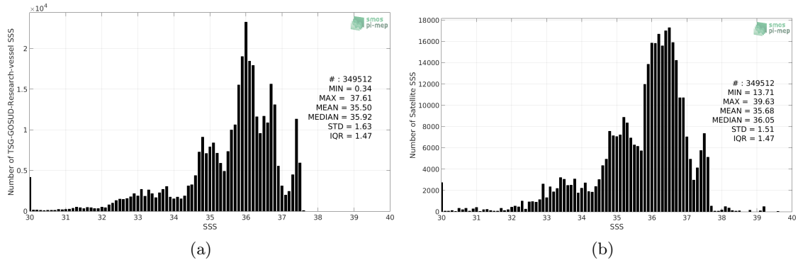
Figure 2: Histograms of SSS from TSG-GOSUD-Research-vessel (a) and SMAP-L3-JPL-V4.2-8DAY-RUNNING-60KM (b) considering all match-up pairs per bins of 0.1 over the Tropical Atlantic Ocean Pi-MEP region and for the full satellite product period.
