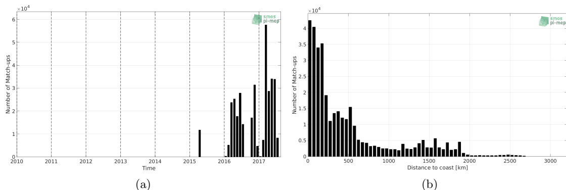
Figure 1: Number of match-ups between TSG-GOSUD-Research-vessel and SMAP-L3-JPL-V4.2-8DAY-RUNNING-60KM SSS as a function of time (a) and as function of the distance to coast (b) over the Tropical Atlantic Ocean Pi-MEP region and for the full satellite product period.
