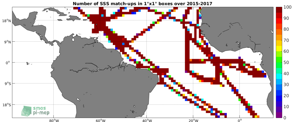
Figure 4: Number of SSS match-ups between TSG-GOSUD-Research-vessel SSS and the SMAP-L3-JPL-V4.2-8DAY-RUNNING-60KM SSS product for the Tropical Atlantic Ocean Pi-MEP region over 1^\circ \times 1^\circ boxes and for the full satellite product period.
