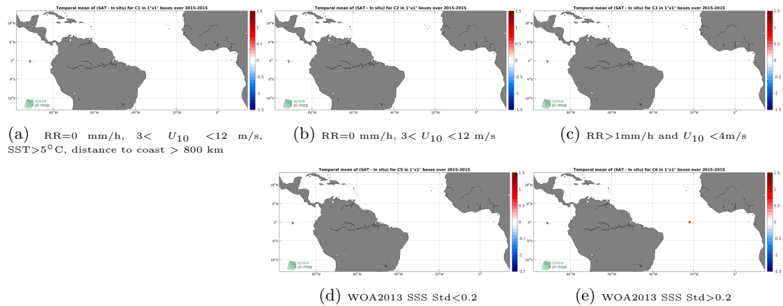
Figure 11: Temporal mean gridded over spatial boxes of size 1^\circ \times 1^\circ of \Delta SSS (SMAP-L3-JPL-V4.2-MONTHLY-60KM - Surface drifters) for 5 different subdatasets corresponding to:RR=0 mm/h, 3 < U_{10} < 12 m/s, SST >5^\circ\text{C} , distance to coast > 800 km (a), RR=0 mm/h, 3 < U_{10} < 12 m/s (b), RR >1 mm/h and U_{10} < 4 m/s (c), WOA2013 SSS Std <0.2 (d), WOA2013 SSS Std >0.2 (e).
