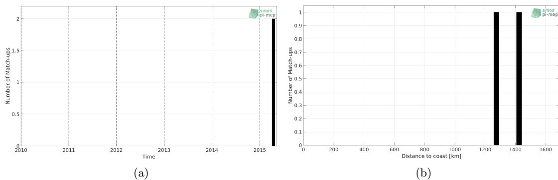
Figure 1: Number of match-ups between Surface drifters and SMAP-L3-JPL-V4.2-MONTHLY-60KM SSS as a function of time (a) and as function of the distance to coast (b) over the Tropical Atlantic Ocean Pi-MEP region and for the full satellite product period.
