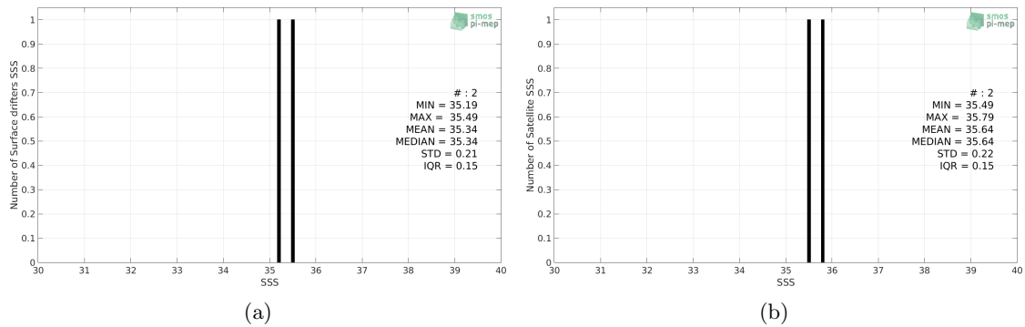
Figure 2: Histograms of SSS from Surface drifters (a) and SMAP-L3-JPL-V4.2-MONTHLY-60KM (b) considering all match-up pairs per bins of 0.1 over the Tropical Atlantic Ocean Pi-MEP region and for the full satellite product period.
