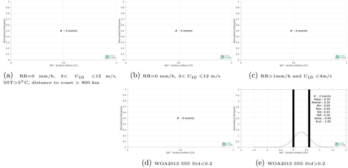
Figure 12: Normalized histogram of \Delta\text{SSS} (SMAP-L3-JPL-V4.2-MONTHLY-60KM - Surface drifters) for 5 different subdatasets corresponding to: RR=0 mm/h, 3 < U_{10} < 12 m/s, SST > 5^\circ\text{C} , distance to coast > 800 km (a), RR=0 mm/h, 3 < U_{10} < 12 m/s (b), RR > 1\text{mm/h} and U_{10} < 4\text{m/s} (c), WOA2013 SSS Std < 0.2 (d), WOA2013 SSS Std > 0.2 (e).
