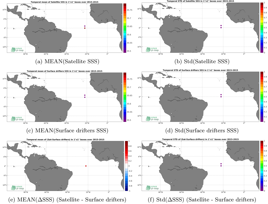
Figure 5: Temporal mean (left) and Std (right) of SSS from SMAP-L3-JPL-V4.2-MONTHLY-60KM (top), Surface drifters (middle), and of \Delta SSS (Satellite - Surface drifters). Only match-up pairs are used to generate these maps.
