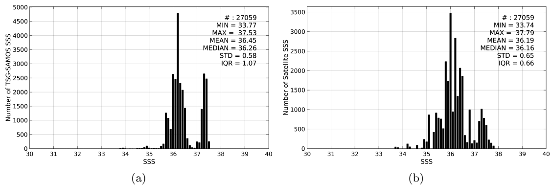
Figure 2: Histograms of SSS from TSG-SAMOS (a) and SMAP-L3-JPL-V4-8DAY-RUNNING-60KM (b) considering all match-up pairs per bins of 0.1 over the Tropical Atlantic Ocean Pi-MEP region and for the full satellite product period.
