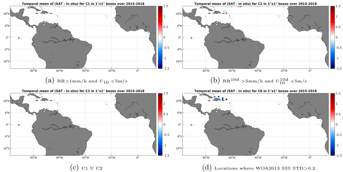
Figure 12: Temporal mean gridded over spatial boxes of size 1^\circ \times 1^\circ of \Delta SSS (SMAP-L3-JPL-V4-8DAY-RUNNING-60KM - TSG-SAMOS) for 4 different subdatasets corresponding to: RR > 1 mm/h and U_{10} < 5 m/s (a), RR 10d > 5 mm/h and U_{10}^{10d} < 5 m/s (b), C1 U C2 (c), Locations where WOA2013 SSS STD > 0.2 (d).
