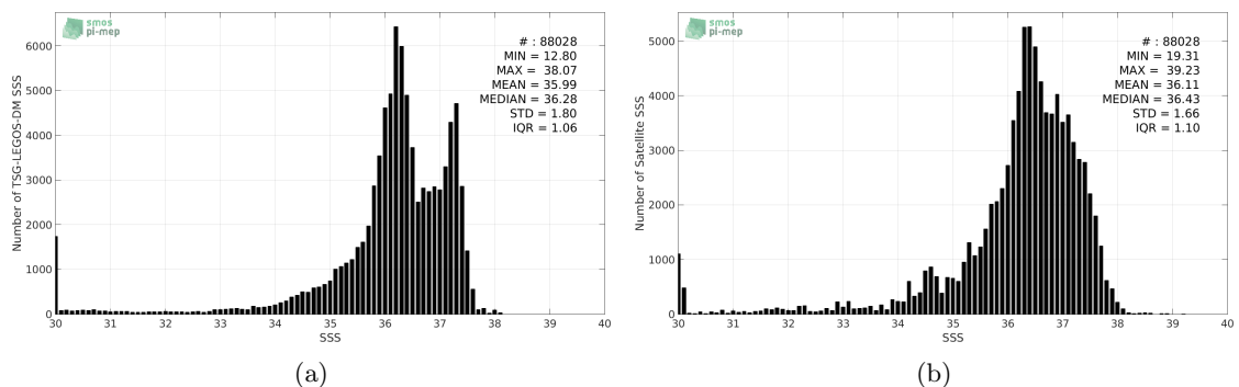
Figure 2: Histograms of SSS from TSG-LEGOS-DM (a) and SMAP-L3-JPL-V4-8DAY-RUNNING-60KM (b) considering all match-up pairs per bins of 0.1 over the Tropical Atlantic Ocean Pi-MEP region and for the full satellite product period.
