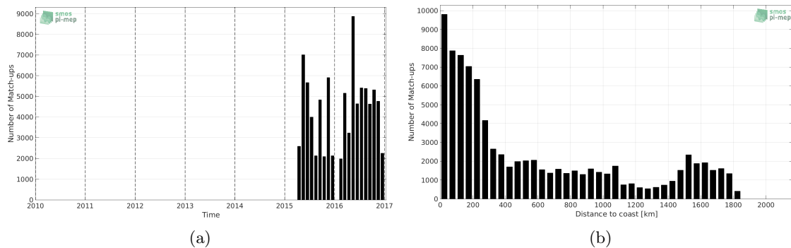
Figure 1: Number of match-ups between TSG-LEGOS-DM and SMAP-L3-JPL-V4-8DAY-RUNNING-60KM SSS as a function of time (a) and as function of the distance to coast (b) over the Tropical Atlantic Ocean Pi-MEP region and for the full satellite product period.
