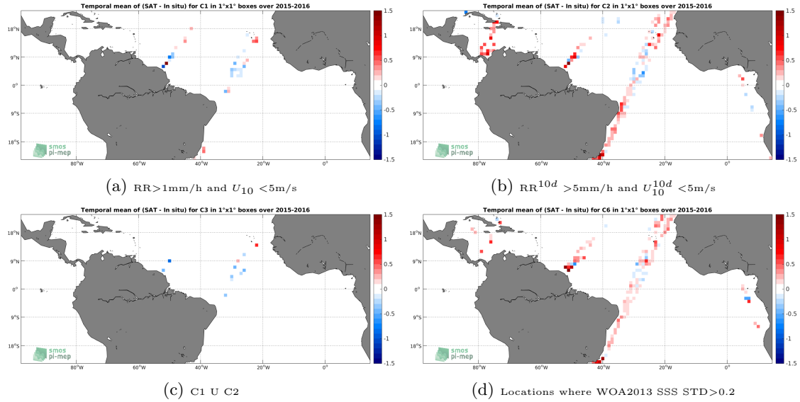
Figure 12: Temporal mean gridded over spatial boxes of size 1^\circ \times 1^\circ of \Delta SSS (SMAP-L3-JPL-V4-8DAY-RUNNING-60KM - TSG-LEGOS-DM) for 4 different subdatasets corresponding to: RR > 1\text{mm/h} and U_{10} < 5\text{m/s} (a), RR^{10d} > 5\text{mm/h} and U_{10}^{10d} < 5\text{m/s} (b), C1 U C2 (c), Locations where WOA2013 SSS STD > 0.2 (d).
