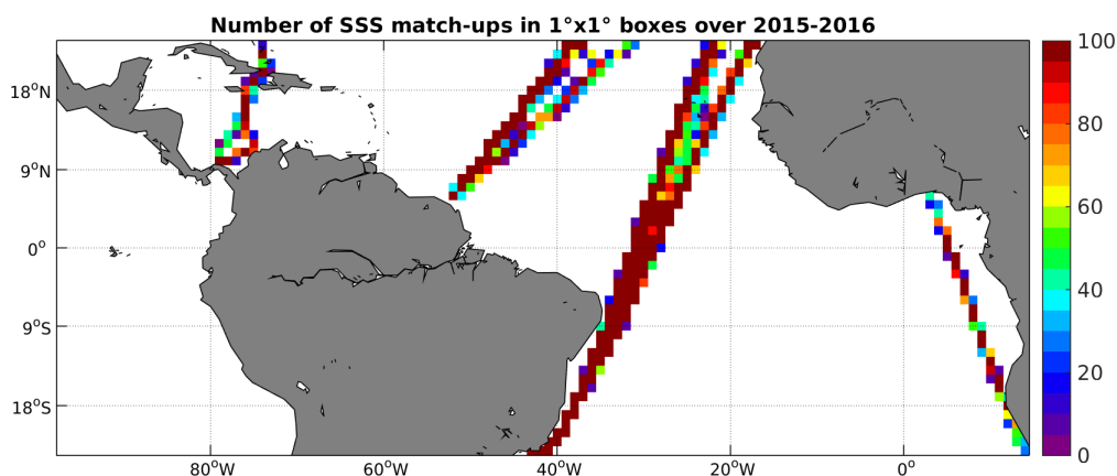
Figure 4: Number of SSS match-ups between TSG-LEGOS-DM SSS and the SMAP-L3-JPL-V4-8DAY-RUNNING-60KM SSS product for the Tropical Atlantic Ocean Pi-MEP region over 1^\circ \times 1^\circ boxes and for the full satellite product period.
