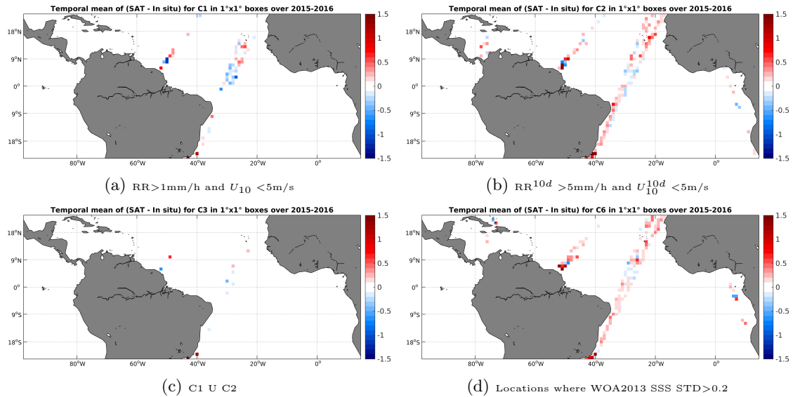
Figure 12: Temporal mean gridded over spatial boxes of size 1^\circ \times 1^\circ of \Delta SSS (SMAP-L3-JPL-V4-8DAY-RUNNING-60KM - TSG-LEGOS-DM) for 4 different subdatasets corresponding to: RR > 1mm/h and U_{10} < 5 m/s (a), RR^{10d} > 5 mm/h and U_{10}^{10d} < 5 m/s (b), C1 U C2 (c), Locations where WOA2013 SSS STD > 0.2 (d).
