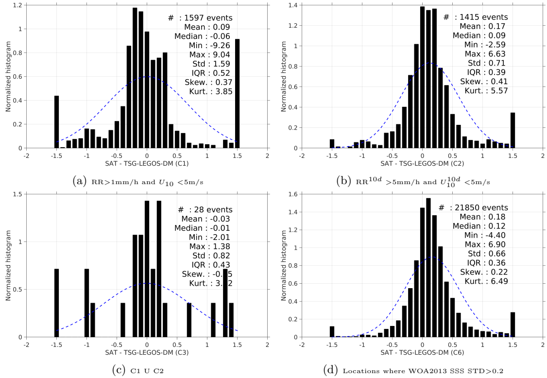
Figure 13: Normalized histogram of \Delta\text{SSS} (SMAP-L3-JPL-V4-8DAY-RUNNING-60KM - TSG-LEGOS-DM) for 6 different subdatasets corresponding to: RR > 1mm/h and U_{10} < 5\text{m/s} (a), RR^{10d} > 5\text{mm/h} and U_{10}^{10d} < 5\text{m/s} (b), C1 U C2 (c), Locations where WOA2013 SSS STD > 0.2 (d).
