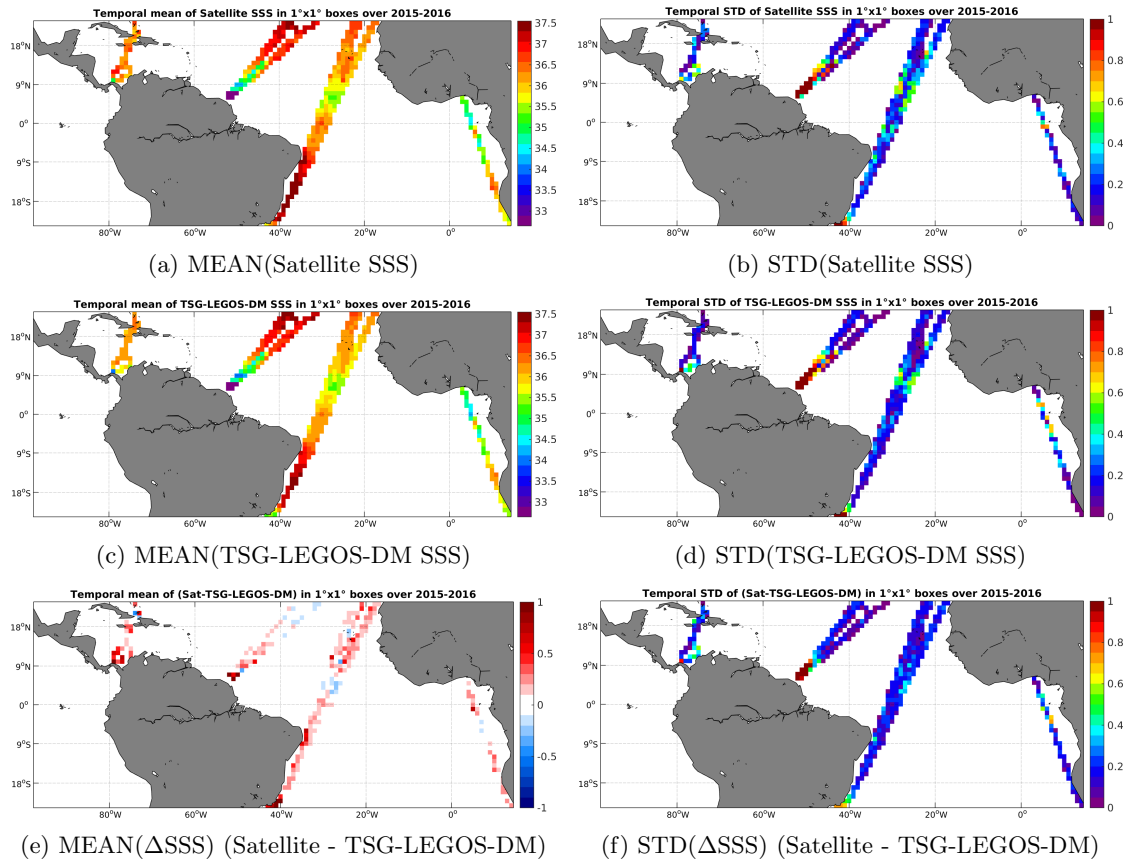
Figure 6: Temporal mean (left) and STD (right) of SSS from SMAP-L3-JPL-V4-8DAY-RUNNING-60KM (top), TSG-LEGOS-DM (middle), and of \Delta SSS (Satellite - TSG-LEGOS-DM). Only match-up pairs are used to generate these maps.
