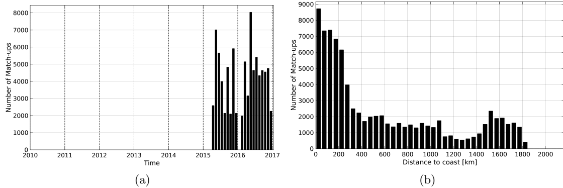
Figure 1: Number of match-ups between TSG-LEGOS-DM and SMAP-L3-JPL-V4-8DAY-RUNNING-60KM SSS as a function of time (a) and as function of the distance to coast (b) over the Tropical Atlantic Ocean Pi-MEP region and for the full satellite product period.
