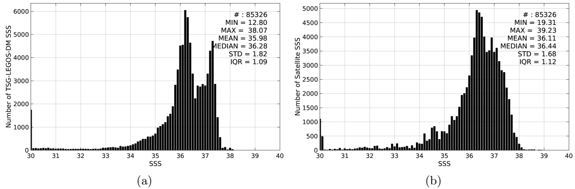
Figure 2: Histograms of SSS from TSG-LEGOS-DM (a) and SMAP-L3-JPL-V4-8DAY-RUNNING-60KM (b) considering all match-up pairs per bins of 0.1 over the Tropical Atlantic Ocean Pi-MEP region and for the full satellite product period.
