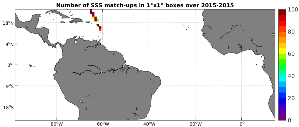
Figure 4: Number of SSS match-ups between TSG-GOSUD-Sailing-ship SSS and the SMAP-L3-JPL-V4-8DAY-RUNNING-60KM SSS product for the Tropical Atlantic Ocean Pi-MEP region over 1^\circ \times 1^\circ boxes and for the full satellite product period.
