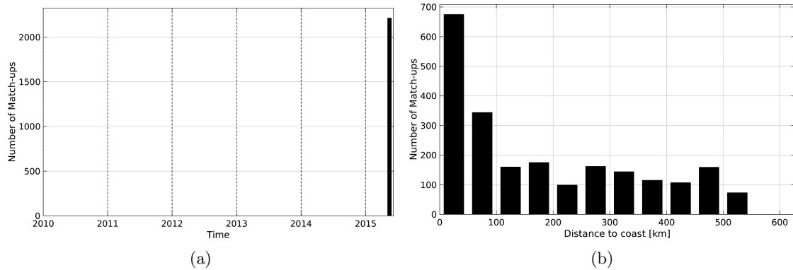
Figure 1: Number of match-ups between TSG-GOSUD-Sailing-ship and SMAP-L3-JPL-V4-8DAY-RUNNING-60KM SSS as a function of time (a) and as function of the distance to coast (b) over the Tropical Atlantic Ocean Pi-MEP region and for the full satellite product period.
