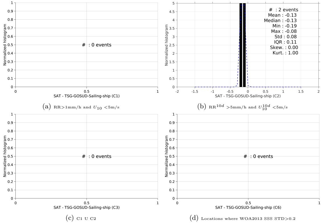
Figure 13: Normalized histogram of \Delta\text{SSS} (SMAP-L3-JPL-V4-8DAY-RUNNING-60KM - TSG-GOSUD-Sailing-ship) for 6 different subdatasets corresponding to: RR > 1\text{mm/h} and U_{10} < 5\text{m/s} (a), RR^{10d} > 5\text{mm/h} and U_{10}^{10d} < 5\text{m/s} (b), C1 U C2 (c), Locations where WOA2013 SSS STD > 0.2 (d).
