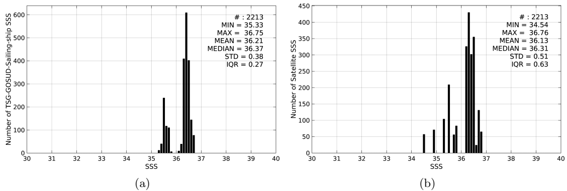
Figure 2: Histograms of SSS from TSG-GOSUD-Sailing-ship (a) and SMAP-L3-JPL-V4-8DAY-RUNNING-60KM (b) considering all match-up pairs per bins of 0.1 over the Tropical Atlantic Ocean Pi-MEP region and for the full satellite product period.
