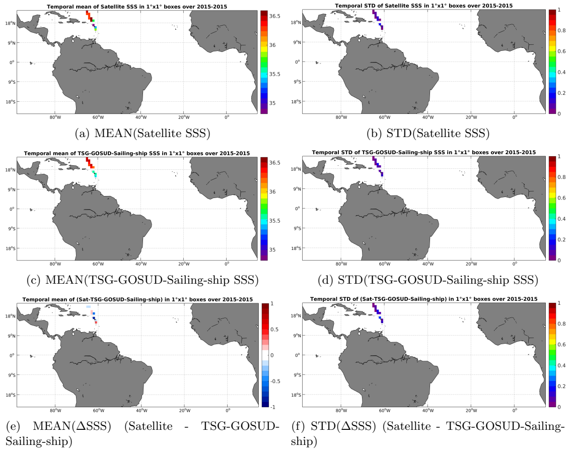
Figure 6: Temporal mean (left) and STD (right) of SSS from SMAP-L3-JPL-V4-8DAY-RUNNING-60KM (top), TSG-GOSUD-Sailing-ship (middle), and of \Delta SSS (Satellite - TSG-GOSUD-Sailing-ship). Only match-up pairs are used to generate these maps.
