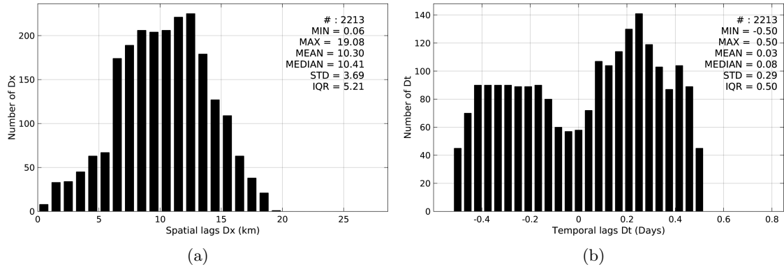
Figure 5: Histograms of the spatial (a) and temporal (b) lags between the time of the TSG-GOSUD-Sailing-ship measurements and the date of the corresponding SMAP-L3-JPL-V4-8DAY-RUNNING-60KM SSS product.
