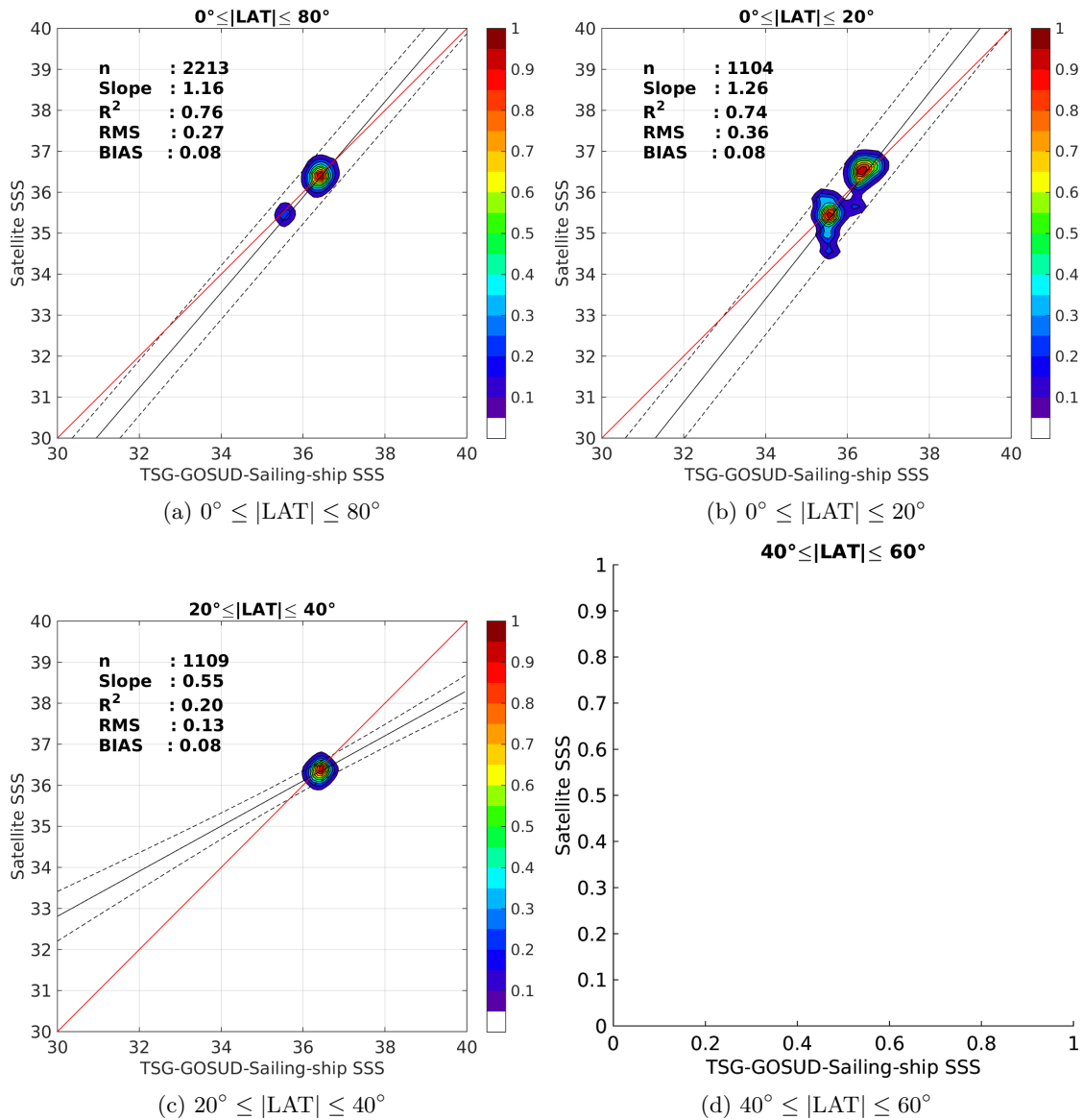
Figure 9: Contour maps of the concentration of SMAP-L3-JPL-V4-8DAY-RUNNING-60KM SSS (y-axis) versus TSG-GOSUD-Sailing-ship SSS (x-axis) at match-up pairs for different latitude bands. For each plot, the red line shows x=y . The black thin and dashed lines indicate a linear fit through the data cloud and the \pm 95\% confidence levels, respectively. The number match-up pairs n , the slope and R^2 coefficient of the linear fit, the root mean square (RMS) and the mean bias between satellite and in situ data are indicated for each latitude band in each plots.
