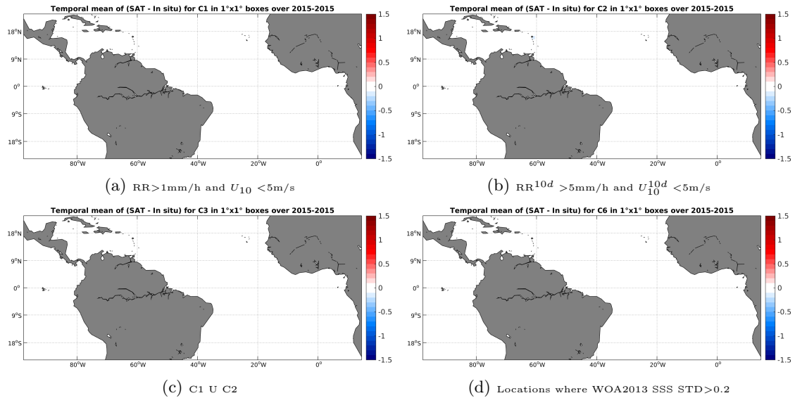
Figure 12: Temporal mean gridded over spatial boxes of size 1^\circ \times 1^\circ of \Delta SSS (SMAP-L3-JPL-V4-8DAY-RUNNING-60KM - TSG-GOSUD-Sailing-ship) for 4 different subdatasets corresponding to:RR>1mm/h and U_{10} < 5m/s (a), RR^{10d} > 5mm/h and U_{10d} < 5m/s (b), C1 U C2 (c),Locations where WOA2013 SSS STD>0.2 (d).
