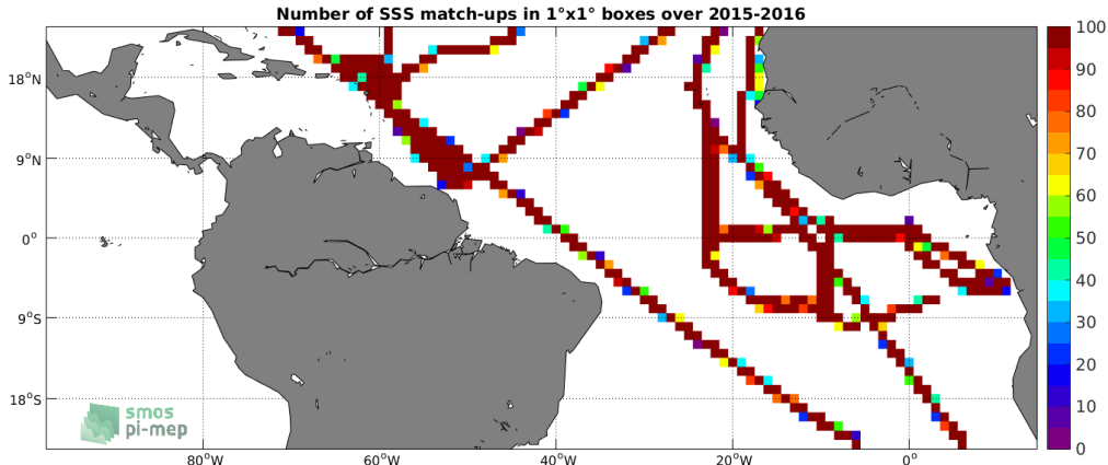
Figure 4: Number of SSS match-ups between TSG-GOSUD-Research-vessel SSS and the SMAP-L3-JPL-V4-8DAY-RUNNING-60KM SSS product for the Tropical Atlantic Ocean Pi-MEP region over 1^\circ \times 1^\circ boxes and for the full satellite product period.
