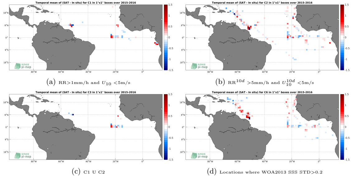
Figure 12: Temporal mean gridded over spatial boxes of size 1^\circ \times 1^\circ of \Delta SSS (SMAP-L3-JPL-V4-8DAY-RUNNING-60KM - TSG-GOSUD-Research-vessel) for 4 different subdatasets corresponding to: RR > 1\text{mm/h} and U_{10} < 5\text{m/s} (a), RR^{10d} > 5\text{mm/h} and U_{10}^{10d} < 5\text{m/s} (b), C1 U C2 (c), Locations where WOA2013 SSS STD > 0.2 (d).
