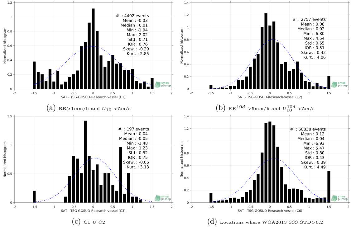
Figure 13: Normalized histogram of \Delta SSS (SMAP-L3-JPL-V4-8DAY-RUNNING-60KM - TSG-GOSUD-Research-vessel) for 6 different subdatasets corresponding to: RR > 1mm/h and U_{10} < 5 m/s (a), RR^{10d} > 5 mm/h and U_{10}^{10d} < 5 m/s (b), C1 U C2 (c), Locations where WOA2013 SSS STD > 0.2 (d).
