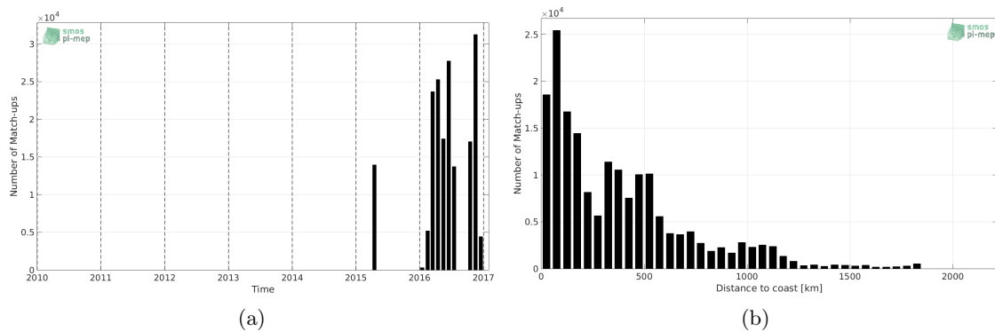
Figure 1: Number of match-ups between TSG-GOSUD-Research-vessel and SMAP-L3-JPL-V4-8DAY-RUNNING-60KM SSS as a function of time (a) and as function of the distance to coast (b) over the Tropical Atlantic Ocean Pi-MEP region and for the full satellite product period.
