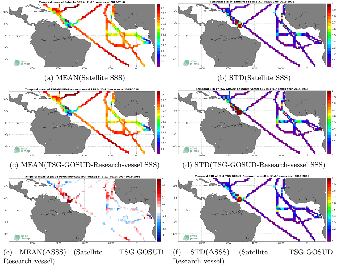
Figure 6: Temporal mean (left) and STD (right) of SSS from SMAP-L3-JPL-V4-8DAY-RUNNING-60KM (top), TSG-GOSUD-Research-vessel (middle), and of \Delta SSS (Satellite - TSG-GOSUD-Research-vessel). Only match-up pairs are used to generate these maps.
