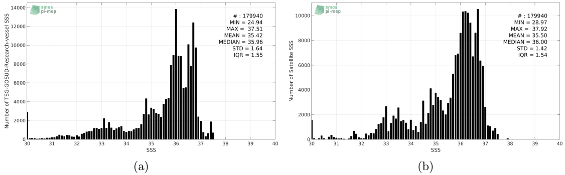
Figure 2: Histograms of SSS from TSG-GOSUD-Research-vessel (a) and SMAP-L3-JPL-V4-8DAY-RUNNING-60KM (b) considering all match-up pairs per bins of 0.1 over the Tropical Atlantic Ocean Pi-MEP region and for the full satellite product period.
