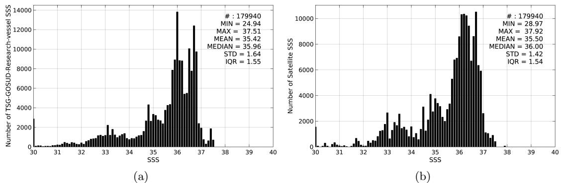
Figure 2: Histograms of SSS from TSG-GOSUD-Research-vessel (a) and SMAP-L3-JPL-V4-8DAY-RUNNING-60KM (b) considering all match-up pairs per bins of 0.1 over the Tropical Atlantic Ocean Pi-MEP region and for the full satellite product period.
