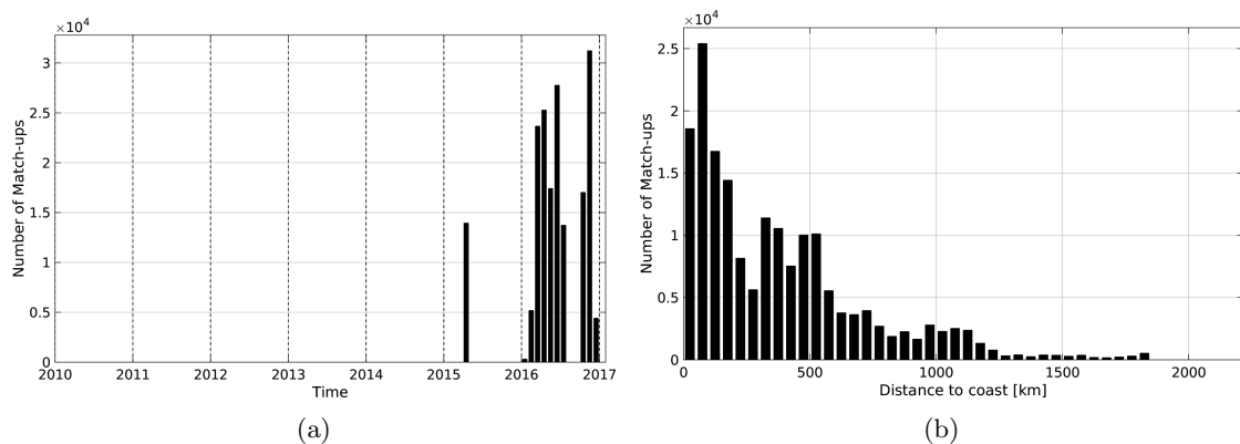
Figure 1: Number of match-ups between TSG-GOSUD-Research-vessel and SMAP-L3-JPL-V4-8DAY-RUNNING-60KM SSS as a function of time (a) and as function of the distance to coast (b) over the Tropical Atlantic Ocean Pi-MEP region and for the full satellite product period.
