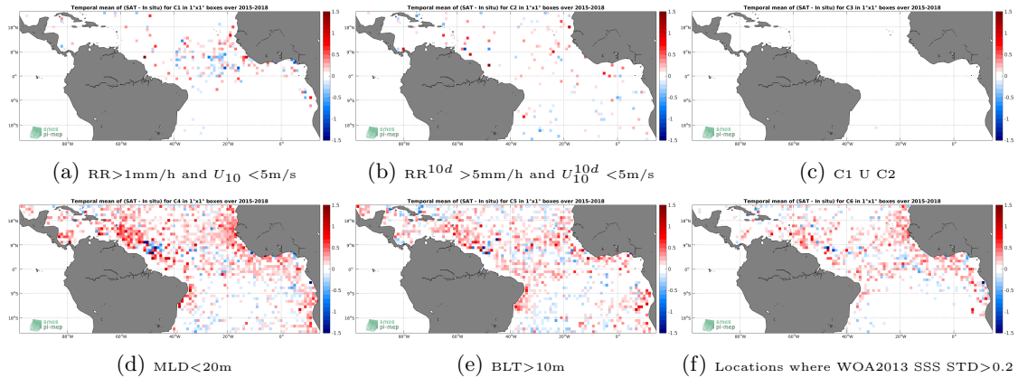
Figure 12: Temporal mean gridded over spatial boxes of size 1^\circ \times 1^\circ of \Delta SSS (SMAP-L3-JPL-V4-8DAY-RUNNING-60KM - Argo) for 6 different subdatasets corresponding to: RR > 1\text{mm/h} and U_{10} < 5\text{m/s} (a), RR^{10d} > 5\text{mm/h} and U_{10}^{10d} < 5\text{m/s} (b), C1 U C2 (c), MLD < 20\text{m} (d), BLT > 10\text{m} (e), Locations where WOA2013 SSS STD > 0.2 (f).
