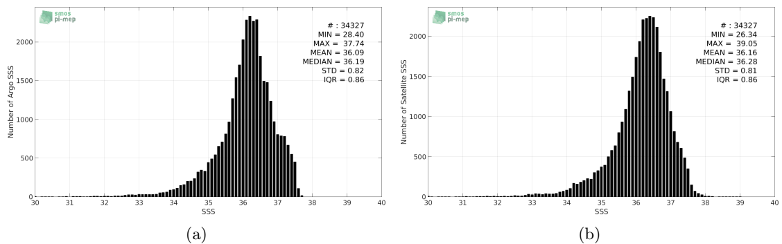
Figure 2: Histograms of SSS from Argo (a) and SMAP-L3-JPL-V4-8DAY-RUNNING-60KM (b) considering all match-up pairs per bins of 0.1 over the Tropical Atlantic Ocean Pi-MEP region and for the full satellite product period.
