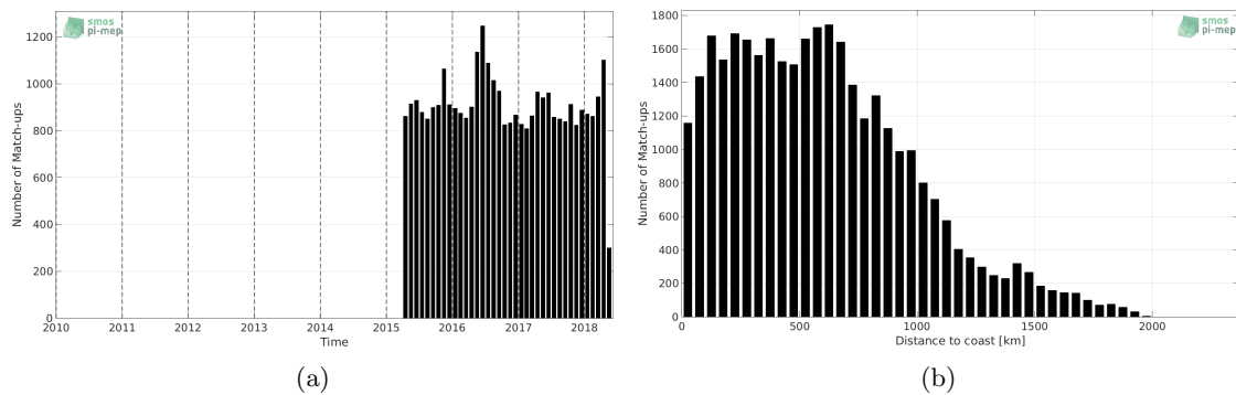
Figure 1: Number of match-ups between Argo and SMAP-L3-JPL-V4-8DAY-RUNNING-60KM SSS as a function of time (a) and as function of the distance to coast (b) over the Tropical Atlantic Ocean Pi-MEP region and for the full satellite product period.
