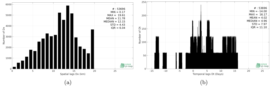
Figure 5: Histograms of the spatial (a) and temporal (b) lags between the time of the TSG-SAMOS measurements and the date of the corresponding SMAP-L3-JPL-V4-MONTHLY-60KM SSS product.
