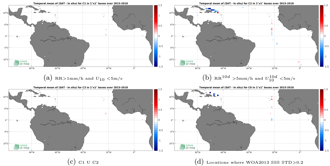
Figure 12: Temporal mean gridded over spatial boxes of size 1^\circ \times 1^\circ of \Delta\text{SSS} (SMAP-L3-JPL-V4-MONTHLY-60KM - TSG-SAMOS) for 4 different subdatasets corresponding to: RR > 1mm/h and U_{10} < 5\text{m/s} (a), RR^{10d} > 5\text{mm/h} and U_{10}^{10d} < 5\text{m/s} (b), C1 U C2 (c), Locations where WOA2013 SSS STD > 0.2 (d).
