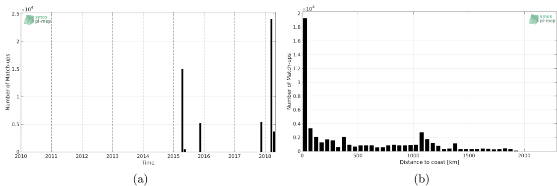
Figure 1: Number of match-ups between TSG-SAMOS and SMAP-L3-JPL-V4-MONTHLY-60KM SSS as a function of time (a) and as function of the distance to coast (b) over the Tropical Atlantic Ocean Pi-MEP region and for the full satellite product period.
