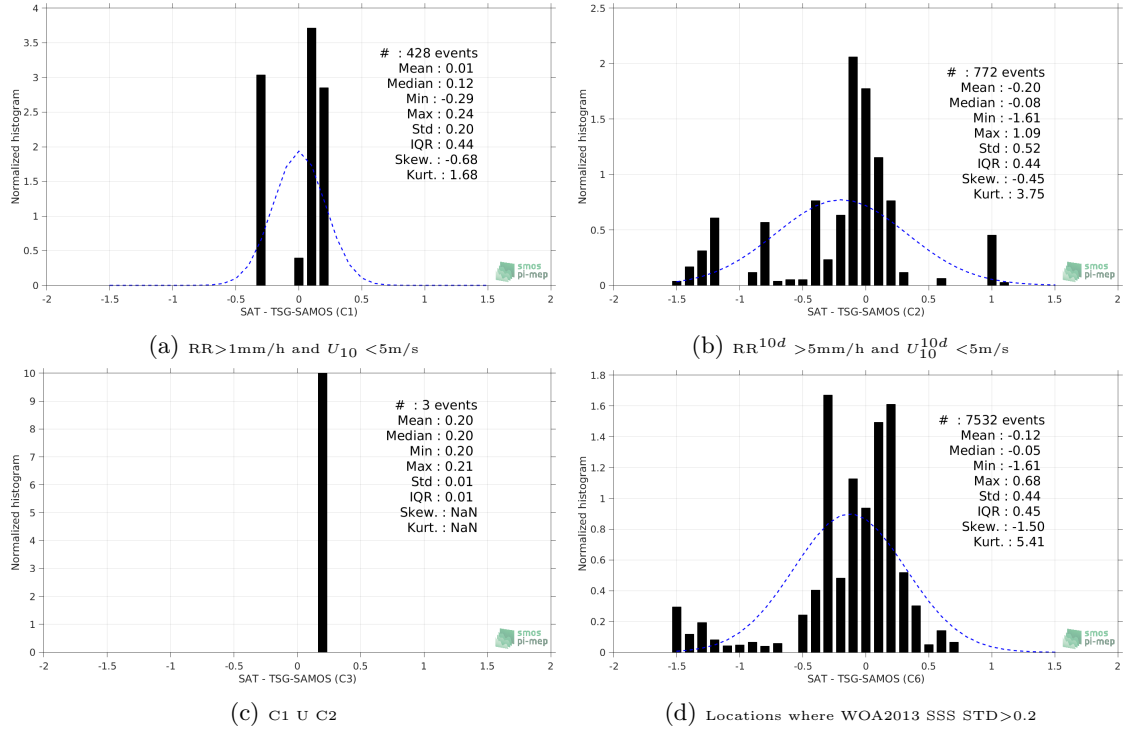
Figure 13: Normalized histogram of \Delta\text{SSS} (SMAP-L3-JPL-V4-MONTHLY-60KM - TSG-SAMOS) for 6 different subdatasets corresponding to: RR > 1\text{mm/h} and U_{10} < 5\text{m/s} (a), RR^{10d} > 5\text{mm/h} and U_{10}^{10d} < 5\text{m/s} (b), C1 U C2 (c), Locations where WOA2013 SSS STD > 0.2 (d).
