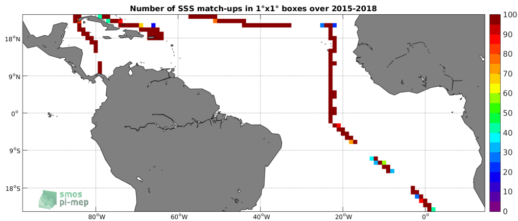
Figure 4: Number of SSS match-ups between TSG-SAMOS SSS and the SMAP-L3-JPL-V4-MONTHLY-60KM SSS product for the Tropical Atlantic Ocean Pi-MEP region over 1^\circ \times 1^\circ boxes and for the full satellite product period.
