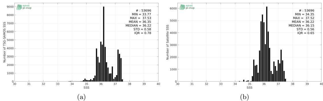
Figure 2: Histograms of SSS from TSG-SAMOS (a) and SMAP-L3-JPL-V4-MONTHLY-60KM (b) considering all match-up pairs per bins of 0.1 over the Tropical Atlantic Ocean Pi-MEP region and for the full satellite product period.
