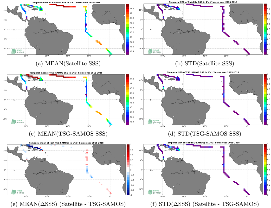
Figure 6: Temporal mean (left) and STD (right) of SSS from SMAP-L3-JPL-V4-MONTHLY-60KM (top), TSG-SAMOS (middle), and of \Delta SSS (Satellite - TSG-SAMOS). Only match-up pairs are used to generate these maps.
