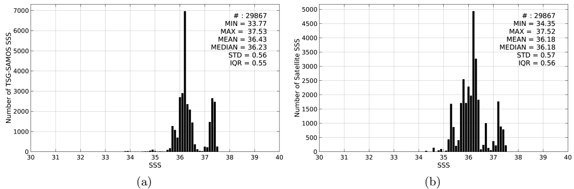
Figure 2: Histograms of SSS from TSG-SAMOS (a) and SMAP-L3-JPL-V4-MONTHLY-60KM (b) considering all match-up pairs per bins of 0.1 over the Tropical Atlantic Ocean Pi-MEP region and for the full satellite product period.
