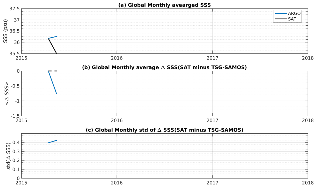
Figure 7: Time series of the monthly averaged mean SSS (top), mean \Delta SSS (Satellite - TSG-SAMOS) and STD of \Delta SSS (Satellite - TSG-SAMOS) over the Tropical Atlantic Ocean Pi-MEP region considering all match-ups collected by the Pi-MEP platform.
