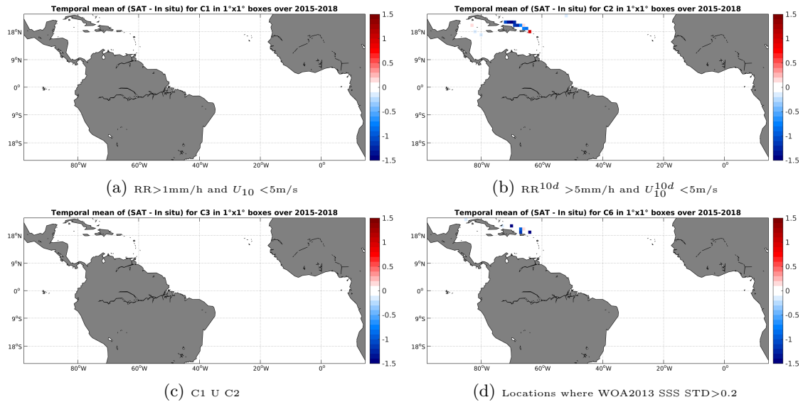
Figure 12: Temporal mean gridded over spatial boxes of size 1^\circ \times 1^\circ of \Delta SSS (SMAP-L3-JPL-V4-MONTHLY-60KM - TSG-SAMOS) for 4 different subdatasets corresponding to:RR>1mm/h and U_{10} < 5 m/s (a), RR^{10d} > 5 mm/h and U_{10}^{10d} < 5 m/s (b), C1 U C2 (c),Locations where WOA2013 SSS STD>0.2 (d).
