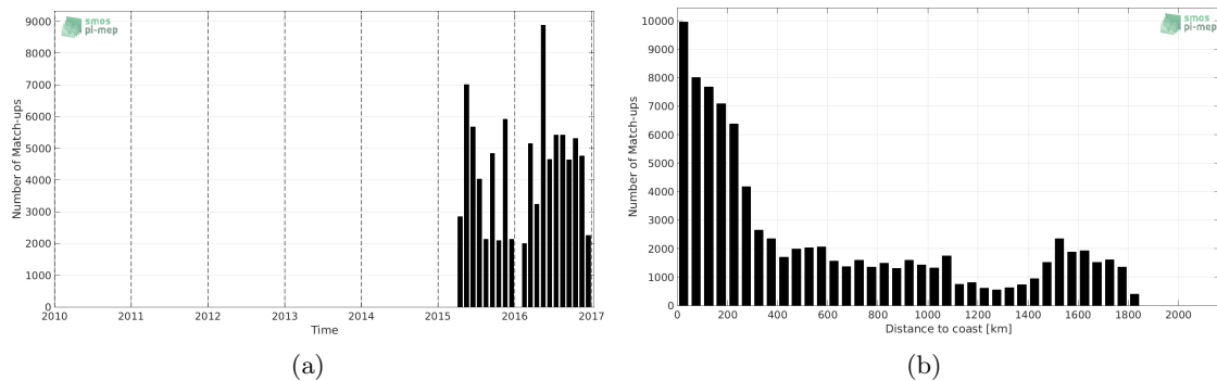
Figure 1: Number of match-ups between TSG-LEGOS-DM and SMAP-L3-JPL-V4-MONTHLY-60KM SSS as a function of time (a) and as function of the distance to coast (b) over the Tropical Atlantic Ocean Pi-MEP region and for the full satellite product period.
