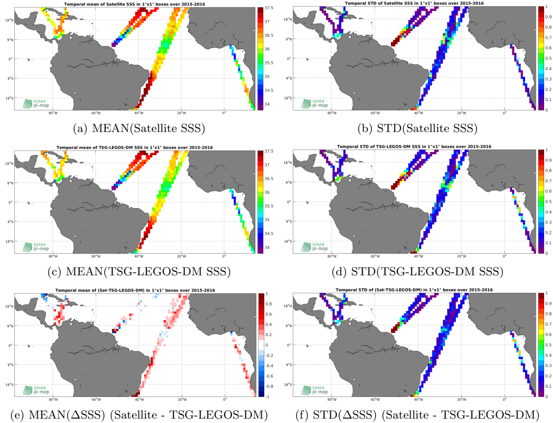
Figure 6: Temporal mean (left) and STD (right) of SSS from SMAP-L3-JPL-V4-MONTHLY-60KM (top), TSG-LEGOS-DM (middle), and of \Delta SSS (Satellite - TSG-LEGOS-DM). Only match-up pairs are used to generate these maps.
