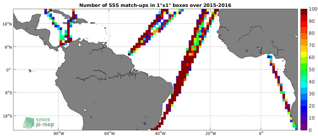
Figure 4: Number of SSS match-ups between TSG-LEGOS-DM SSS and the SMAP-L3-JPL-V4-MONTHLY-60KM SSS product for the Tropical Atlantic Ocean Pi-MEP region over 1^\circ \times 1^\circ boxes and for the full satellite product period.
