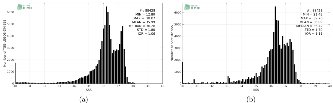
Figure 2: Histograms of SSS from TSG-LEGOS-DM (a) and SMAP-L3-JPL-V4-MONTHLY-60KM (b) considering all match-up pairs per bins of 0.1 over the Tropical Atlantic Ocean Pi-MEP region and for the full satellite product period.
