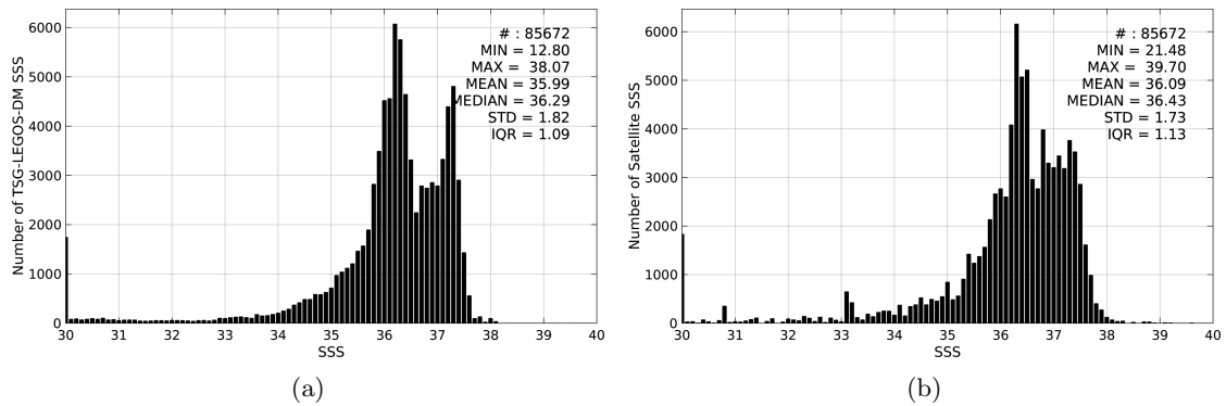
Figure 2: Histograms of SSS from TSG-LEGOS-DM (a) and SMAP-L3-JPL-V4-MONTHLY-60KM (b) considering all match-up pairs per bins of 0.1 over the Tropical Atlantic Ocean Pi-MEP region and for the full satellite product period.
