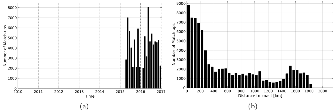
Figure 1: Number of match-ups between TSG-LEGOS-DM and SMAP-L3-JPL-V4-MONTHLY-60KM SSS as a function of time (a) and as function of the distance to coast (b) over the Tropical Atlantic Ocean Pi-MEP region and for the full satellite product period.
