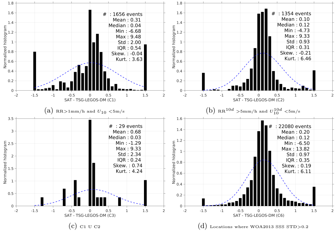
Figure 13: Normalized histogram of \Delta\text{SSS} (SMAP-L3-JPL-V4-MONTHLY-60KM - TSG-LEGOS-DM) for 6 different subdatasets corresponding to: RR > 1\text{mm/h} and U_{10} < 5\text{m/s} (a), RR^{10d} > 5\text{mm/h} and U_{10}^{10d} < 5\text{m/s} (b), C1 U C2 (c), Locations where WOA2013 SSS STD > 0.2 (d).
