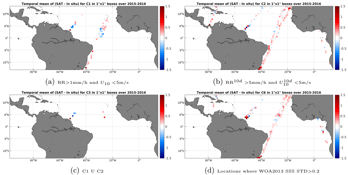
Figure 12: Temporal mean gridded over spatial boxes of size 1^\circ \times 1^\circ of \Delta SSS (SMAP-L3-JPL-V4-MONTHLY-60KM - TSG-LEGOS-DM) for 4 different subdatasets corresponding to:RR>1mm/h and U_{10} < 5 m/s (a), RR^{10d} > 5 mm/h and U_{10}^{10d} < 5 m/s (b), C1 U C2 (c),Locations where WOA2013 SSS STD>0.2 (d).
