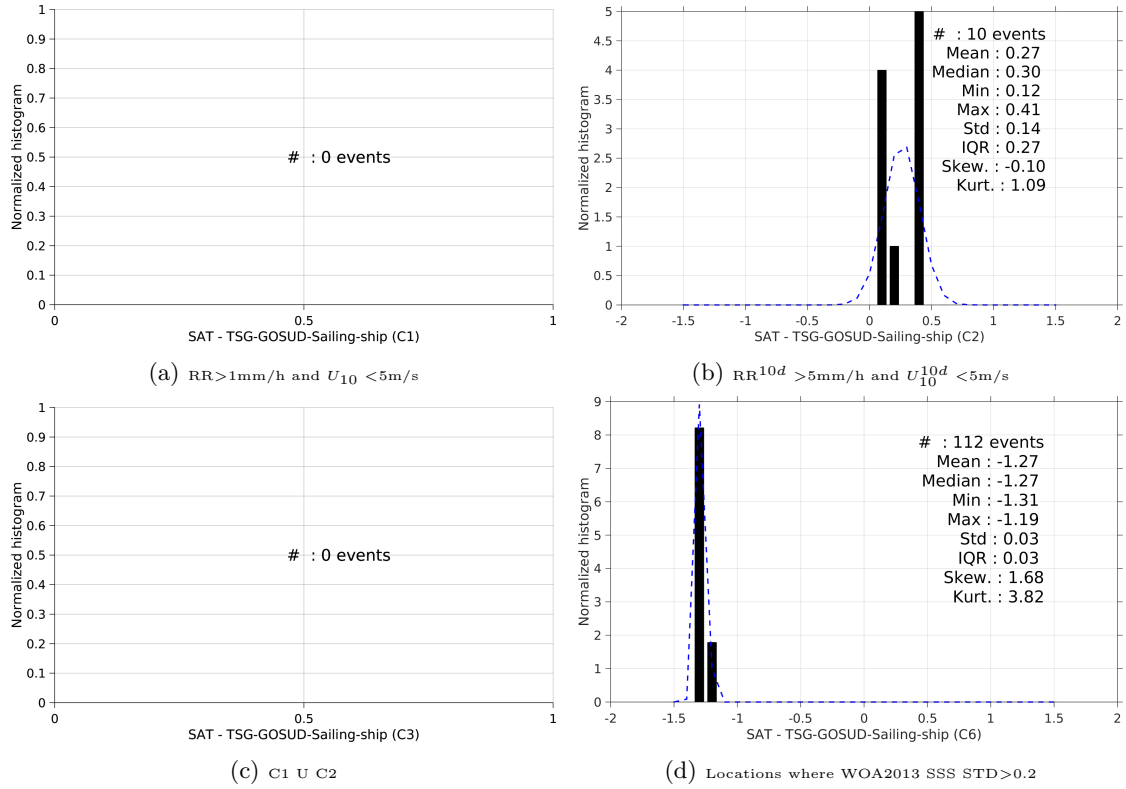
Figure 13: Normalized histogram of \Delta\text{SSS} (SMAP-L3-JPL-V4-MONTHLY-60KM - TSG-GOSUD-Sailing-ship) for 6 different subdatasets corresponding to: RR > 1\text{mm/h} and U_{10} < 5\text{m/s} (a), RR^{10d} > 5\text{mm/h} and U_{10}^{10d} < 5\text{m/s} (b), C1 U C2 (c), Locations where WOA2013 SSS STD > 0.2 (d).
