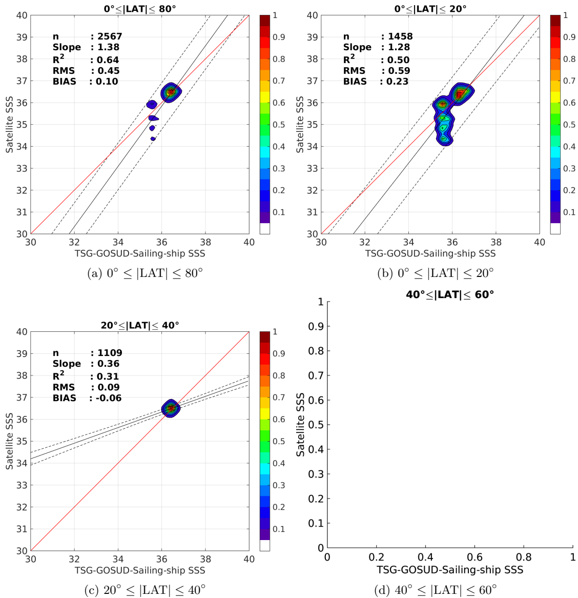
Figure 9: Contour maps of the concentration of SMAP-L3-JPL-V4-MONTHLY-60KM SSS (y-axis) versus TSG-GOSUD-Sailing-ship SSS (x-axis) at match-up pairs for different latitude bands. For each plot, the red line shows x=y . The black thin and dashed lines indicate a linear fit through the data cloud and the \pm 95\% confidence levels, respectively. The number match-up pairs n , the slope and R^2 coefficient of the linear fit, the root mean square (RMS) and the mean bias between satellite and in situ data are indicated for each latitude band in each plots.
