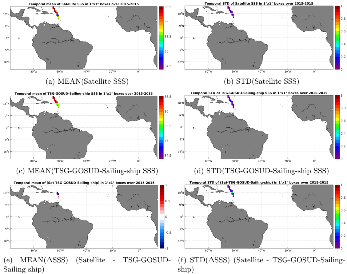
Figure 6: Temporal mean (left) and STD (right) of SSS from SMAP-L3-JPL-V4-MONTHLY-60KM (top), TSG-GOSUD-Sailing-ship (middle), and of \Delta SSS (Satellite - TSG-GOSUD-Sailing-ship). Only match-up pairs are used to generate these maps.
