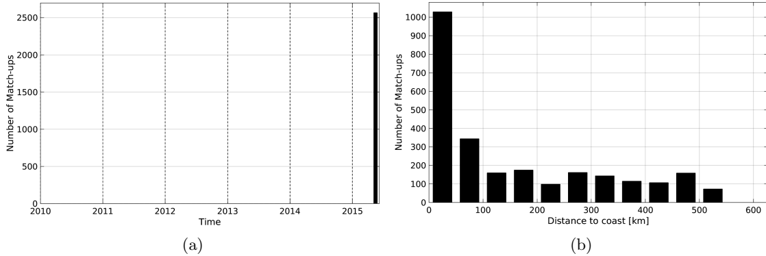
Figure 1: Number of match-ups between TSG-GOSUD-Sailing-ship and SMAP-L3-JPL-V4-MONTHLY-60KM SSS as a function of time (a) and as function of the distance to coast (b) over the Tropical Atlantic Ocean Pi-MEP region and for the full satellite product period.
