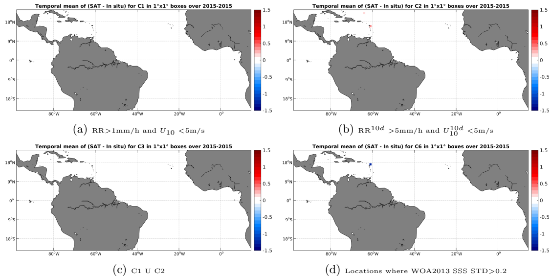
Figure 12: Temporal mean gridded over spatial boxes of size 1^\circ \times 1^\circ of \Delta SSS (SMAP-L3-JPL-V4-MONTHLY-60KM - TSG-GOSUD-Sailing-ship) for 4 different subdatasets corresponding to: RR > 1\text{mm/h} and U_{10} < 5\text{m/s} (a), RR^{10d} > 5\text{mm/h} and U_{10}^{10d} < 5\text{m/s} (b), C1 U C2 (c), Locations where WOA2013 SSS STD > 0.2 (d).
