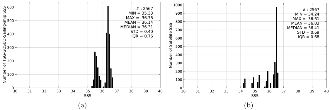
Figure 2: Histograms of SSS from TSG-GOSUD-Sailing-ship (a) and SMAP-L3-JPL-V4-MONTHLY-60KM (b) considering all match-up pairs per bins of 0.1 over the Tropical Atlantic Ocean Pi-MEP region and for the full satellite product period.
