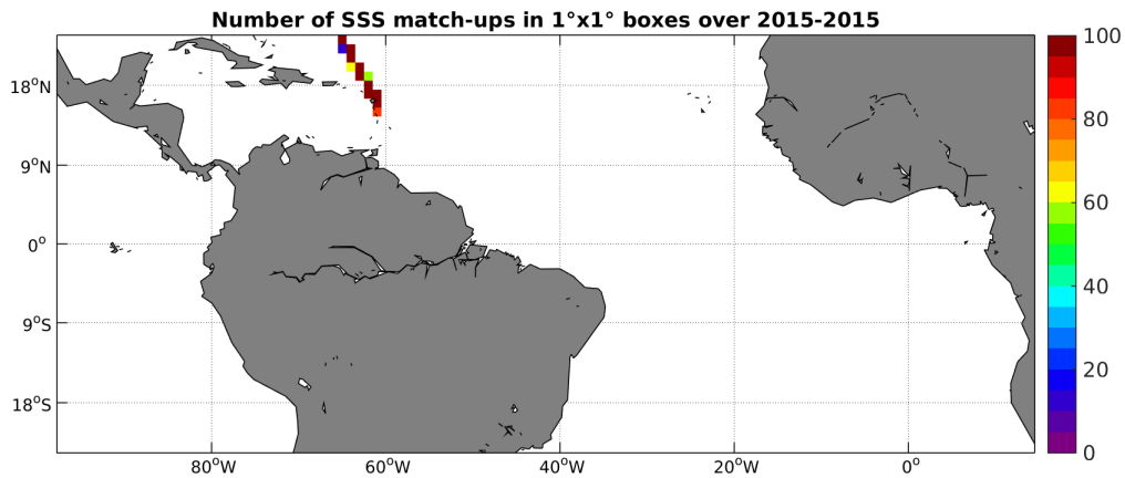
Figure 4: Number of SSS match-ups between TSG-GOSUD-Sailing-ship SSS and the SMAP-L3-JPL-V4-MONTHLY-60KM SSS product for the Tropical Atlantic Ocean Pi-MEP region over 1^{\circ} \times 1^{\circ} boxes and for the full satellite product period.
