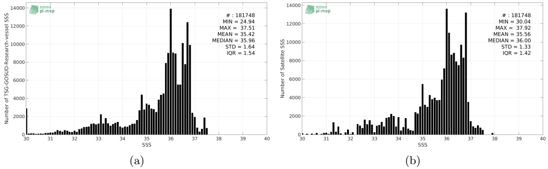
Figure 2: Histograms of SSS from TSG-GOSUD-Research-vessel (a) and SMAP-L3-JPL-V4-MONTHLY-60KM (b) considering all match-up pairs per bins of 0.1 over the Tropical Atlantic Ocean Pi-MEP region and for the full satellite product period.
