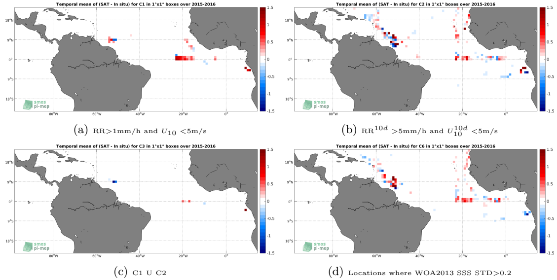
Figure 12: Temporal mean gridded over spatial boxes of size 1^\circ \times 1^\circ of \Delta SSS (SMAP-L3-JPL-V4-MONTHLY-60KM - TSG-GOSUD-Research-vessel) for 4 different subdatasets corresponding to: RR > 1\text{mm/h} and U_{10} < 5\text{m/s} (a), RR^{10d} > 5\text{mm/h} and U_{10}^{10d} < 5\text{m/s} (b), C1 U C2 (c), Locations where WOA2013 SSS STD > 0.2 (d).
