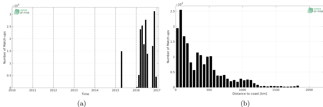
Figure 1: Number of match-ups between TSG-GOSUD-Research-vessel and SMAP-L3-JPL-V4-MONTHLY-60KM SSS as a function of time (a) and as function of the distance to coast (b) over the Tropical Atlantic Ocean Pi-MEP region and for the full satellite product period.
