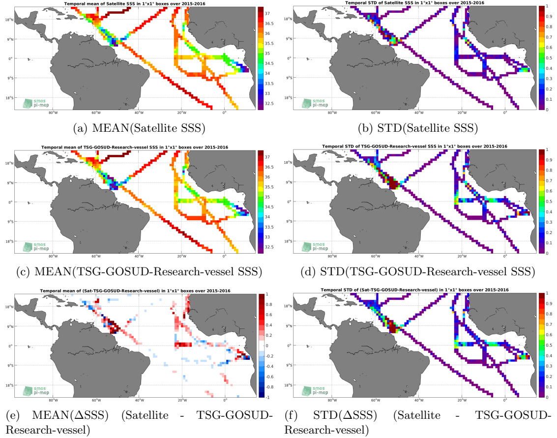
Figure 6: Temporal mean (left) and STD (right) of SSS from SMAP-L3-JPL-V4-MONTHLY-60KM (top), TSG-GOSUD-Research-vessel (middle), and of \Delta SSS (Satellite - TSG-GOSUD-Research-vessel). Only match-up pairs are used to generate these maps.
