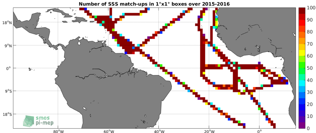
Figure 4: Number of SSS match-ups between TSG-GOSUD-Research-vessel SSS and the SMAP-L3-JPL-V4-MONTHLY-60KM SSS product for the Tropical Atlantic Ocean Pi-MEP region over 1^\circ \times 1^\circ boxes and for the full satellite product period.
