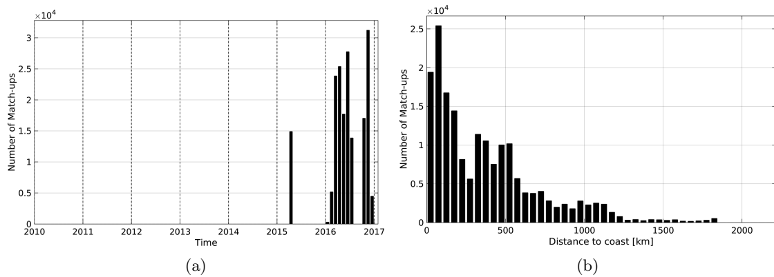
Figure 1: Number of match-ups between TSG-GOSUD-Research-vessel and SMAP-L3-JPL-V4-MONTHLY-60KM SSS as a function of time (a) and as function of the distance to coast (b) over the Tropical Atlantic Ocean Pi-MEP region and for the full satellite product period.
