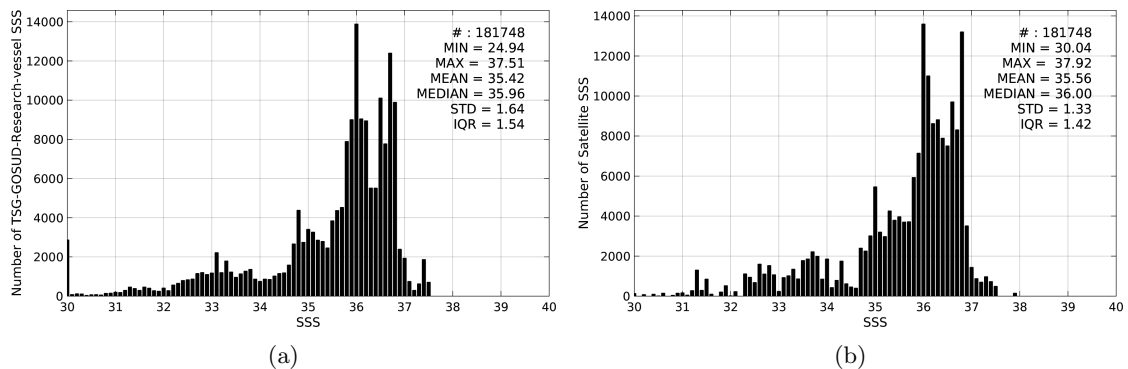
Figure 2: Histograms of SSS from TSG-GOSUD-Research-vessel (a) and SMAP-L3-JPL-V4-MONTHLY-60KM (b) considering all match-up pairs per bins of 0.1 over the Tropical Atlantic Ocean Pi-MEP region and for the full satellite product period.
