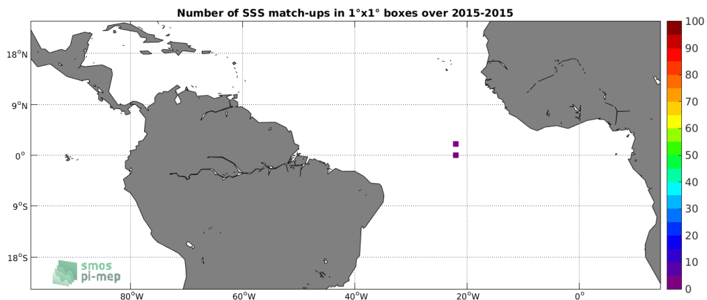
Figure 3: Number of SSS match-ups between Surface drifters SSS and the SMAP-L3-JPL-V4-MONTHLY-60KM SSS product for the Tropical Atlantic Ocean Pi-MEP region over 1°x1° boxes and for the full satellite product period.
