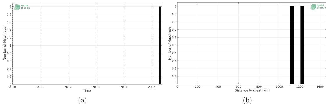
Figure 1: Number of match-ups between Surface drifters and SMAP-L3-JPL-V4-MONTHLY-60KM SSS as a function of time (a) and as function of the distance to coast (b) over the Tropical Atlantic Ocean Pi-MEP region and for the full satellite product period.
