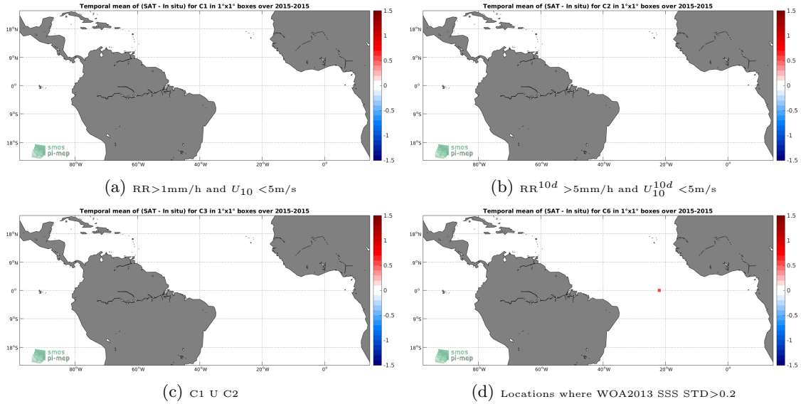
Figure 11: Temporal mean gridded over spatial boxes of size 1^\circ \times 1^\circ of \Delta SSS (SMAP-L3-JPL-V4-MONTHLY-60KM - Surface drifters) for 4 different subdatasets corresponding to: RR > 1\text{mm/h} and U_{10} < 5\text{m/s} (a), RR^{10d} > 5\text{mm/h} and U_{10}^{10d} < 5\text{m/s} (b), C1 U C2 (c), Locations where WOA2013 SSS STD > 0.2 (d).
