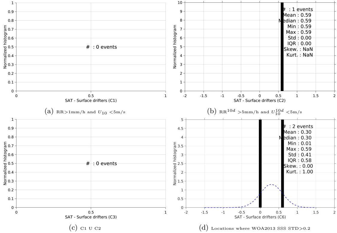
Figure 12: Normalized histogram of \Delta\text{SSS} (SMAP-L3-JPL-V4-MONTHLY-60KM - Surface drifters) for 6 different subdatasets corresponding to: RR > 1\text{mm/h} and U_{10} < 5\text{m/s} (a), RR^{10d} > 5\text{mm/h} and U_{10}^{10d} < 5\text{m/s} (b), C1 U C2 (c), Locations where WOA2013 SSS STD > 0.2 (d).
