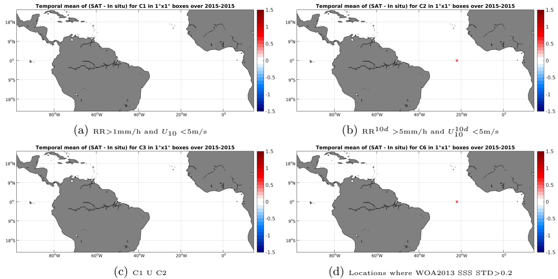
Figure 11: Temporal mean gridded over spatial boxes of size 1^\circ \times 1^\circ of \Delta SSS (SMAP-L3-JPL-V4-MONTHLY-60KM - Surface drifters) for 4 different subdatasets corresponding to: RR > 1mm/h and U_{10} < 5m/s (a), RR^{10d} > 5mm/h and U_{10}^{10d} < 5m/s (b), C1 U C2 (c), Locations where WOA2013 SSS STD > 0.2 (d).
