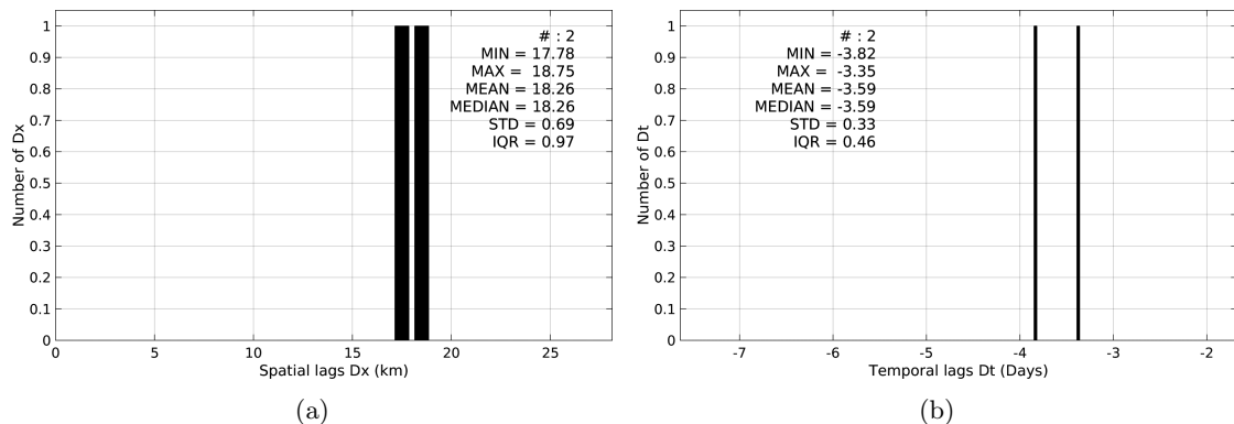
Figure 4: Histograms of the spatial (a) and temporal (b) lags between the time of the Surface drifters measurements and the date of the corresponding SMAP-L3-JPL-V4-MONTHLY-60KM SSS product.
