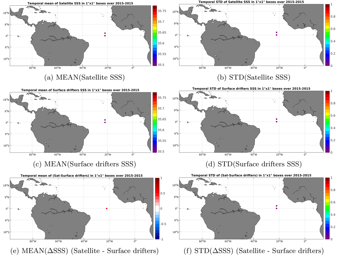
Figure 5: Temporal mean (left) and STD (right) of SSS from SMAP-L3-JPL-V4-MONTHLY-60KM (top), Surface drifters (middle), and of \Delta SSS (Satellite - Surface drifters). Only match-up pairs are used to generate these maps.
