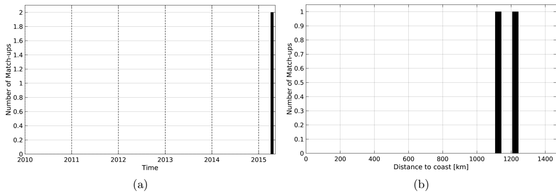
Figure 1: Number of match-ups between Surface drifters and SMAP-L3-JPL-V4-MONTHLY-60KM SSS as a function of time (a) and as function of the distance to coast (b) over the Tropical Atlantic Ocean Pi-MEP region and for the full satellite product period.
