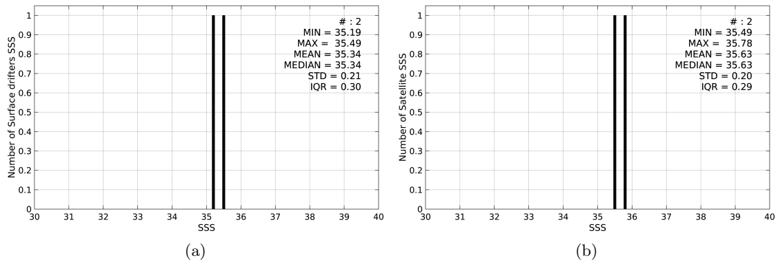
Figure 2: Histograms of SSS from Surface drifters (a) and SMAP-L3-JPL-V4-MONTHLY-60KM (b) considering all match-up pairs per bins of 0.1 over the Tropical Atlantic Ocean Pi-MEP region and for the full satellite product period.
