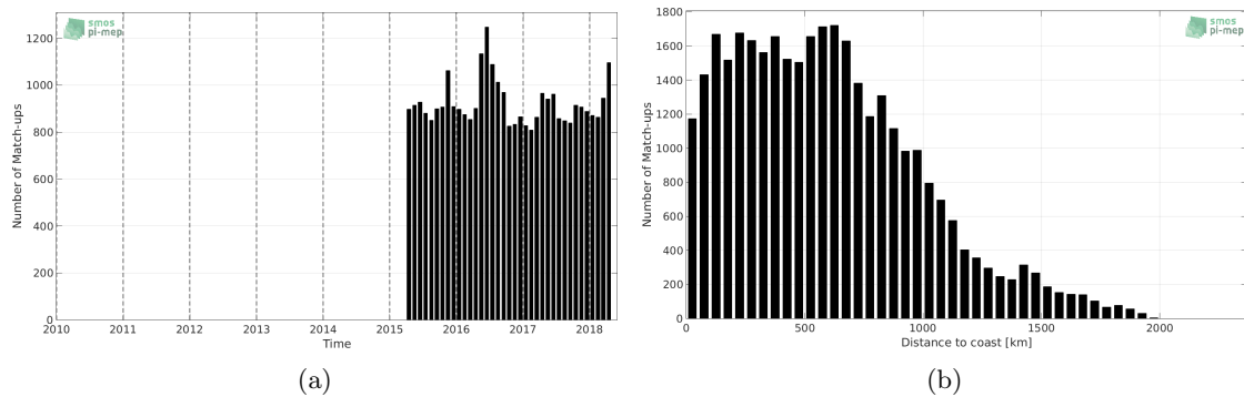
Figure 1: Number of match-ups between Argo and SMAP-L3-JPL-V4-MONTHLY-60KM SSS as a function of time (a) and as function of the distance to coast (b) over the Tropical Atlantic Ocean Pi-MEP region and for the full satellite product period.
