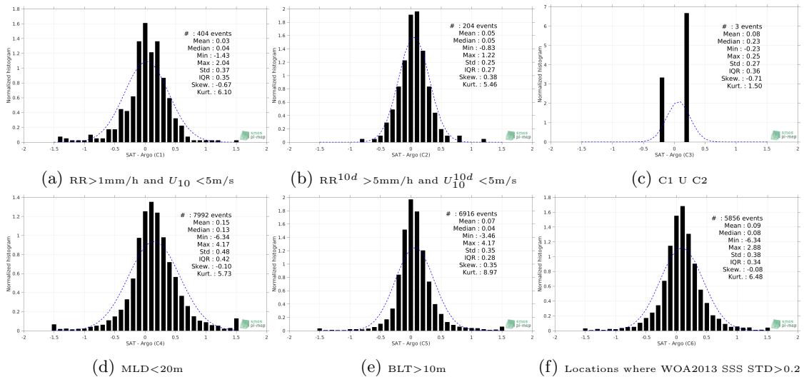
Figure 13: Normalized histogram of \Delta SSS (SMAP-L3-JPL-V4-MONTHLY-60KM - Argo) for 6 different subdatasets corresponding to: RR>1mm/h and U_{10} < 5\text{m/s} (a), RR^{10d} > 5\text{mm/h} and U_{10}^{10d} < 5\text{m/s} (b), C1 U C2 (c), MLD<20m (d), BLT>10m (e), Locations where WOA2013 SSS STD>0.2 (f).
