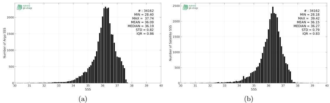
Figure 2: Histograms of SSS from Argo (a) and SMAP-L3-JPL-V4-MONTHLY-60KM (b) considering all match-up pairs per bins of 0.1 over the Tropical Atlantic Ocean Pi-MEP region and for the full satellite product period.
