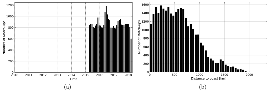
Figure 1: Number of match-ups between Argo and SMAP-L3-JPL-V4-MONTHLY-60KM SSS as a function of time (a) and as function of the distance to coast (b) over the Tropical Atlantic Ocean Pi-MEP region and for the full satellite product period.
