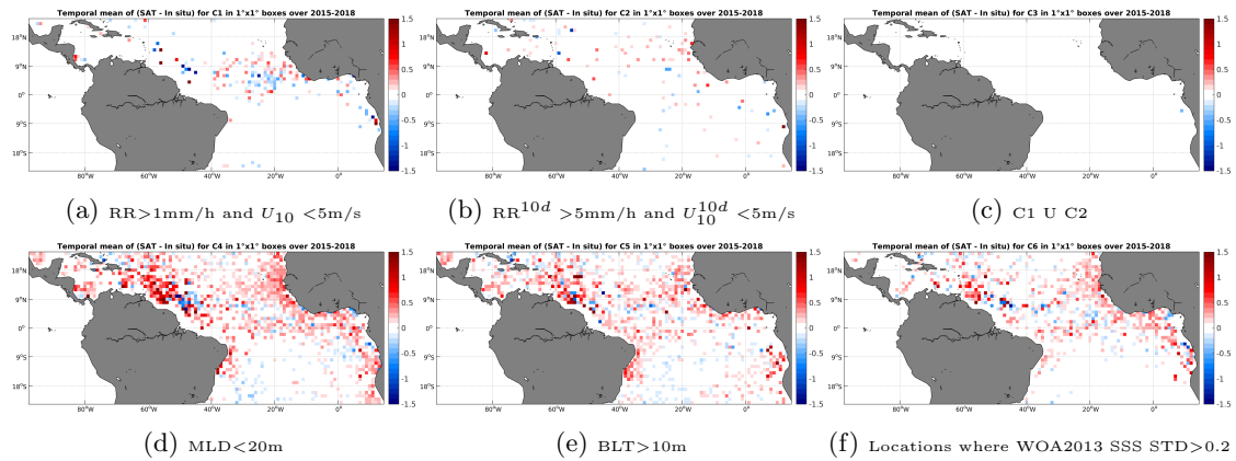
Figure 12: Temporal mean gridded over spatial boxes of size 1^\circ \times 1^\circ of \Delta SSS (SMAP-L3-JPL-V4-MONTHLY-60KM - Argo) for 6 different subdatasets corresponding to:RR >1 mm/h and U_{10} < 5 m/s (a), RR ^{10d} > 5 mm/h and U_{10}^{10d} < 5 m/s (b), C1 U C2 (c),MLD <20 m (d),BLT >10 m (e),Locations where WOA2013 SSS STD >0.2 (f).
