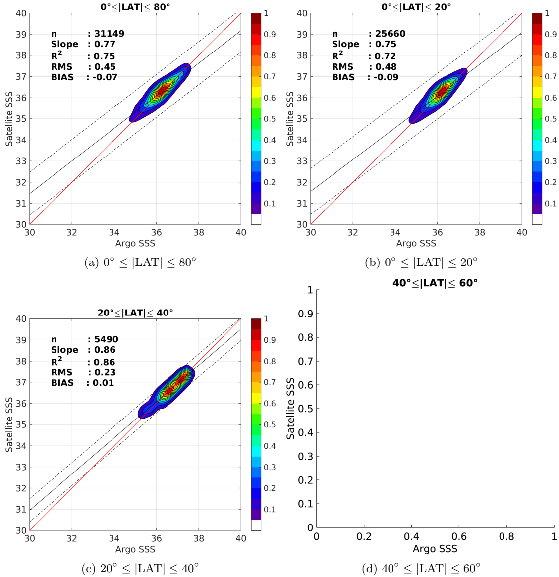
Figure 9: Contour maps of the concentration of SMAP-L3-JPL-V4-MONTHLY-60KM SSS (y-axis) versus Argo SSS (x-axis) at match-up pairs for different latitude bands. For each plot, the red line shows x=y . The black thin and dashed lines indicate a linear fit through the data cloud and the \pm 95\% confidence levels, respectively. The number match-up pairs n , the slope and R^2 coefficient of the linear fit, the root mean square (RMS) and the mean bias between satellite and in situ data are indicated for each latitude band in each plots.
