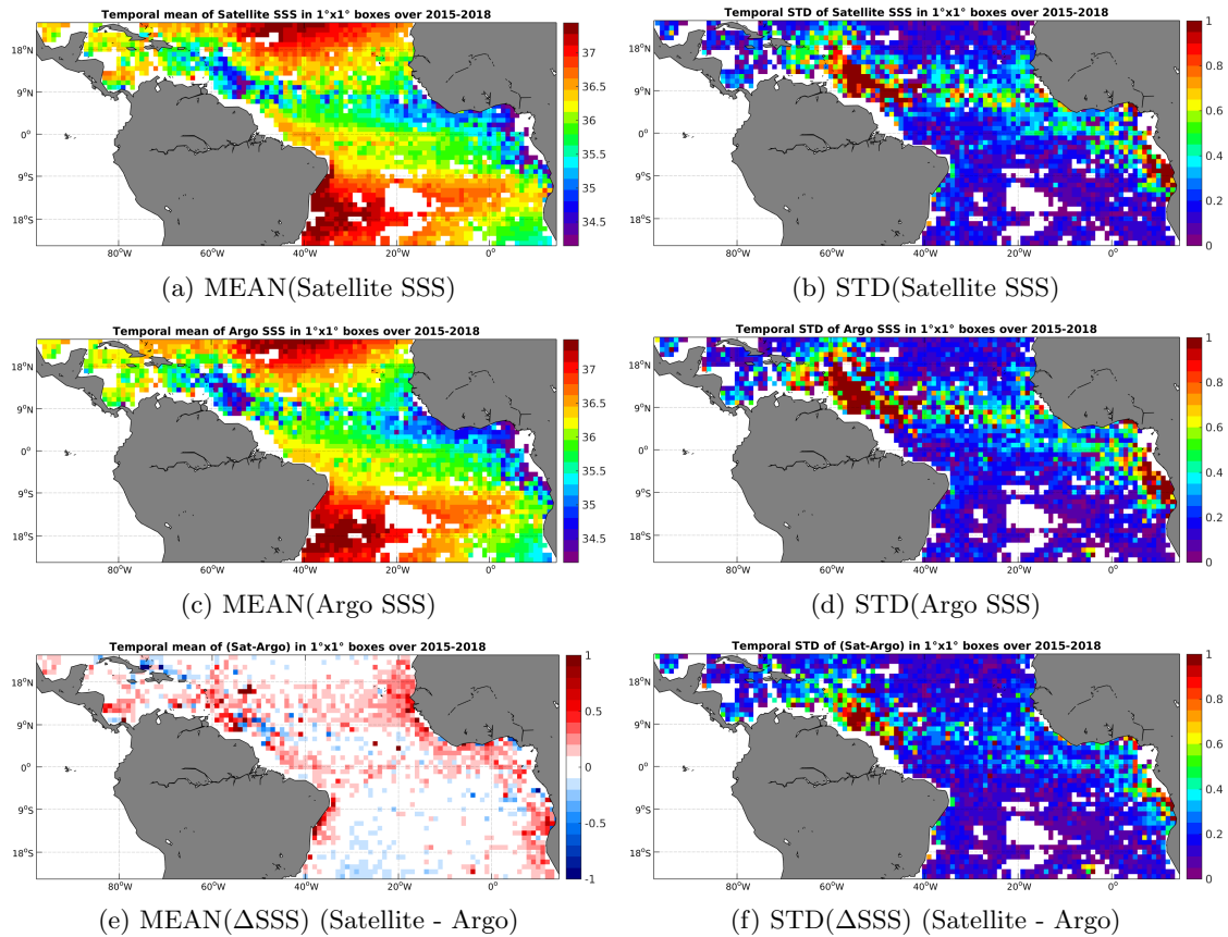
Figure 6: Temporal mean (left) and STD (right) of SSS from SMAP-L3-JPL-V4-MONTHLY-60KM (top), Argo (middle), and of \Delta SSS (Satellite - Argo). Only match-up pairs are used to generate these maps.
