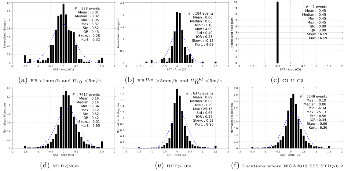
Figure 13: Normalized histogram of \Delta SSS (SMAP-L3-JPL-V4-MONTHLY-60KM - Argo) for 6 different subdatasets corresponding to: RR>1mm/h and U_{10} < 5\text{m/s} (a), RR^{10d} > 5\text{mm/h} and U_{10}^{10d} < 5\text{m/s} (b), C1 U C2 (c), MLD<20m (d), BLT>10m (e), Locations where WOA2013 SSS STD>0.2 (f).
