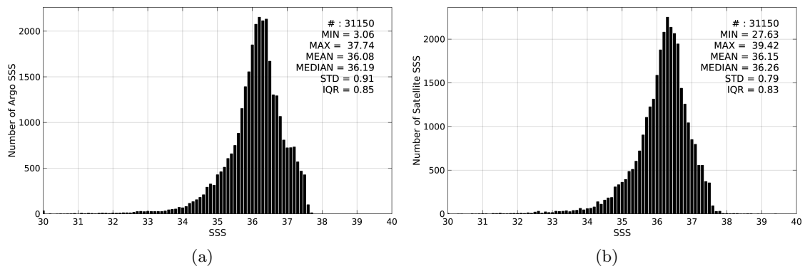
Figure 2: Histograms of SSS from Argo (a) and SMAP-L3-JPL-V4-MONTHLY-60KM (b) considering all match-up pairs per bins of 0.1 over the Tropical Atlantic Ocean Pi-MEP region and for the full satellite product period.
