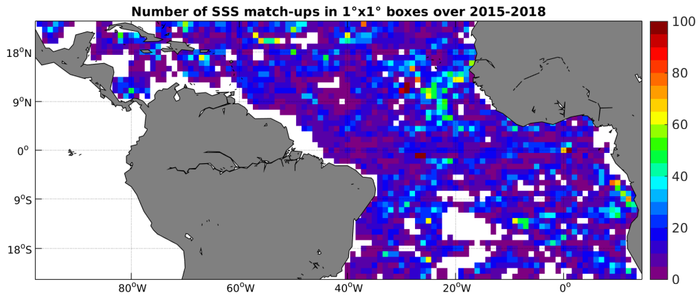
Figure 4: Number of SSS match-ups between Argo SSS and the SMAP-L3-JPL-V4-MONTHLY-60KM SSS product for the Tropical Atlantic Ocean Pi-MEP region over 1^\circ \times 1^\circ boxes and for the full satellite product period.
