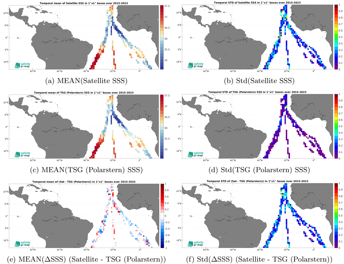
Figure 7: Temporal mean (left) and Std (right) of SSS from SMAP SSS L2 v6 (RSS) (top), TSG (Polarstern) (middle), and of \Delta SSS (Satellite - TSG (Polarstern)). Only match-up pairs are used to generate these maps.
