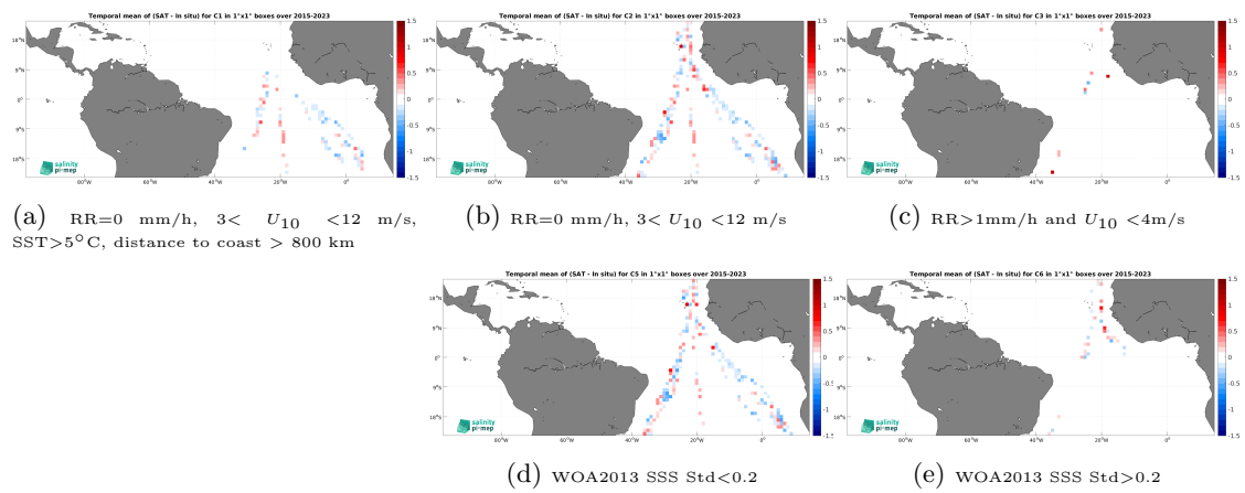
Figure 14: Temporal mean gridded over spatial boxes of size 1^\circ \times 1^\circ of \Delta\text{SSS} (SMAP SSS L2 v6 (RSS) - TSG (Polarstern)) for 5 different subdatasets corresponding to:RR=0 mm/h, 3 < U_{10} < 12 m/s, SST >5^\circ\text{C} , distance to coast > 800 km (a), RR=0 mm/h, 3 < U_{10} < 12 m/s (b), RR >1 mm/h and U_{10} < 4 m/s (c), WOA2013 SSS Std <0.2 (d), WOA2013 SSS Std >0.2 (e).
