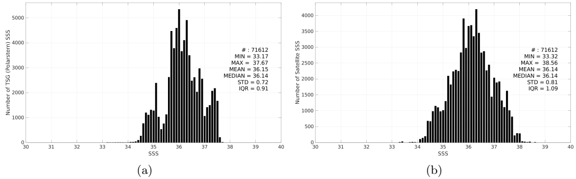
Figure 3: Histograms of SSS from TSG (Polarstern) (a) and SMAP SSS L2 v6 (RSS) (b) considering all match-up pairs per bins of 0.1 over the Tropical Atlantic Ocean Pi-MEP region and for the full satellite product period.
