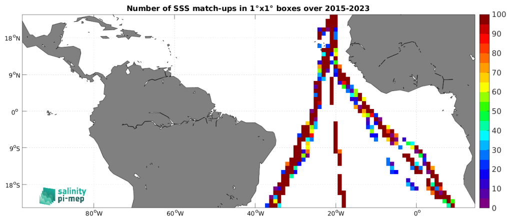
Figure 5: Number of SSS match-ups between TSG (Polarstern) SSS and the SMAP SSS L2 v6 (RSS) SSS product for the Tropical Atlantic Ocean Pi-MEP region over 1^\circ \times 1^\circ boxes and for the full satellite product period.
