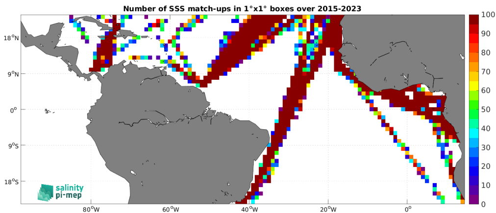
Figure 5: Number of SSS match-ups between TSG (LEGOS-DM) SSS and the SMAP SSS L2 v6 (RSS) SSS product for the Tropical Atlantic Ocean Pi-MEP region over 1°×1° boxes and for the full satellite product period.
