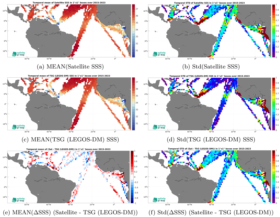
Figure 7: Temporal mean (left) and Std (right) of SSS from SMAP SSS L2 v6 (RSS) (top), TSG (LEGOS-DM) (middle), and of \Delta SSS (Satellite - TSG (LEGOS-DM)). Only match-up pairs are used to generate these maps.
