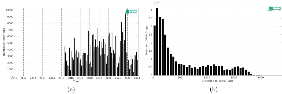
Figure 2: Number of match-ups between TSG (LEGOS-DM) and SMAP SSS L2 v6 (RSS) SSS as a function of time (a) and as function of the distance to coast (b) over the Tropical Atlantic Ocean Pi-MEP region and for the full satellite product period.
