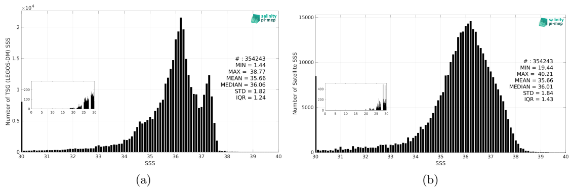
Figure 3: Histograms of SSS from TSG (LEGOS-DM) (a) and SMAP SSS L2 v6 (RSS) (b) considering all match-up pairs per bins of 0.1 over the Tropical Atlantic Ocean Pi-MEP region and for the full satellite product period.
