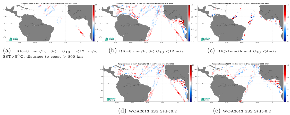
Figure 14: Temporal mean gridded over spatial boxes of size 1^\circ \times 1^\circ of \Delta\text{SSS} (SMAP SSS L2 v6 (RSS) - TSG (LEGOS-DM)) for 5 different subdatasets corresponding to:RR=0 mm/h, 3 < U_{10} < 12 m/s, SST >5^\circ\text{C} , distance to coast > 800 km (a), RR=0 mm/h, 3 < U_{10} < 12 m/s (b), RR >1 mm/h and U_{10} < 4 m/s (c), WOA2013 SSS Std <0.2 (d), WOA2013 SSS Std >0.2 (e).
