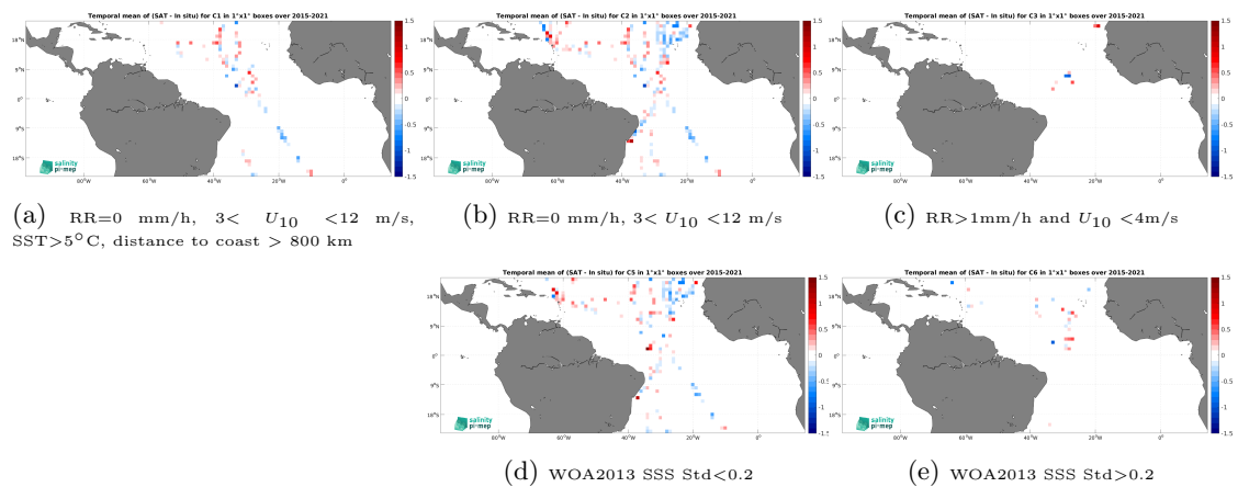
Figure 14: Temporal mean gridded over spatial boxes of size 1^\circ \times 1^\circ of \Delta\text{SSS} (SMAP SSS L2 v6 (RSS) - TSG (GOSUD-Sailing-ship)) for 5 different subdatasets corresponding to:RR=0 mm/h, 3 < U_{10} < 12 m/s, SST >5^\circ\text{C} , distance to coast > 800 km (a), RR=0 mm/h, 3 < U_{10} < 12 m/s (b), RR >1 mm/h and U_{10} < 4 m/s (c), WOA2013 SSS Std <0.2 (d), WOA2013 SSS Std >0.2 (e).
