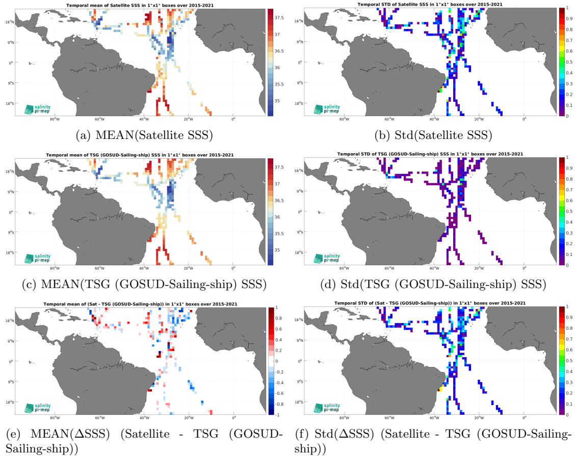
Figure 7: Temporal mean (left) and Std (right) of SSS from SMAP SSS L2 v6 (RSS) (top), TSG (GOSUD-Sailing-ship) (middle), and of \Delta SSS (Satellite - TSG (GOSUD-Sailing-ship)). Only match-up pairs are used to generate these maps.
