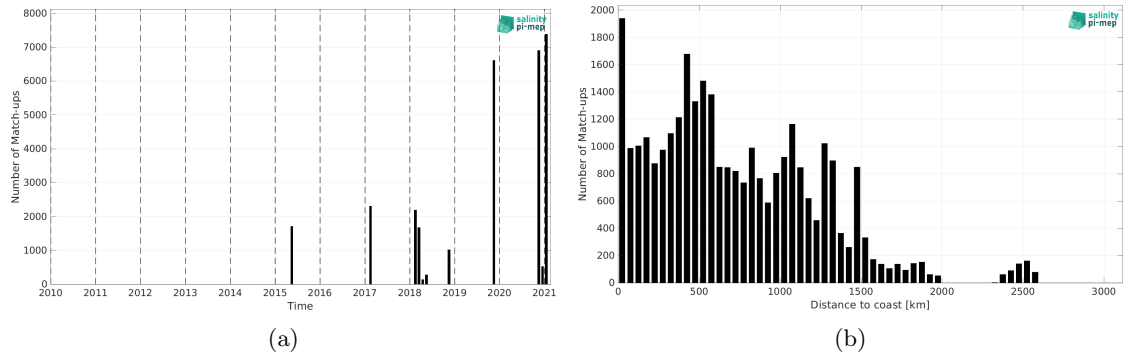
Figure 2: Number of match-ups between TSG (GOSUD-Sailing-ship) and SMAP SSS L2 v6 (RSS) SSS as a function of time (a) and as function of the distance to coast (b) over the Tropical Atlantic Ocean Pi-MEP region and for the full satellite product period.
