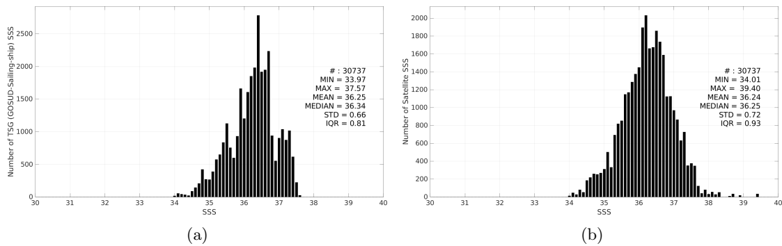
Figure 3: Histograms of SSS from TSG (GOSUD-Sailing-ship) (a) and SMAP SSS L2 v6 (RSS) (b) considering all match-up pairs per bins of 0.1 over the Tropical Atlantic Ocean Pi-MEP region and for the full satellite product period.
