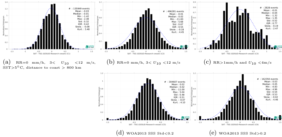
Figure 15: Normalized histogram of \Delta SSS (SMAP SSS L2 v6 (RSS) - TSG (GOSUD-Research-vessel)) for 5 different subdatasets corresponding to: RR=0 mm/h, 3 < U_{10} < 12 m/s, SST > 5^\circ\text{C} , distance to coast > 800 km (a), RR=0 mm/h, 3 < U_{10} < 12 m/s (b), RR > 1 mm/h and U_{10} < 4 m/s (c), WOA2013 SSS Std < 0.2 (d), WOA2013 SSS Std > 0.2 (e).
