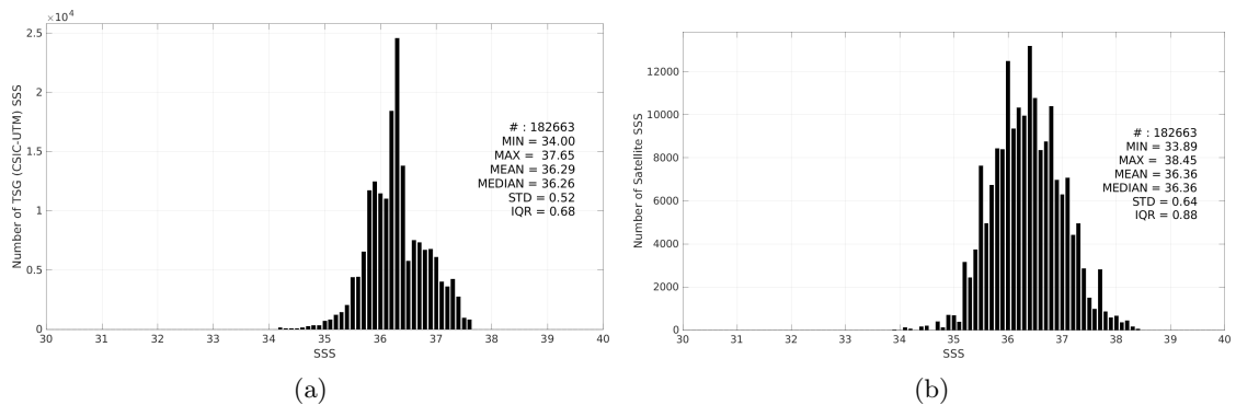
Figure 3: Histograms of SSS from TSG (CSIC-UTM) (a) and SMAP SSS L2 v6 (RSS) (b) considering all match-up pairs per bins of 0.1 over the Tropical Atlantic Ocean Pi-MEP region and for the full satellite product period.
