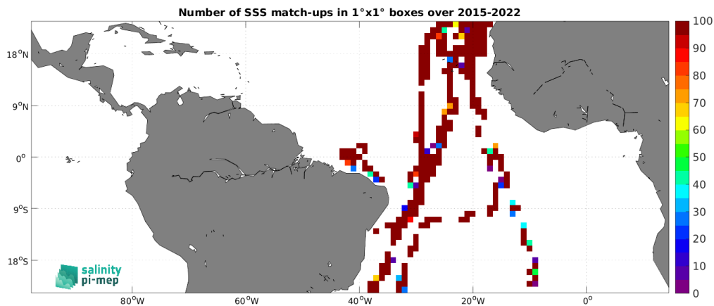
Figure 5: Number of SSS match-ups between TSG (CSIC-UTM) SSS and the SMAP SSS L2 v6 (RSS) SSS product for the Tropical Atlantic Ocean Pi-MEP region over 1^\circ \times 1^\circ boxes and for the full satellite product period.
