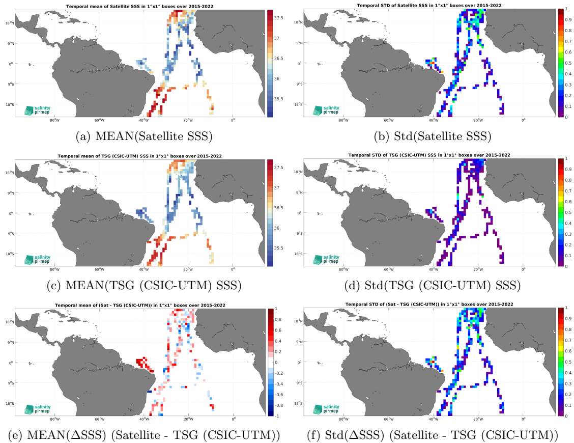
Figure 7: Temporal mean (left) and Std (right) of SSS from SMAP SSS L2 v6 (RSS) (top), TSG (CSIC-UTM) (middle), and of \Delta SSS (Satellite - TSG (CSIC-UTM)). Only match-up pairs are used to generate these maps.
