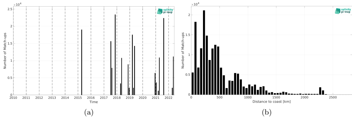
Figure 2: Number of match-ups between TSG (CSIC-UTM) and SMAP SSS L2 v6 (RSS) SSS as a function of time (a) and as function of the distance to coast (b) over the Tropical Atlantic Ocean Pi-MEP region and for the full satellite product period.
