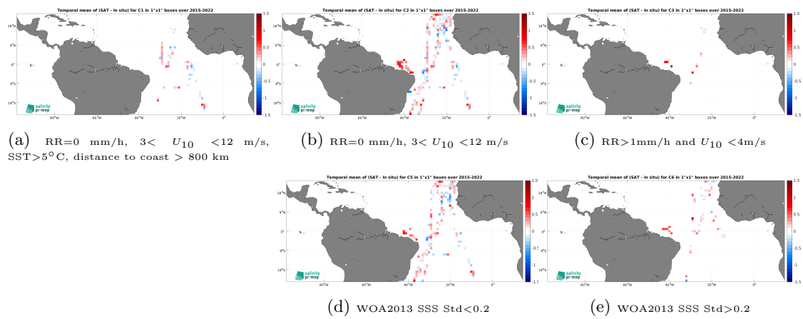
Figure 14: Temporal mean gridded over spatial boxes of size 1^\circ \times 1^\circ of \Delta SSS (SMAP SSS L2 v6 (RSS) - TSG (CSIC-UTM)) for 5 different subdatasets corresponding to:RR=0 mm/h, 3 < U_{10} < 12 m/s, SST >5^\circ\text{C} , distance to coast > 800 km (a), RR=0 mm/h, 3 < U_{10} < 12 m/s (b), RR >1 mm/h and U_{10} < 4 m/s (c), WOA2013 SSS Std <0.2 (d), WOA2013 SSS Std >0.2 (e).
